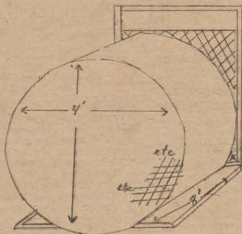
Culvert Trap
