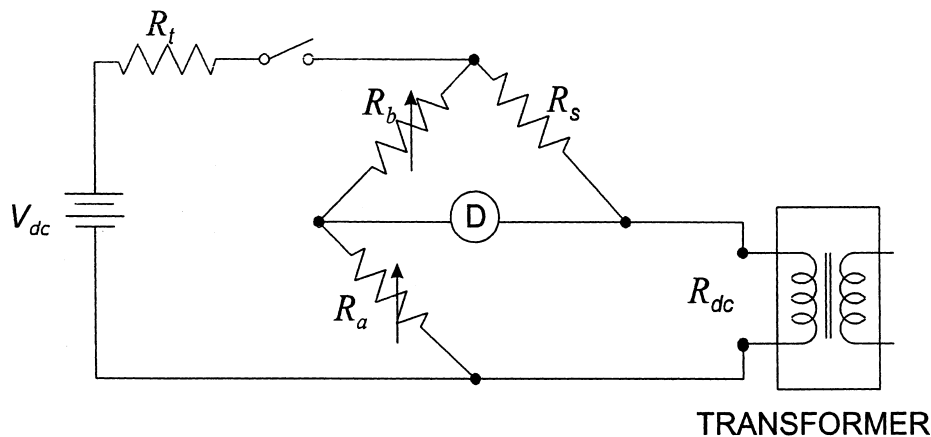
Figure 3.1 Wheatstone Bridge
