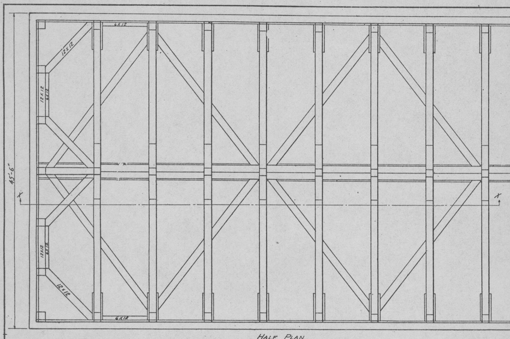
HALF PLAN
