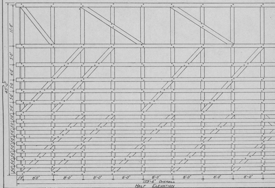
TYPICAL COFFERDAM CRIB FOR INTERMEDIATE PIER
