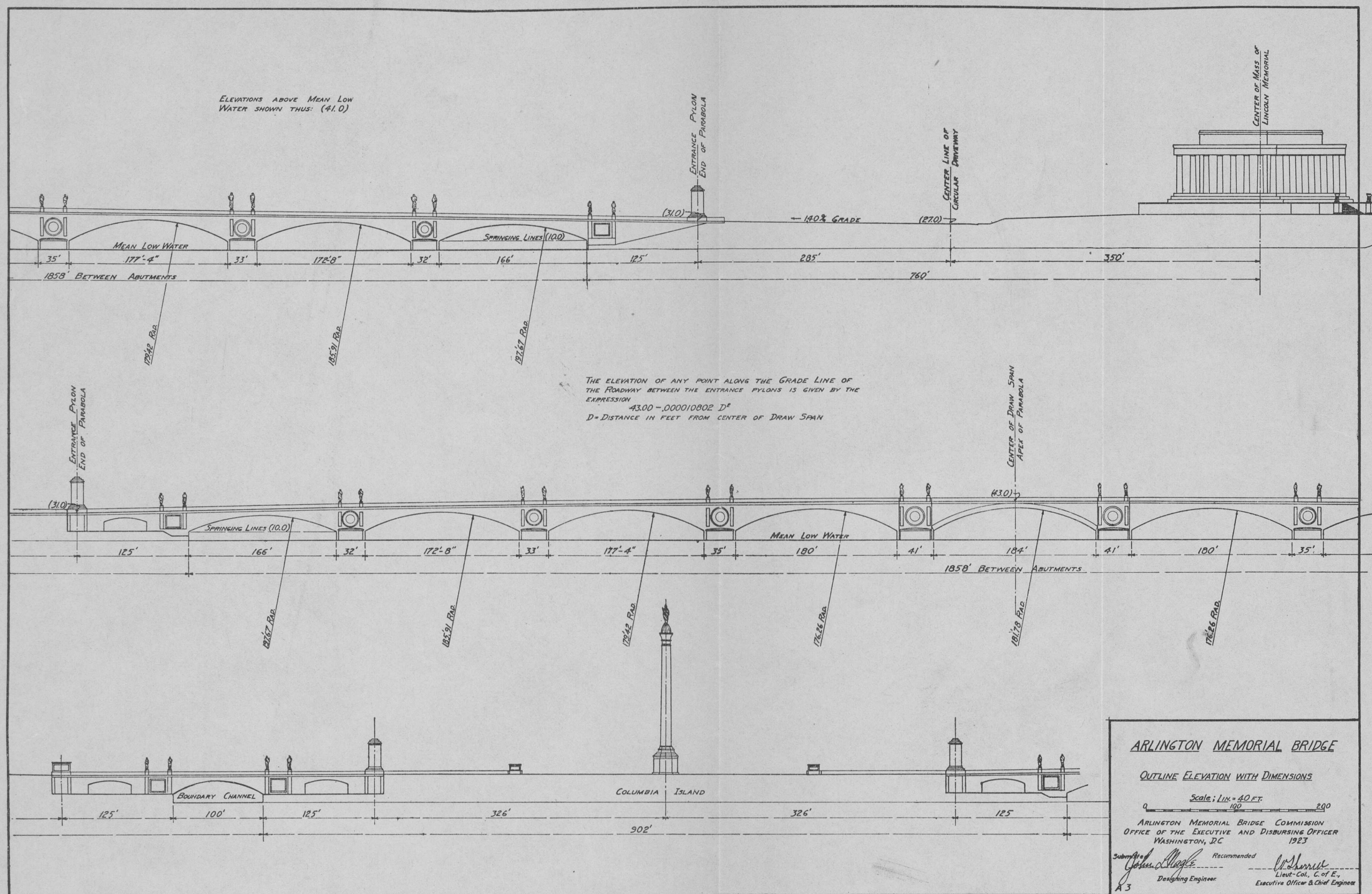
OUTLINE ELEVATION WITH DIMENSIONS
