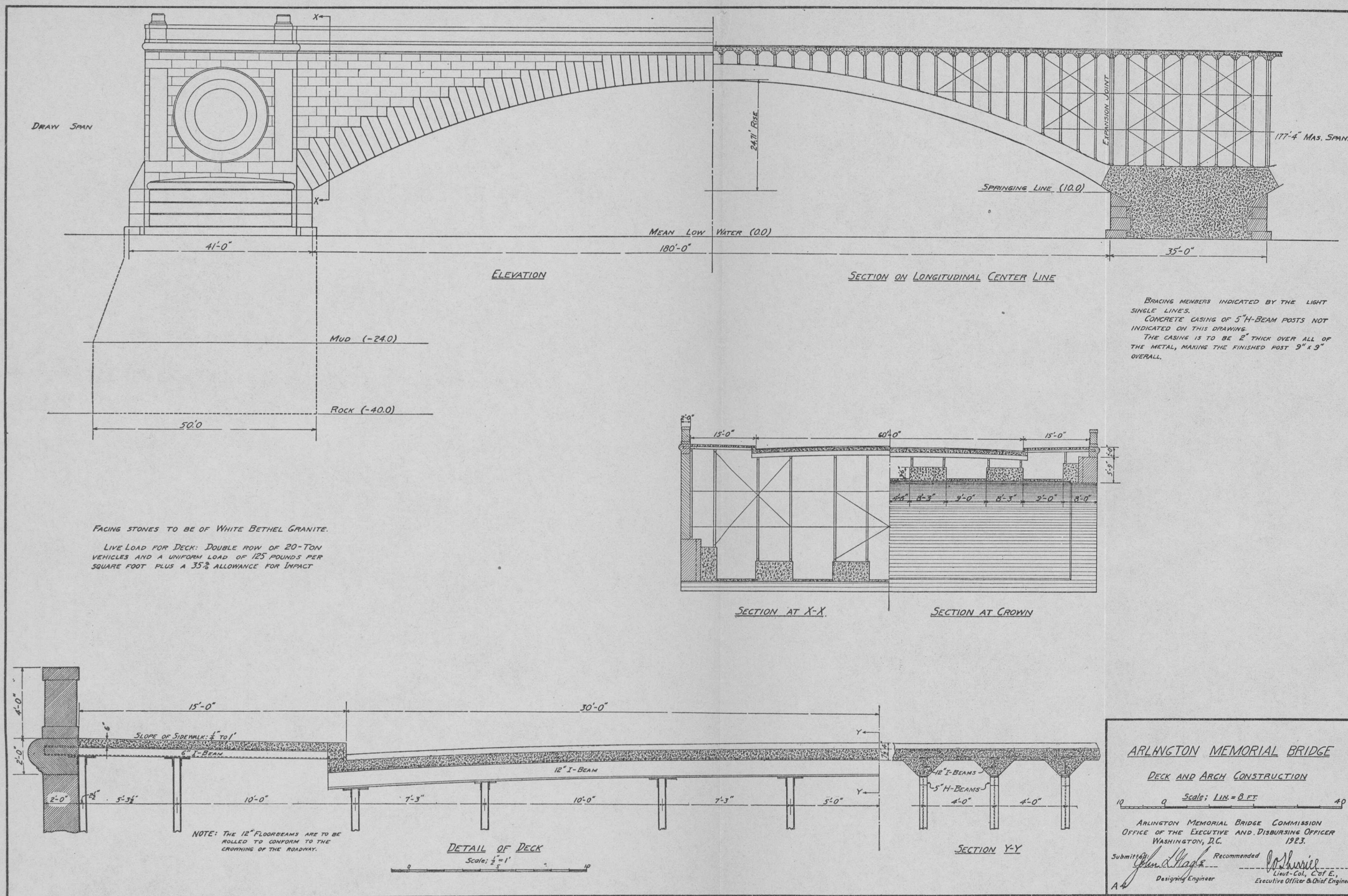
DETAIL OF ARCH RING
