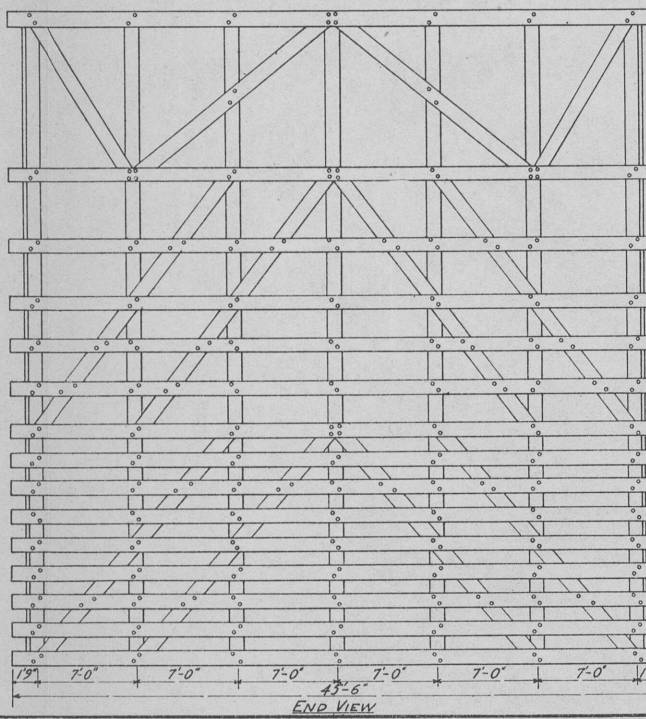
TYPICAL COFFERDAM CRIB FOR INTERMEDIATE PIER
