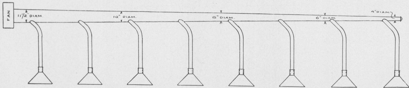
PLATE NO. 4.—MECHANICAL DRAWING SHOWING HOW TO CONSTRUCT AN EXHAUST HOOD FOR LINOTYPE MACHINES.
