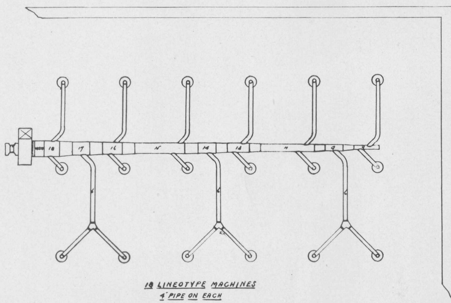
PLATE NO. 2.—MECHANICAL DRAWING SHOWING DETAILS OF CONSTRUCTION OF EXHAUST SYSTEM FOR LINOTYPE MACHINES.
