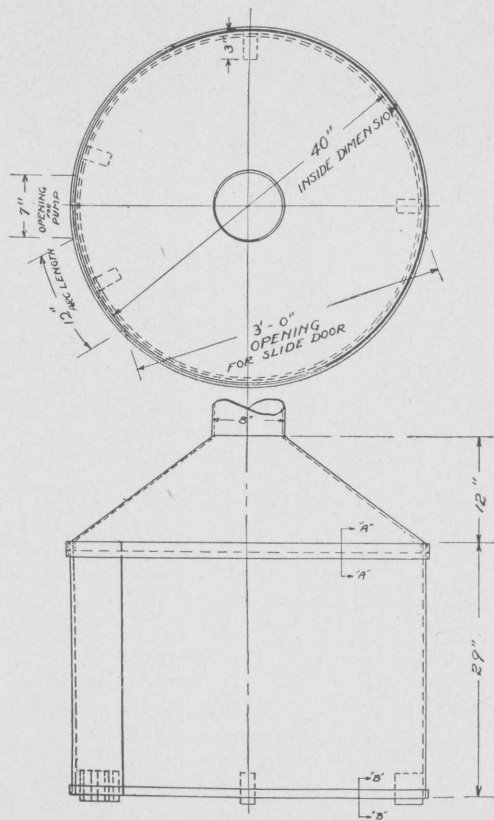
PLATE NO. 9.—MECHANICAL DRAWING SHOWING DETAILS OF CONSTRUCTION FOR HOOD FOR STEREOTYPE MACHINE.
