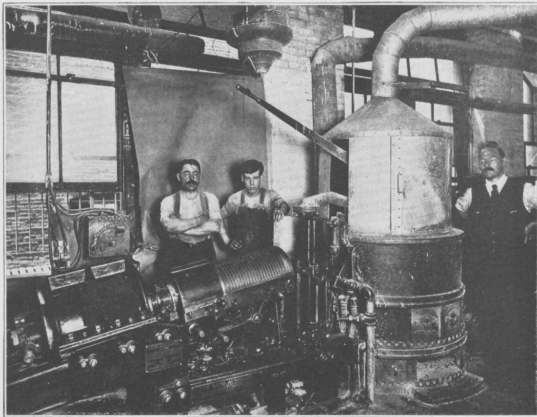
PLATE NO. 8.—EXHAUST HOOD ON MELTING KETTLE IN STEREOTYPE ROOM, SHOWING SLOT FOR PUMP ACTION.
