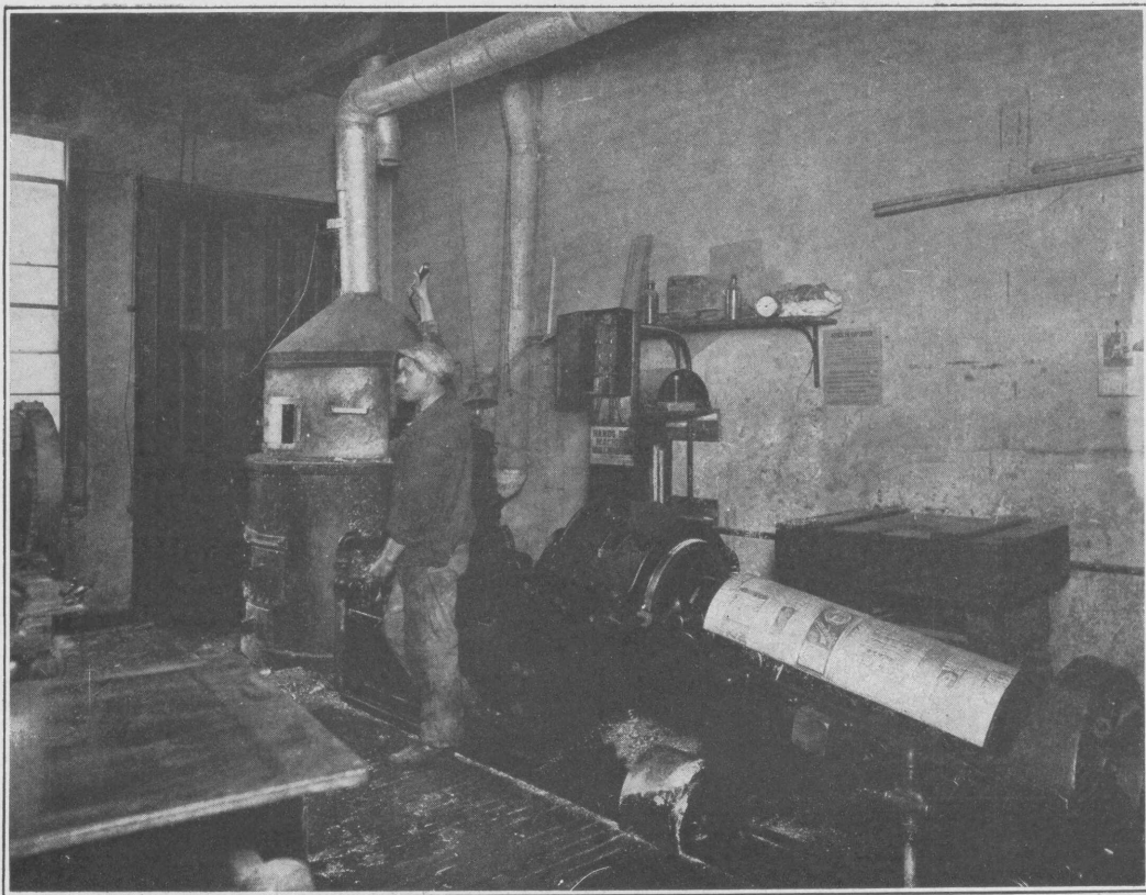
PLATE NO. 7.—MELTING KETTLES IN STEREOTYPE ROOM COMPLETELY INCLOSED WITH EXHAUST HOOD. ACCESS TO KETTLE GAINED BY MEANS OF A SLIDING DOOR.
