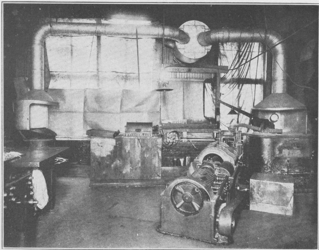
PLATE NO. 6.—OPEN TYPE OF EXHAUST HOODS FOR MELTING KETTLES IN STEREOTYPE ROOM.
