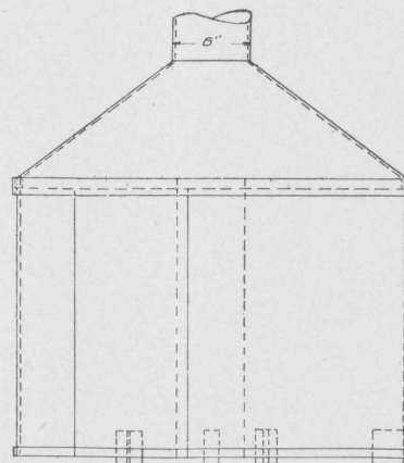
PLATE NO. 9.—MECHANICAL DRAWING SHOWING DETAILS OF CONSTRUCTION FOR HOOD FOR STEREOTYPE MACHINE.
