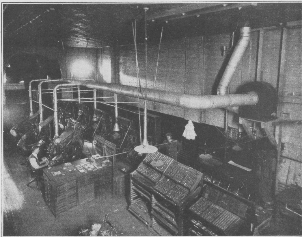
PLATE NO. 5.—SHOWING INSTALLATION OF EXHAUST SYSTEM FOR LINOTYPE MACHINES.
