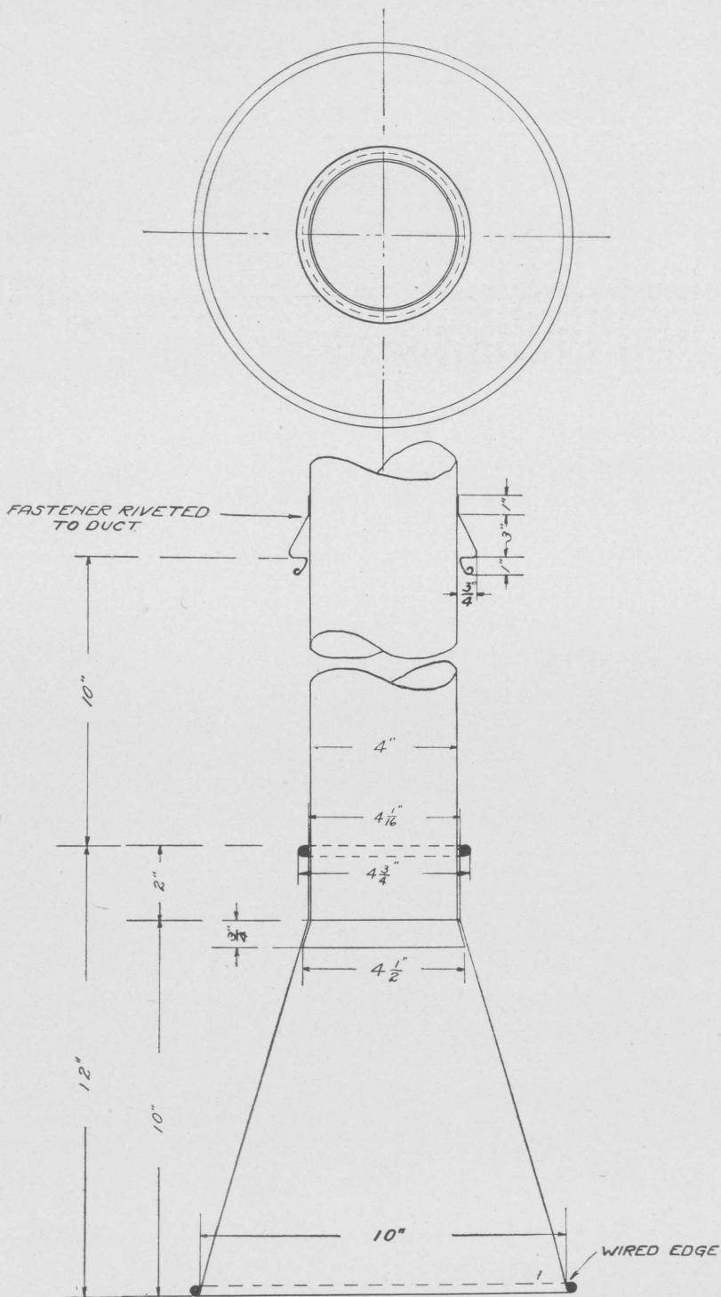
PLATE NO. 3.—MECHANICAL DRAWING SHOWING DETAILS OF CONSTRUCTION OF EXHAUST HOOD FOR LINOTYPE MACHINES.
