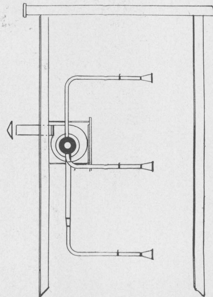
PLATE NO. 2.—MECHANICAL DRAWING SHOWING DETAILS OF CONSTRUCTION OF EXHAUST SYSTEM FOR LINOTYPE MACHINES.
