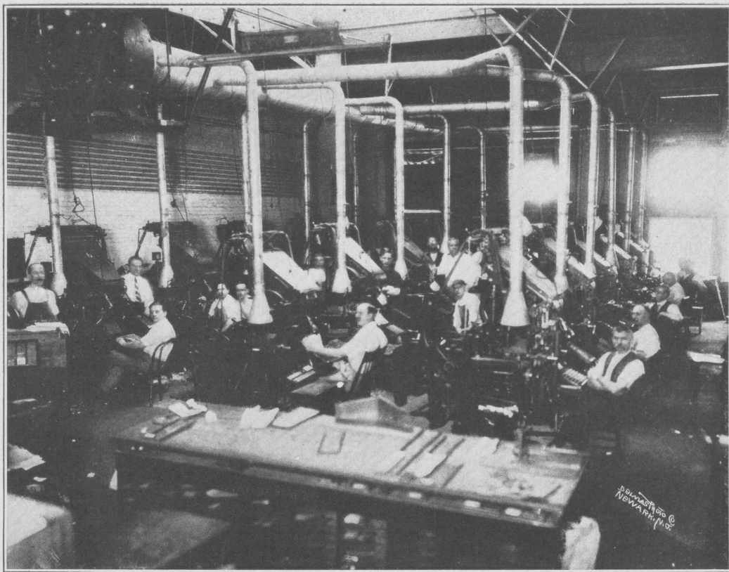
PLATE NO. 1.—MECHANICAL EXHAUST SYSTEM FOR THE REMOVAL OF NOXIOUS FUMES FROM LINOTYPE MACHINES.
