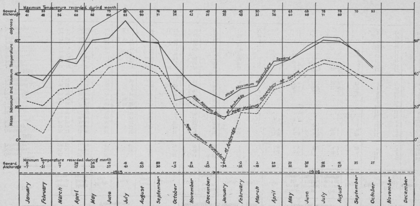
Comparative temperature chart—Anchorage and Seward, Alaska, 1915-16.
