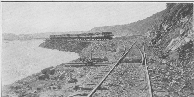
B. MATANUSKA DISTRICT. View showing shear dams constructed along the Matanuska branch line to protect the embankment from the swift current of the river.
