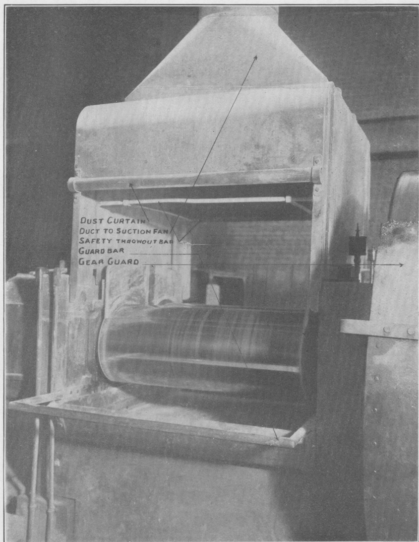
PLATE 4.—A MIXING MILL.
