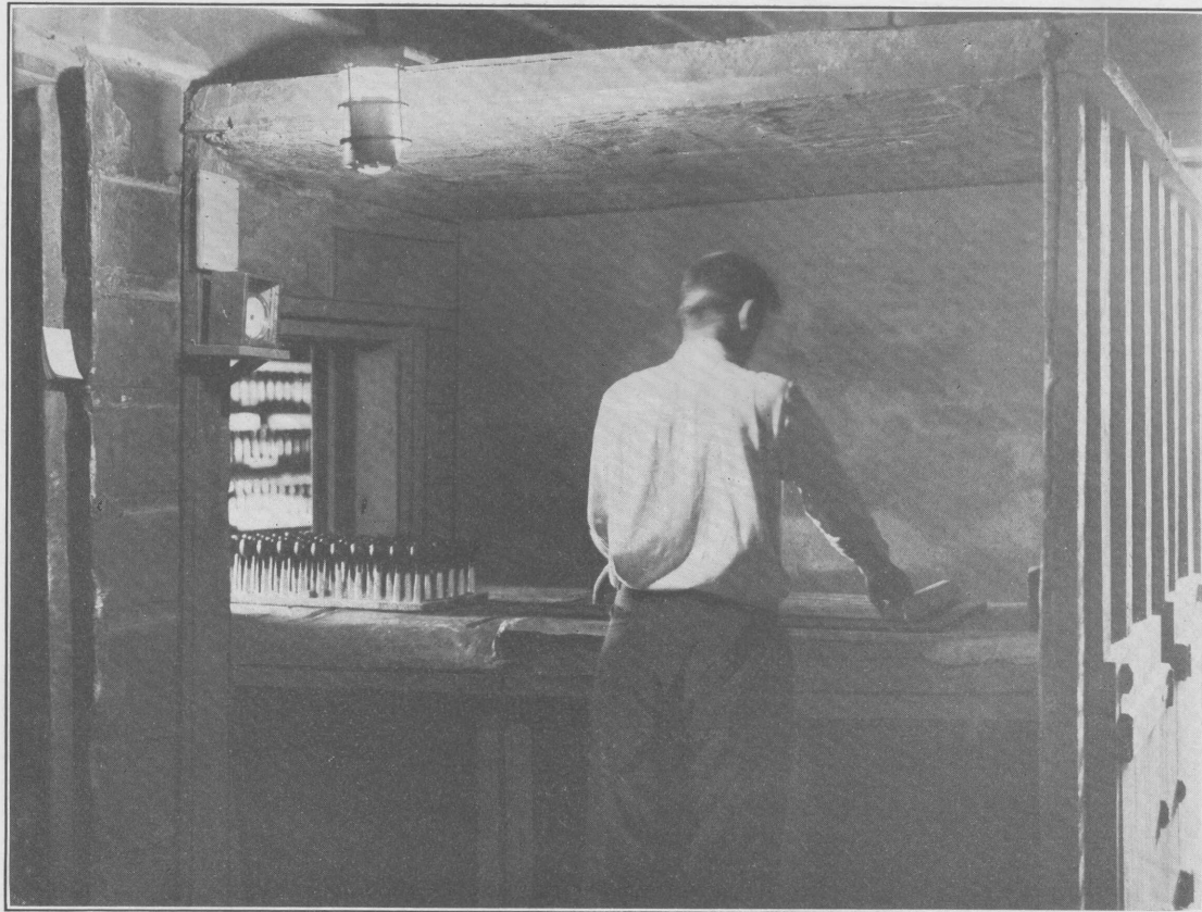
PLATE 13.—ACID CURING OR COLD CURING OF BALLOONS.
