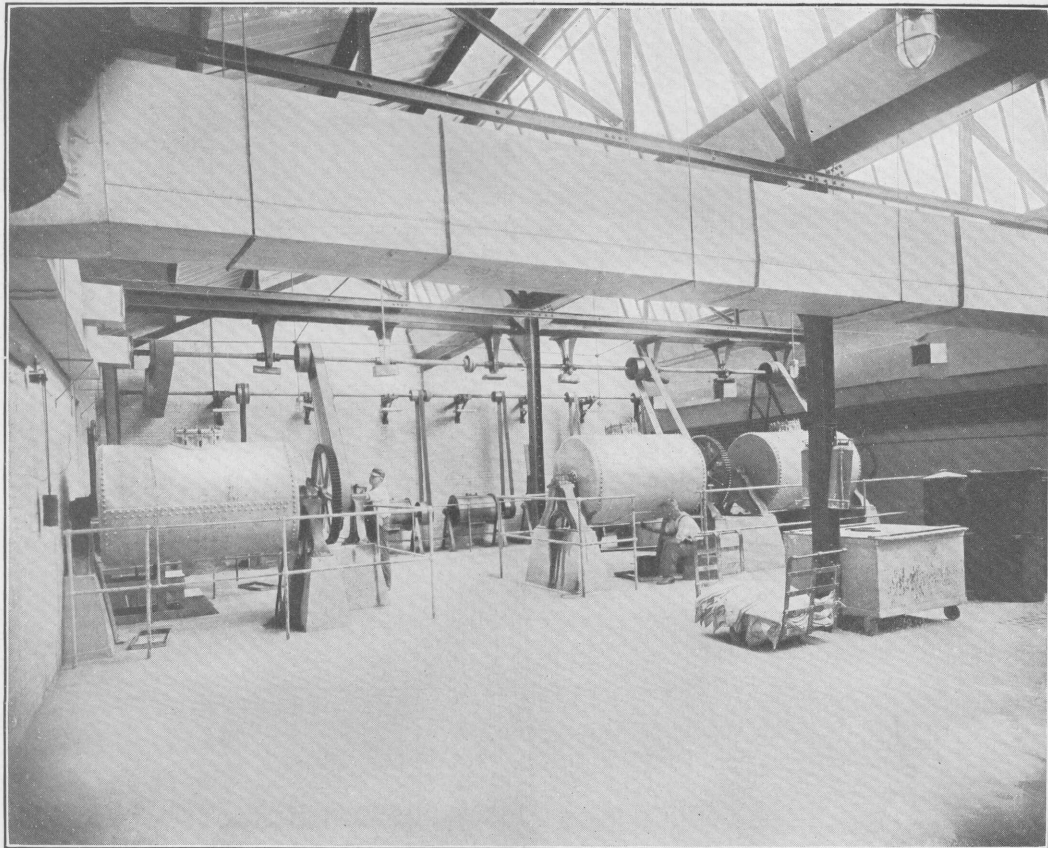
PLATE 7.—CEMENT CHURNING ROOM.
