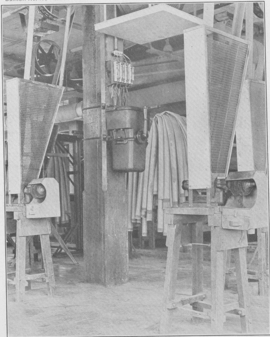
PLATE 6.—MACHINE FOR ROUGHENING ENDS OF INNER TUBES.
