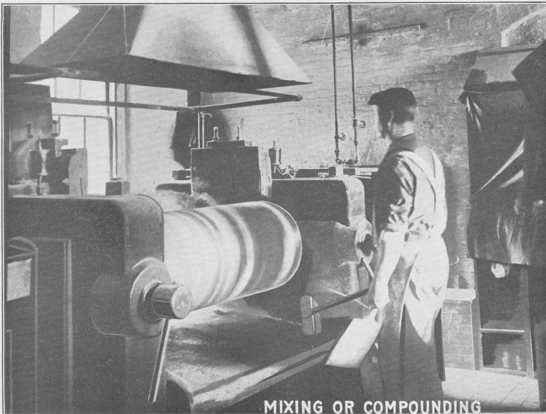
PLATE 2.—MIXING OR COMPOUNDING.
