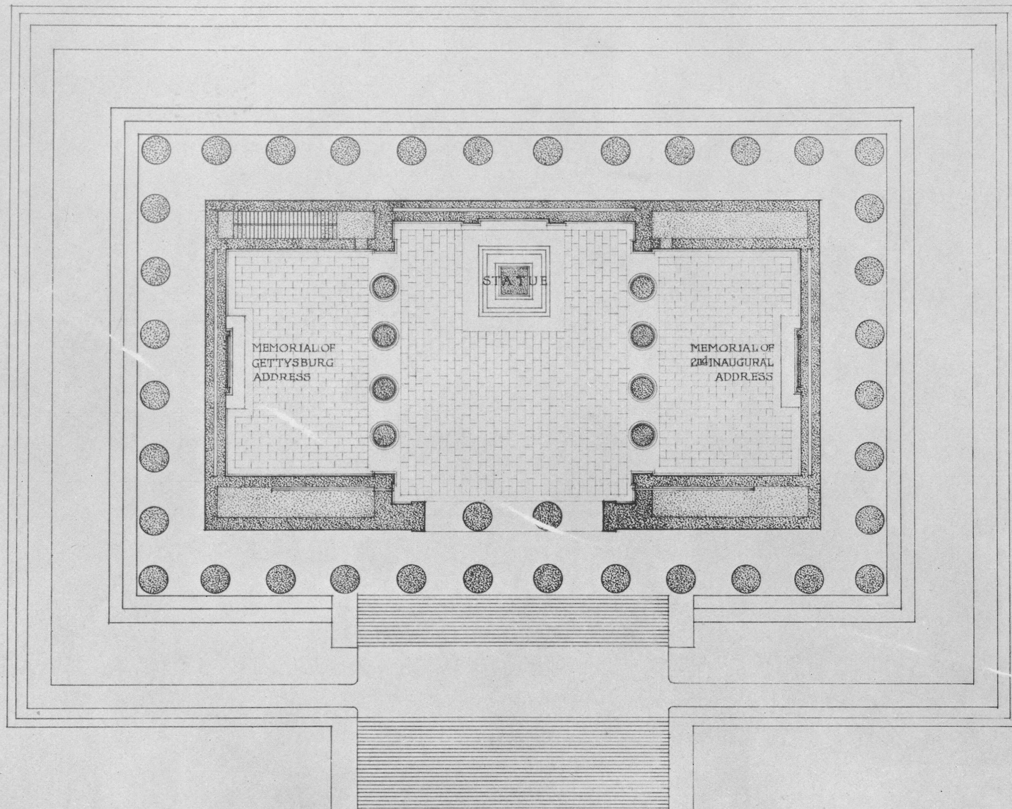
PLAN OF LINCOLN MEMORIAL Scale 20 40 60 80 100 Feet
