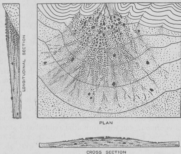
FIGURE 3.—Diagrammatic plan and sections of alluvial fan, showing arrangement of debris. Sketch contours do not show channeling of fan.
