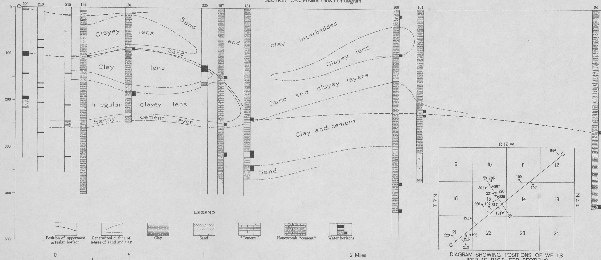
WELL SECTIONS AND DIAGRAM SHOWING PROBABLE UNDERGROUND CONDITIONS AT LANCASTER AND VICINITY AS INDICATED BY WELL LOGS
