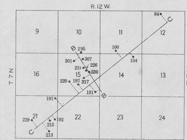
DIAGRAM SHOWING POSITIONS OF WELLS USED AS BASIS FOR SECTIONS
