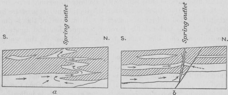
FIGURE 6.—Diagrams showing possible origin of Buckhorn Springs.
