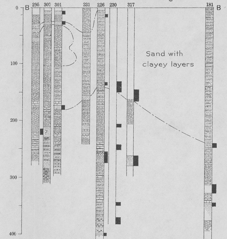
SECTION B-B. Position shown on diagram
