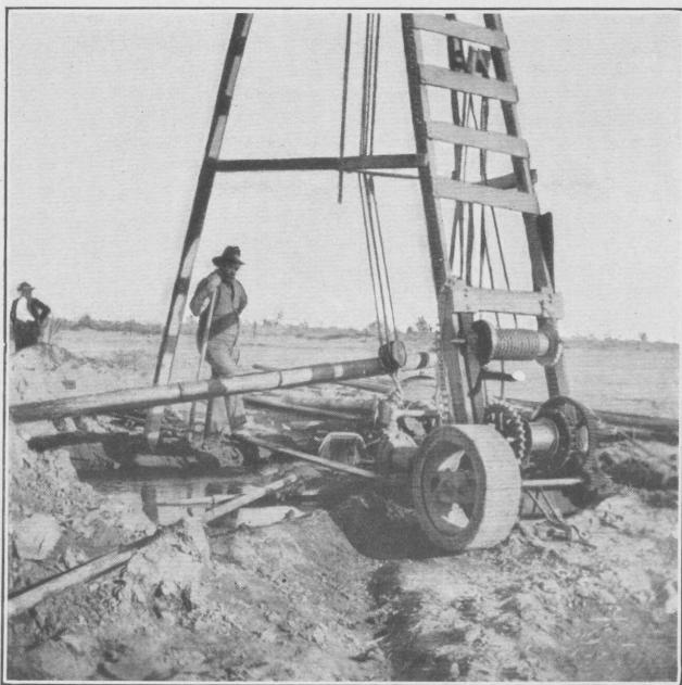
A. TYPE OF WELL-DRILLING RIG USED IN ANTELOPE VALLEY.
