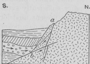
FIGURE 10.—Diagram showing possible origin of Gerblick Spring.
