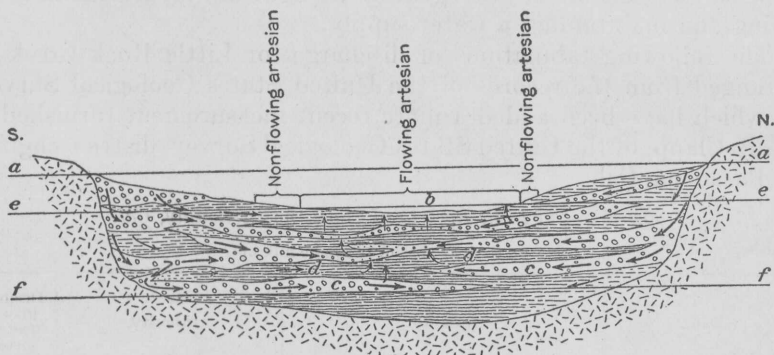
FIGURE 4.—Diagram showing artesian conditions in Antelope Valley.
