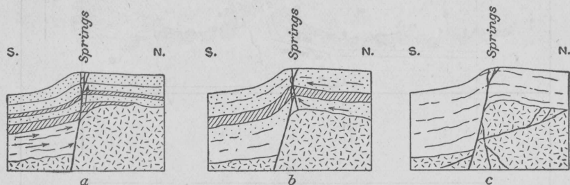
FIGURE 8.—Diagrams showing possible origin of Willow Springs.
