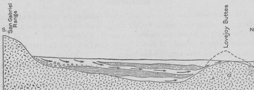
FIGURE 9.—Diagram showing the origin of Lovejoy Springs.
