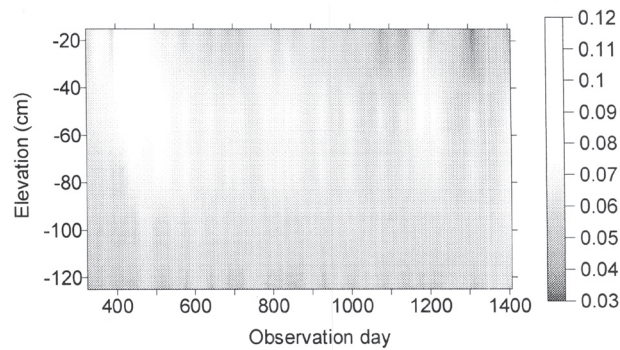
Figure 2. Image map of soil water contents monitored for 3 years (along with soil temperatures) at the USGS Amargosa Research Site, Nevada.
