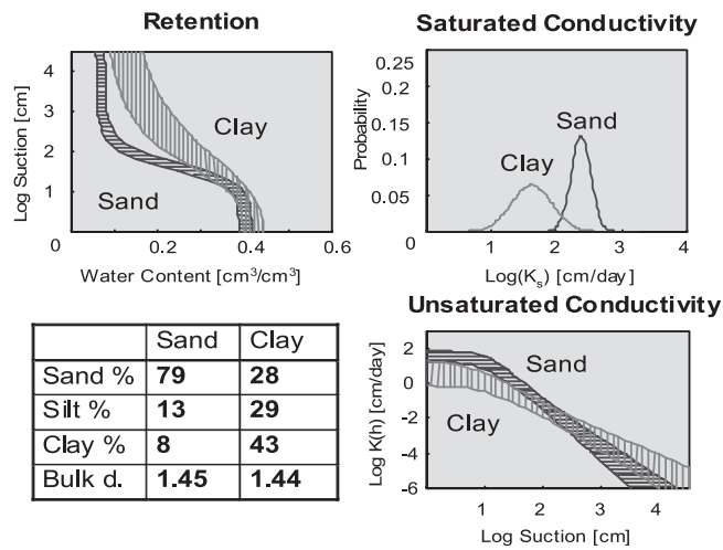
Figure 1. Examples of 90% confidence intervals generated with Rosetta for water retention and the unsaturated hydraulic conductivity for two soils.
