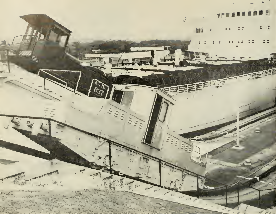
Japanese-built locomotive, with single cab, and an old-style locomotive with cab on each end pass each other on Gatun Locks center wall incline.
