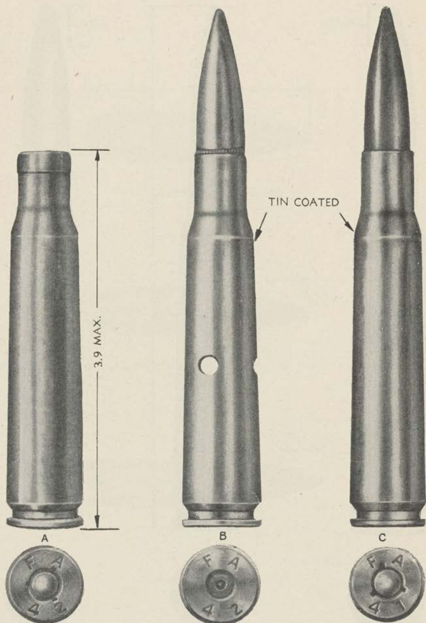
FIGURE 24.—Blank, dummy, and high-pressure test cartridges, caliber .50.
