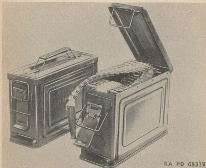
FIGURE 12.1.—Packing box M1 (steel) for 250 caliber .30 cartridges in web belts.
