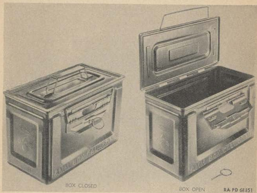
FIGURE 12.2.—Packing box M2 (steel) for 110 caliber .50 cartridges in web belts.
