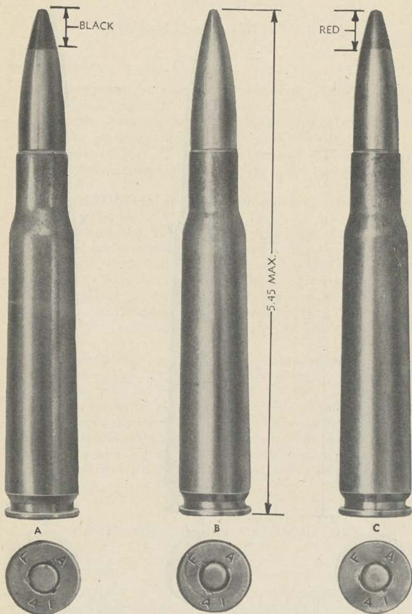
FIGURE 23.—Armor-piercing, ball, and tracer cartridges, caliber .50.
