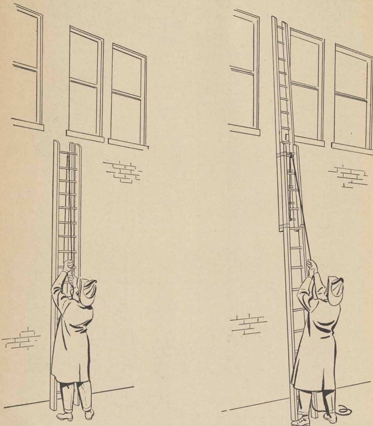
Figure 36. One-man raise for extension ladder.
