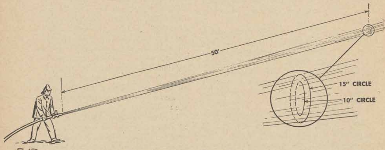
Figure 76. Requirements for solid fire stream.
