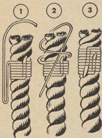
WHIPPING THE END OF A ROPE
