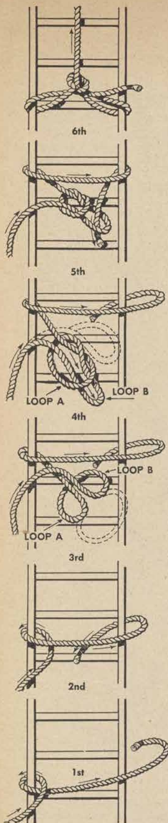
① Six steps in making ladder hoist.
