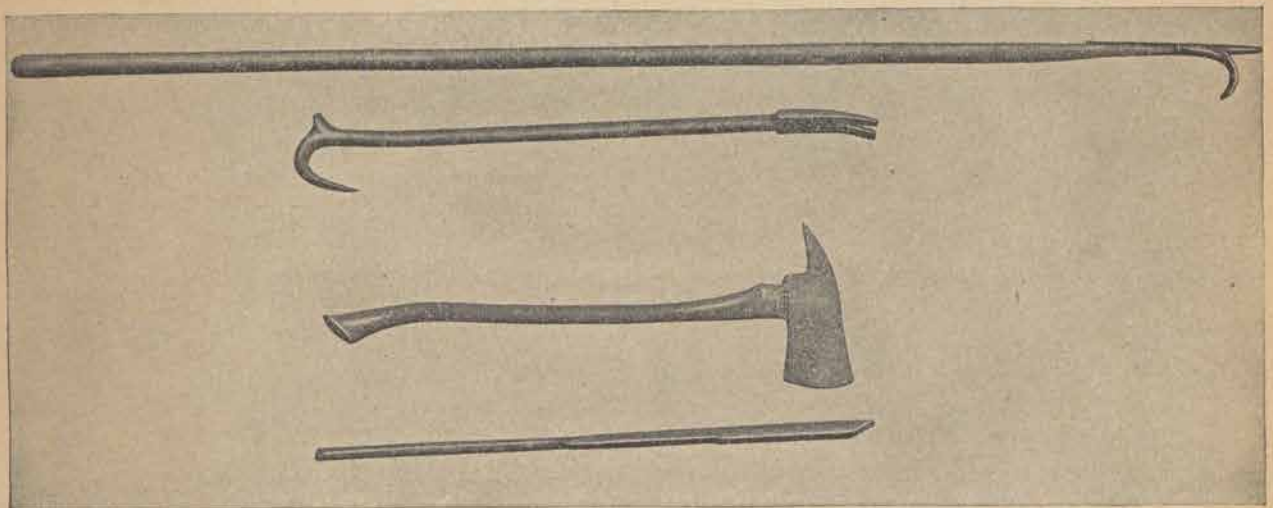
Figure 8. Forcible-entry tools furnished on Corps of Engineer fire trucks. Shown are pike pole, door opener, pick-headed ax, and crowbar.
