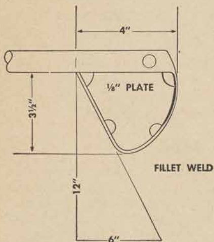
Figure 42. Type of hose clamp that can be made locally.
