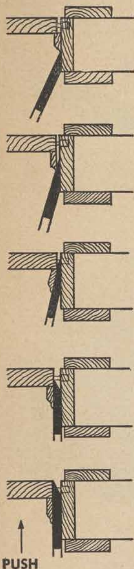
Figure 13. Springing a door in a stopped frame with a door opener. Tool should be used to separate lock and jamb enough for lock to pass keeper.
