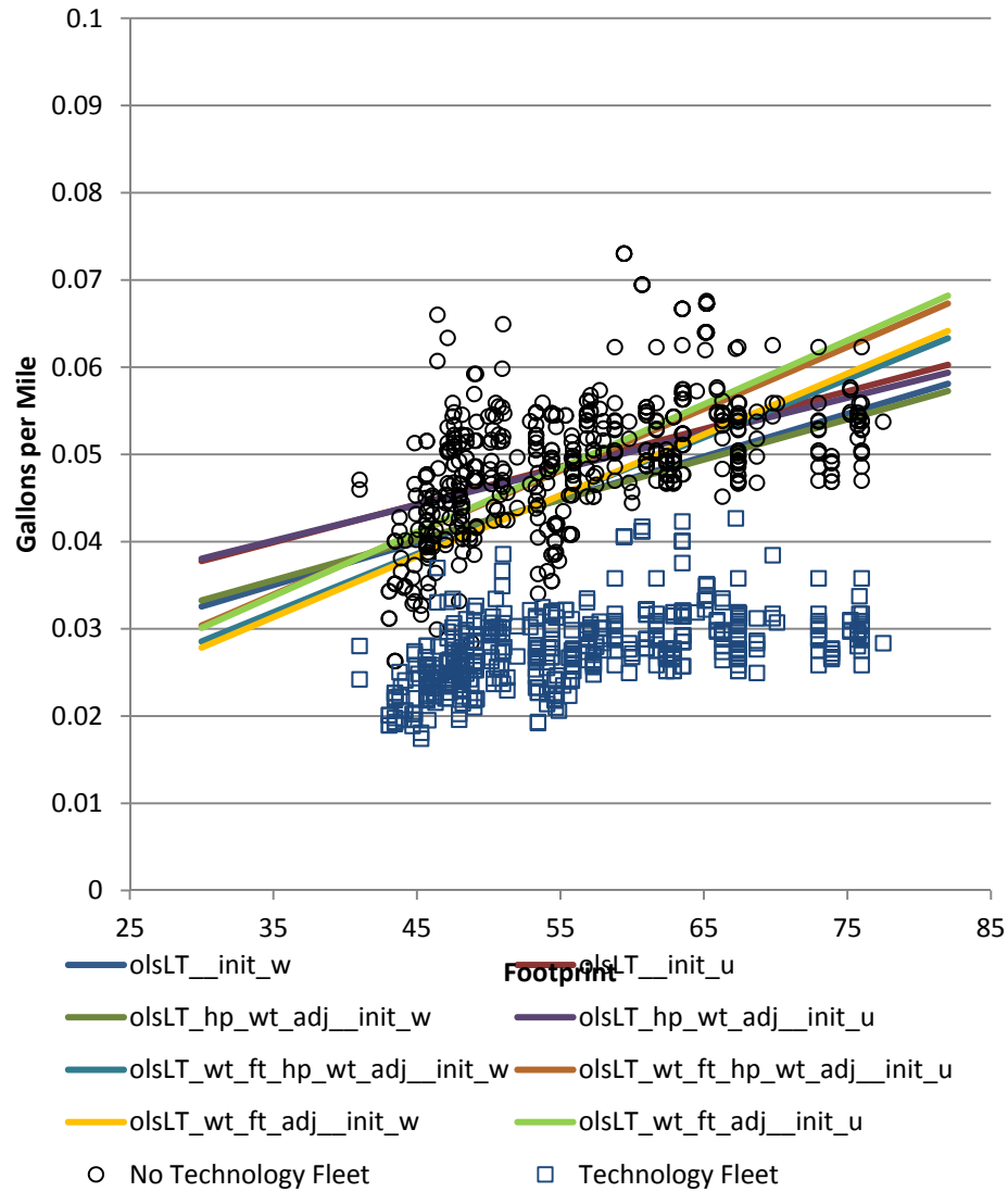
Figure V-11 Best Fit Results for Various Regressions: Trucks, No Added Technology, OLS
