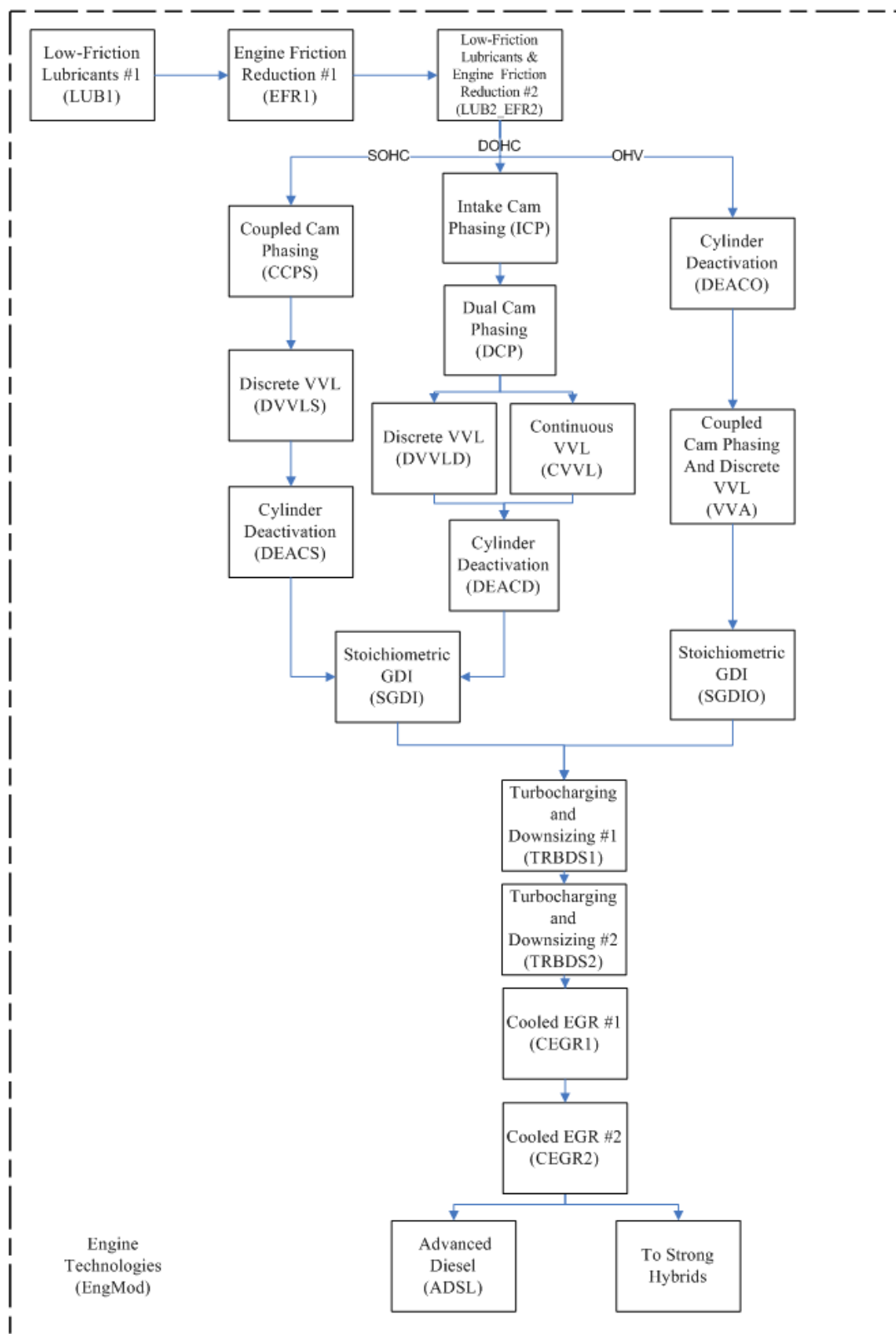
Figure V-29. Engine Technology (EngMod) Decision Tree
