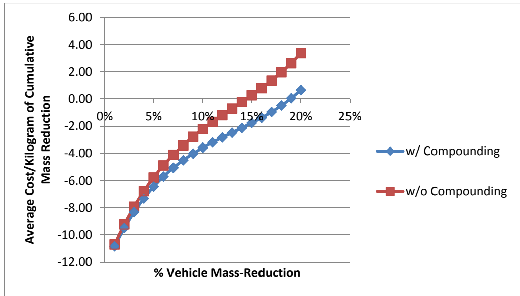
Figure V-47 Cost Curve for the 2010 Toyota Venza – EPA Study (FEV/EDAG/Munro)
