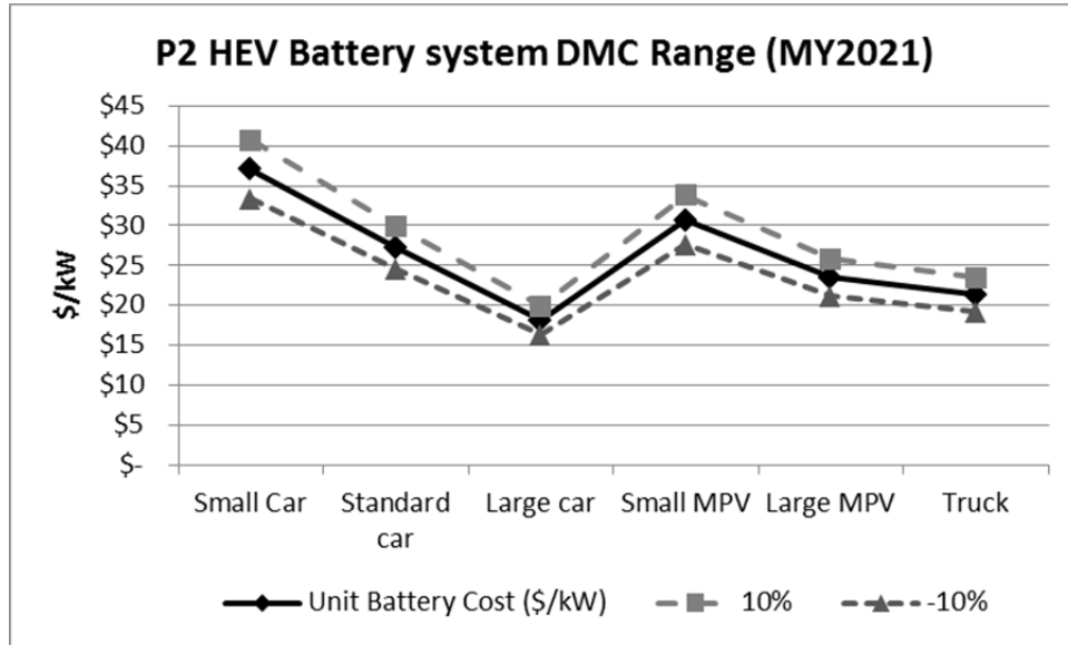
Figure X-1 Battery System Direct Manufacture Cost (DMC) for P2 HEV
