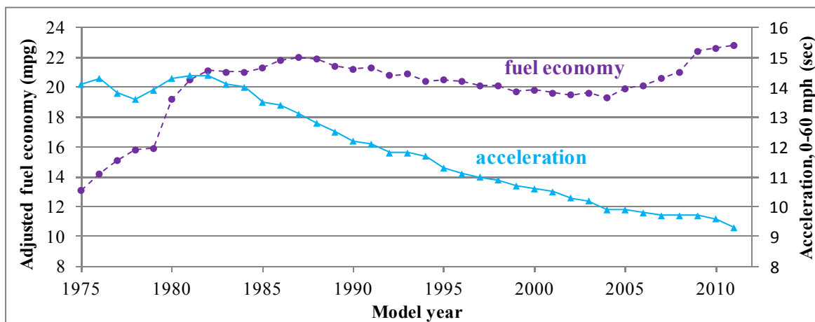
Figure V-38 Light duty fleet trends for acceleration and fuel economy: 1975-2011
