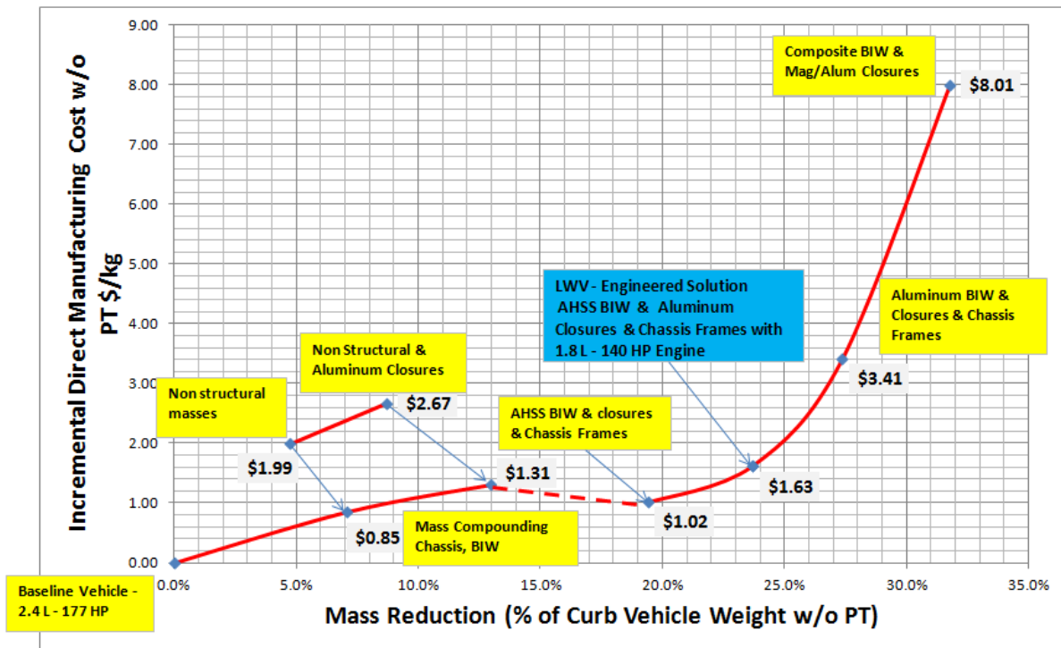
Figure V-46. Mass Reduction Cost for the Glider Only
