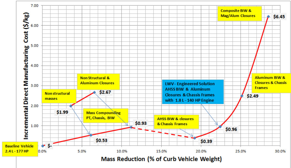
Figure V-45 Mass Reduction Cost with Allowance for Powertrain Downsizing
