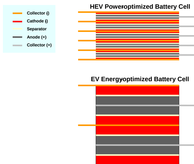
Figure V-33: Schematic representation of power and energy optimized prismatic-layered battery cells
