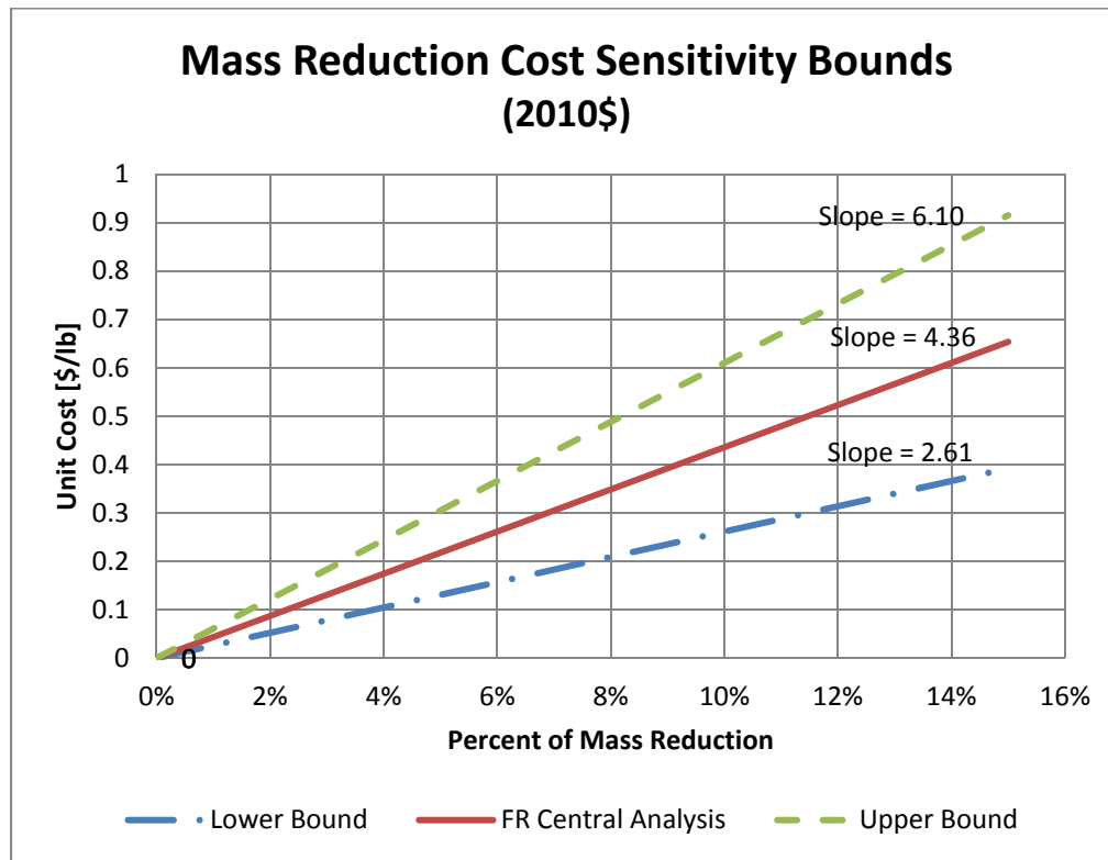
Figure X-6 Direct Manufacturing Cost for Mass Reduction (2010$)
