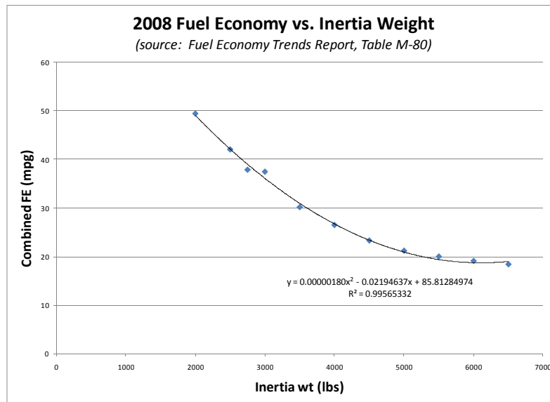
Figure V-34 Average fuel economy based on inertia weight (ETW) from FE Trends data
