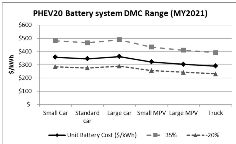
Figure X-2 Battery System Direct Manufacture Cost (DMC) for PHEV20
