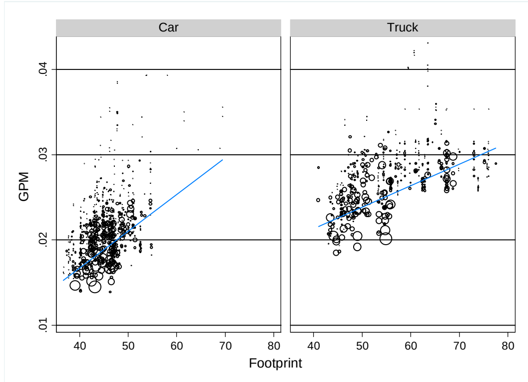
Figure V-8 HP/WT Adjusted Fuel Consumption v. Footprint
