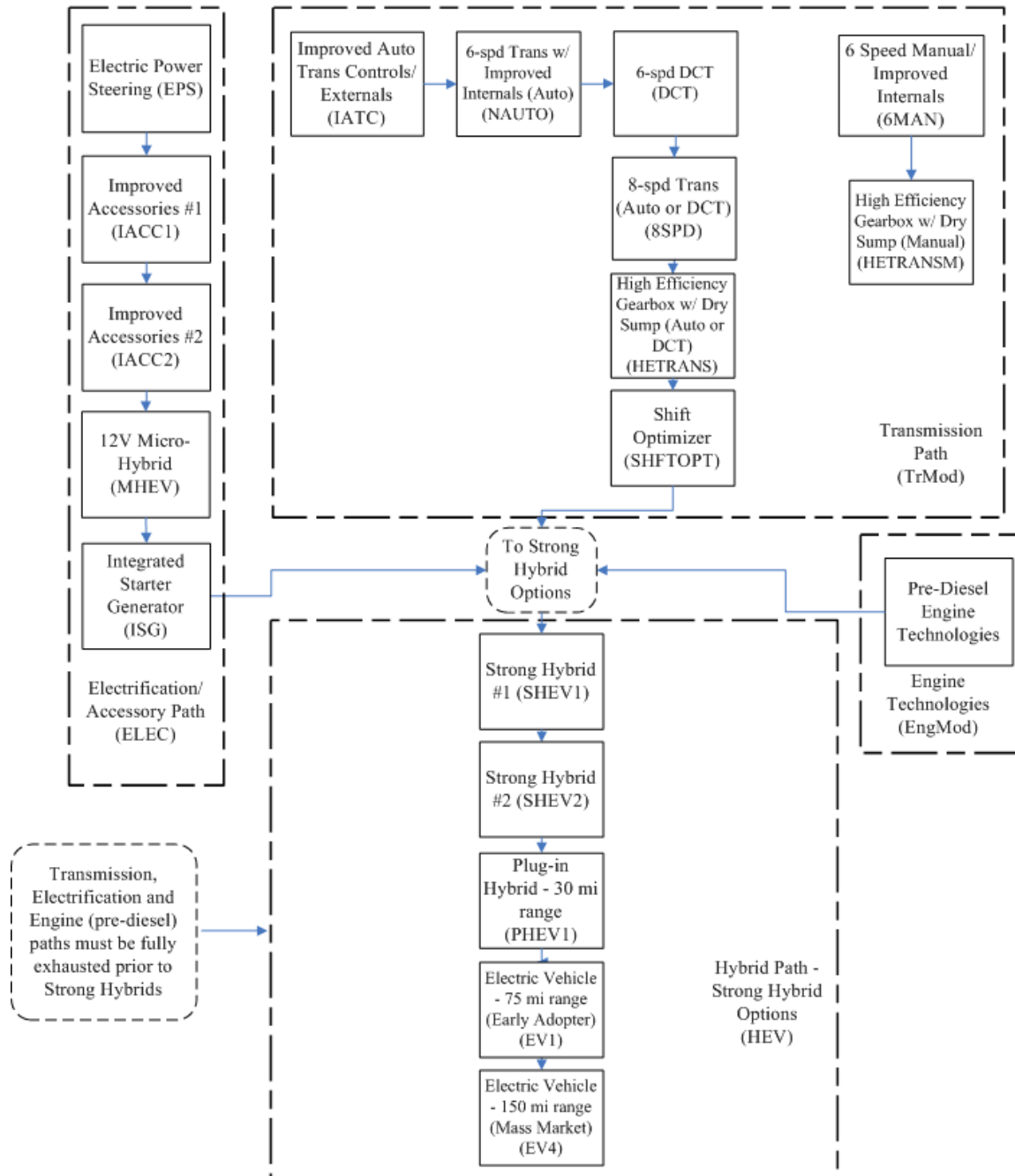
Figure V-30. Electrification/Accessory, Transmission and Hybrid Technology Decision Tree
