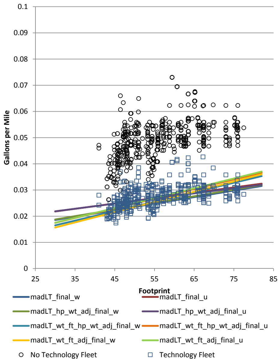
Figure V-16 Best Fit Results for Various Regressions: Trucks, with Added Technology, MAD
