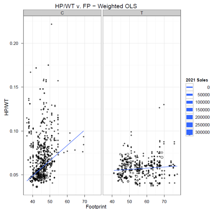
Figure V-6 HP/WT v. FP
