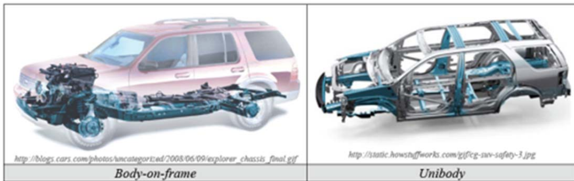
Figure V-42 Illustration of Body-on-Frame (BoF) and Unibody vehicle construction
