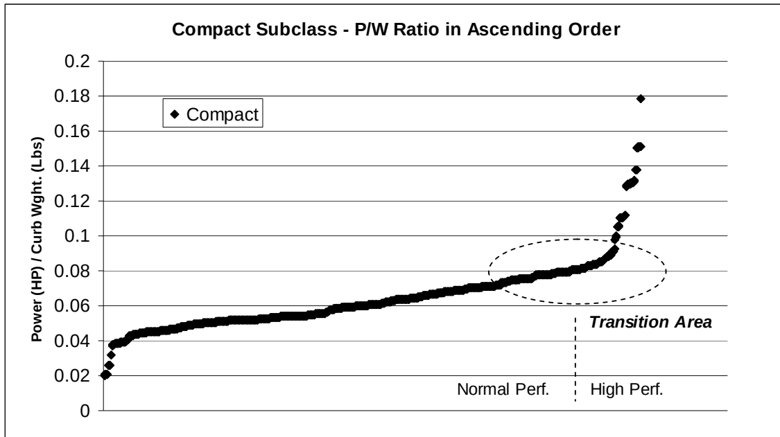
Figure V-32 Power/Weight Ratio for Compact Subclass
