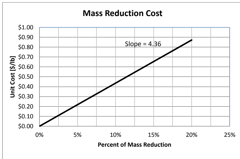
Figure V-44 Mass Reduction Direct Manufacturing Cost ($/lb)
