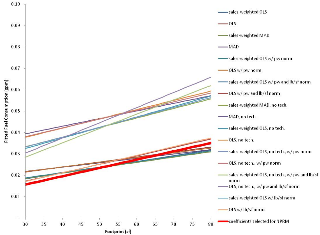
Figure V-23 Fitted Lines, Light Trucks, NPRM Analysis
