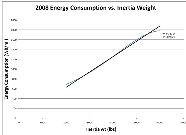
Figure V-35 Equivalent energy consumption (in Wh/mi) for baseline vehicles
