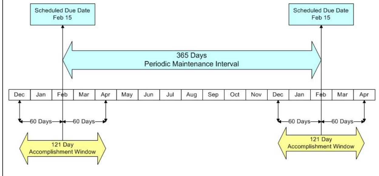
Figure 3-2. Annual PM Interval Example.
