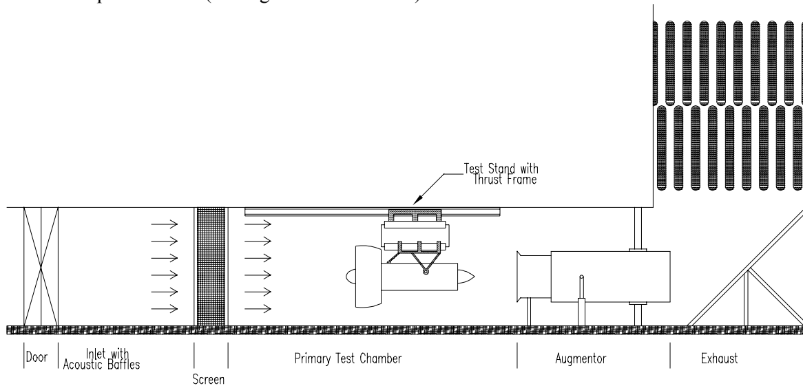
FIGURE 2-1. TEST CELL CONFIGURATION: “L” TYPE
