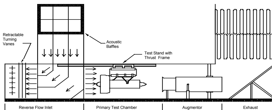
FIGURE 2-3. TEST CELL CONFIGURATION: FOLDED INLET TYPE
