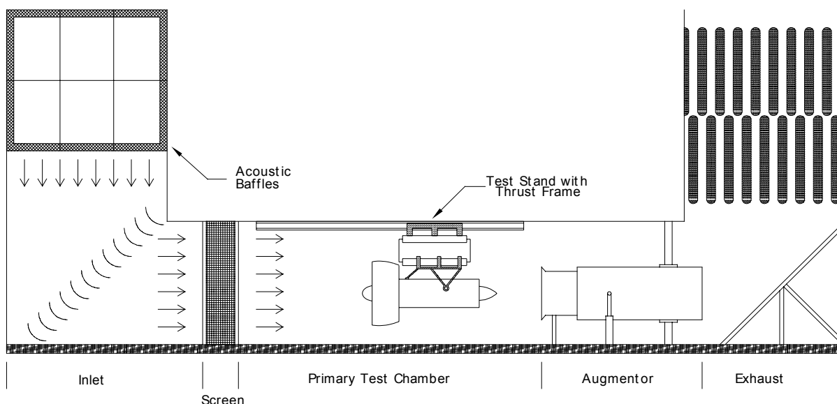
FIGURE 2-2. TEST CELL CONFIGURATION: “U” TYPE
