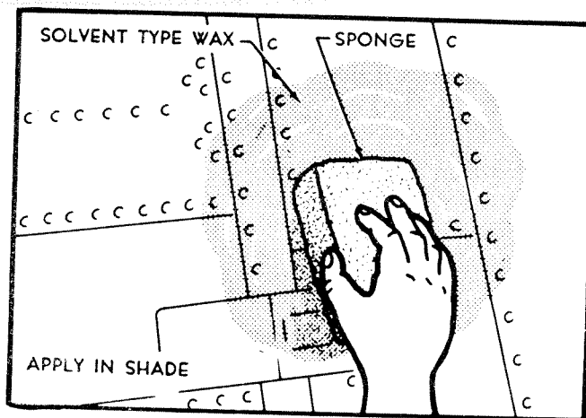
FIGURE 6-16. APPLYING WAX TO CLEANED SURFACES
