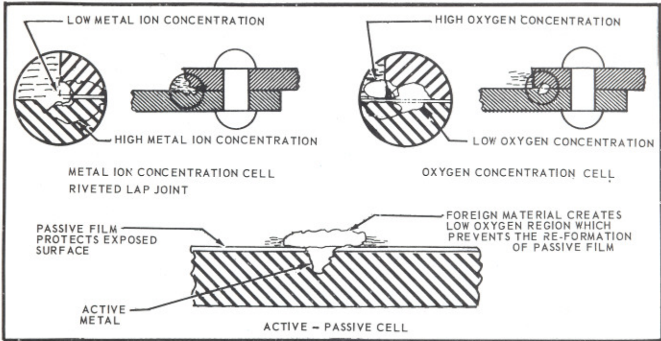
FIGURE 2-6. CONCENTRATION CELL CORROSION
