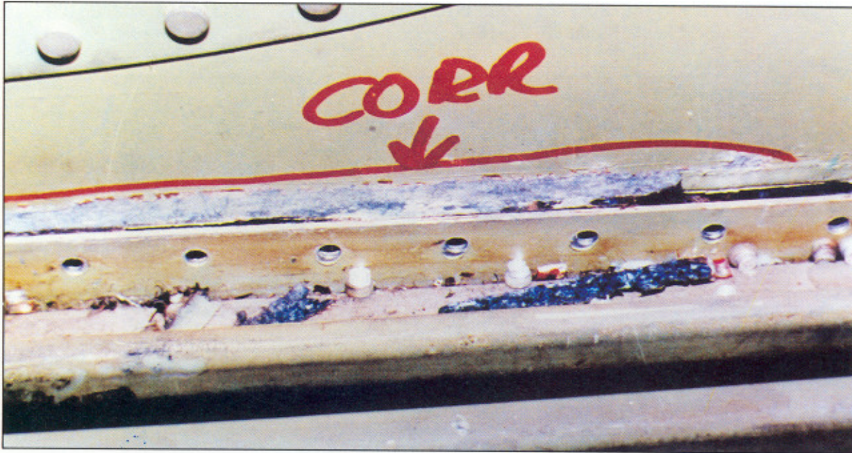
FIGURE 5-10. REMOVAL OF FILLET SEAL FROM INTERNAL EDGE OF LAP JOINT EXPOSED FULL EXTENT OF CORROSION
