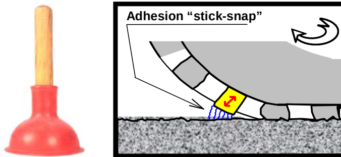
Figure 13. “The Suction Cup” generation mechanism.
