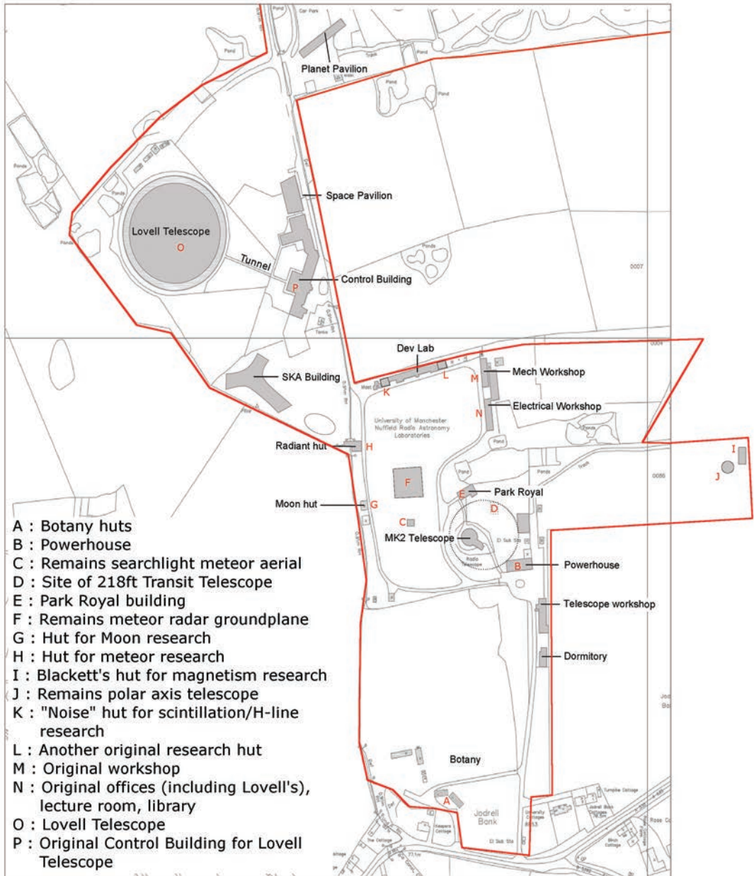
1. Layout of the Jodrell Bank Observatory site (edged in red). Various current and heritage features are labeled. Courtesy of The University of Manchester.
