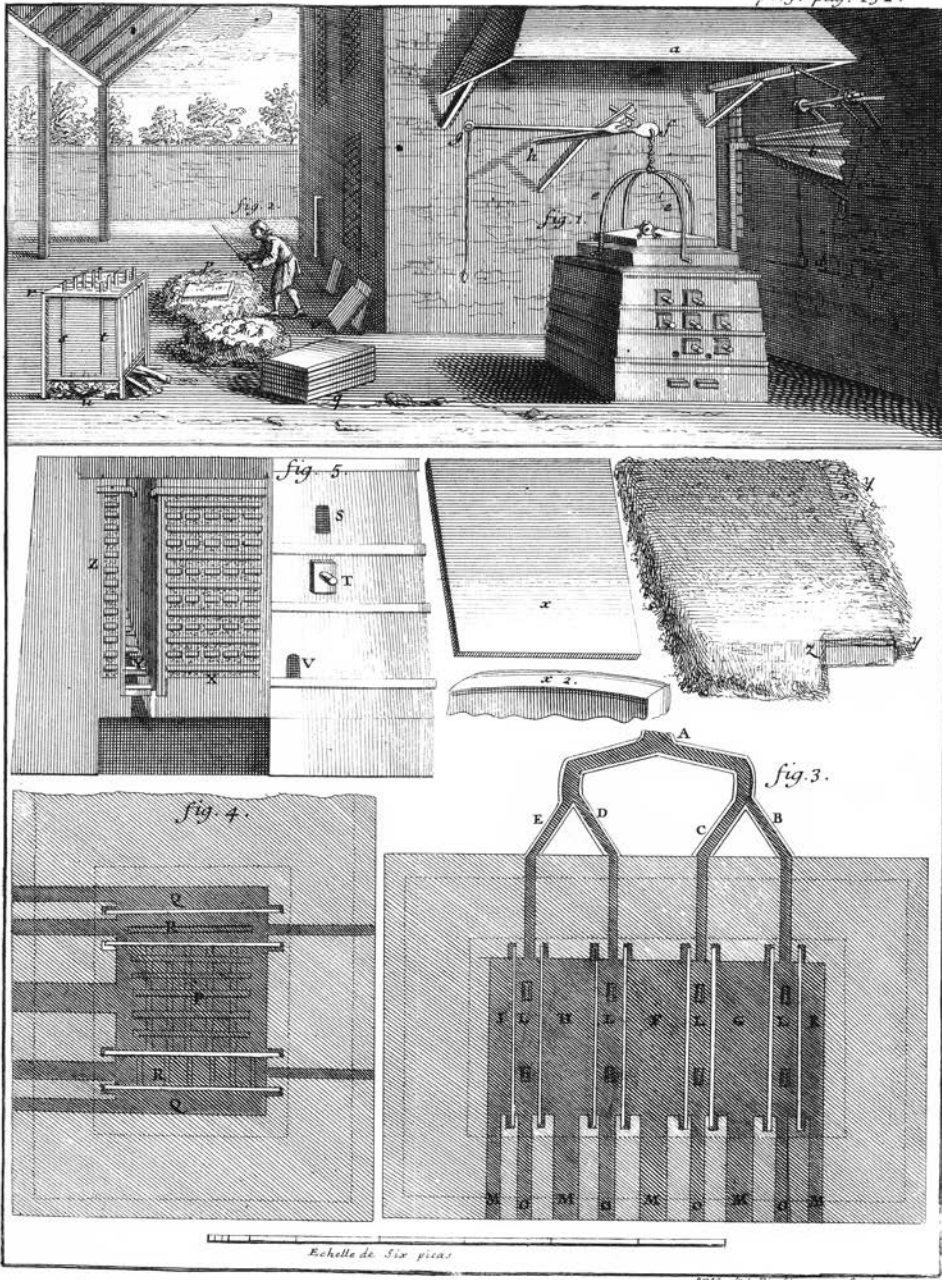
3. Cement-steel works, René Antoine Ferchault de Réaumur, 1722. Photo: Deutsches Museum Archives.
