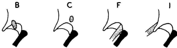
FIGURE 1.—Omohyoideus character states.
