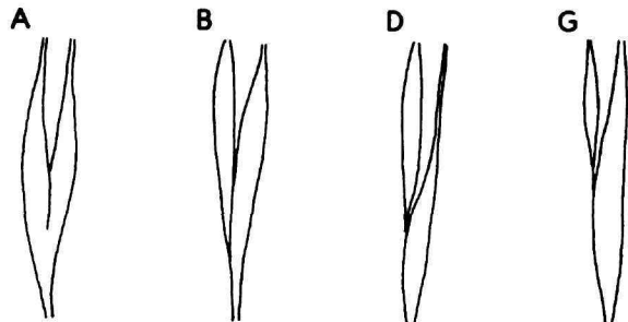
FIGURE 3.—Semitendinosus character states.
