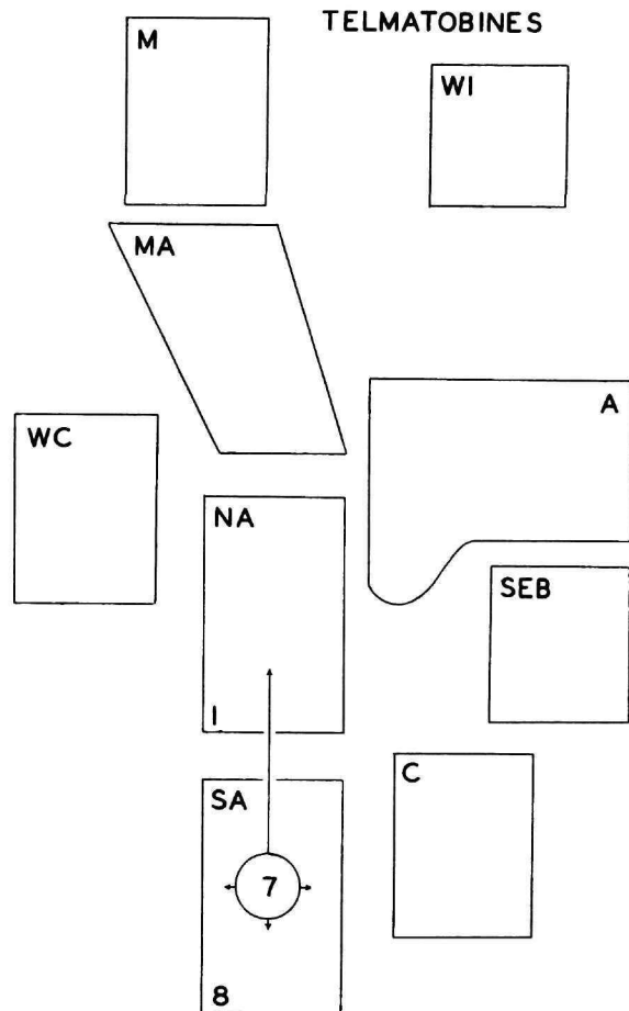
FIGURE 12.—Proposed telmatobine radiation. (Number in circle is number of endemic genera; numbers at bottom are total number of genera; abbreviations as in legend for Figure 10.)
