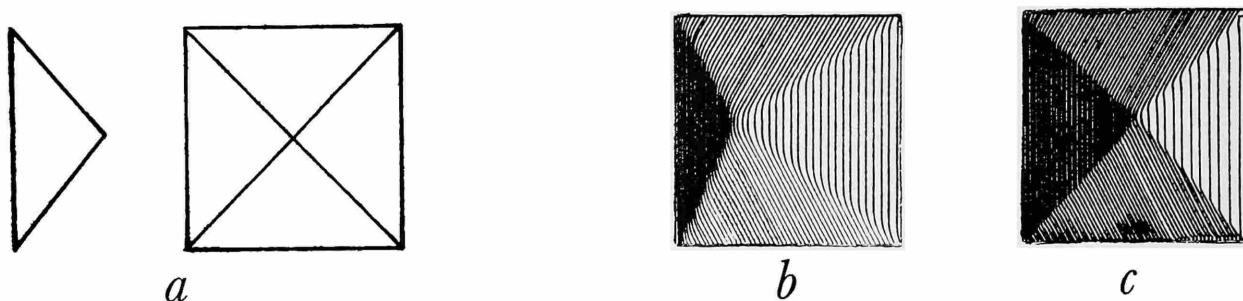
FIGURE 6.—Images produced with the Saxton medal ruling machine: a , side and top views of pyramid-shaped model used in tests; b , image produced with a horizontal arm simulating Goebrecht's design; c , image produced with Saxton's improved diagonal tracer.
