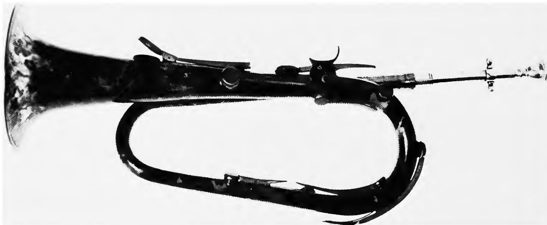
Figure 9. Tortoise-shell bugle marked "George Shaw, Thompson Ct.," patented 1845. In e_b or f , nine keys with channel-shaped shanks over block mounts. Hole covers are cupped for stuffed pads. Mouthpiece and shank not original. USNM 251,395.
