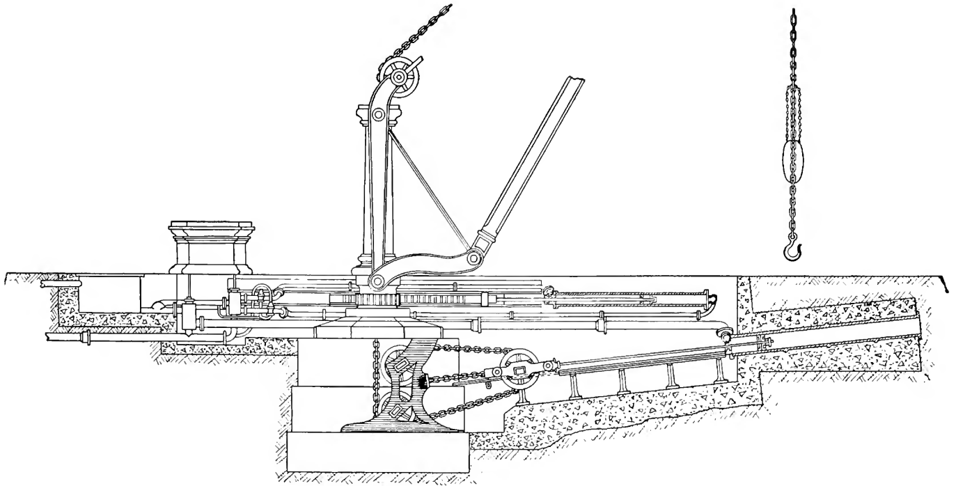
FIGURE 3.—The hydraulic crane was rationalized in 1846 by William Armstrong, who eliminated the winding drum and used the hydraulic piston to draw apart the two elements of an inverse rope tackle. As the sheaves were separated, the tackle's free end was drawn in raising the hook and its load, in the machine shown at three times the piston's travel and speed. The smaller hydraulic cylinder above drove a rack to slew (rotate) the crane. The main
