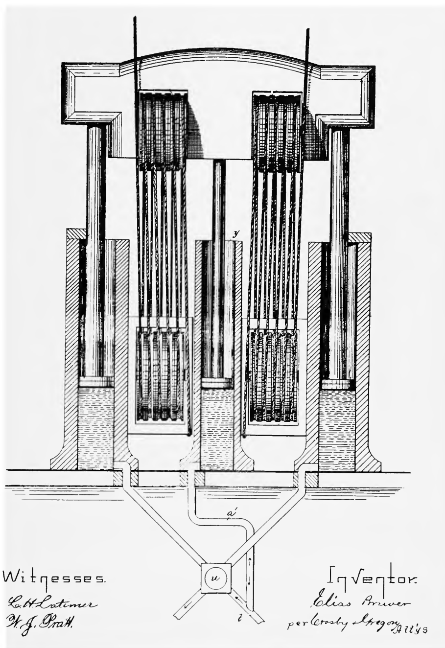
FIGURE 25.—The drawing accompanying Elias Brewer's (apparently) sole patent of 10 April 1877. Although the patent's claims of originality differed somewhat from those of Timothy Stebins's only slightly earlier patent, it is difficult to avoid the conclusion that Brewer was strongly influenced by the prior work of his fellow Bostonian. A principal Brewer claim was counterbalancing of the elevator's dead weight by constant application to the piston in the central cylinder (y) of pressurized water from the supply main—through pipe (a) which was connected to the main ahead of the control valve (u). When the car descended (by gravity), the water in the balance cylinder simply was forced back into the main.
