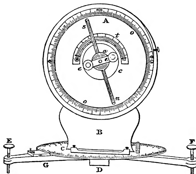
FIGURE 17.—Fox’s “dipping needle deflector,” introduced in 1835. (From Annals of Electricity , 3 (1839) Pl. V, fig. 47.) [Reference: T.B. Jordan, “Description and use of a dipping needle deflector invented by Robert Ware Fox,” Ibid , pages 288–297.]
