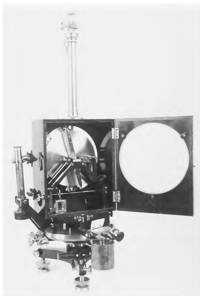
FIGURE 46 (facing page).—No. 17, Universal Magnetometer, CIW 19, 1911.
