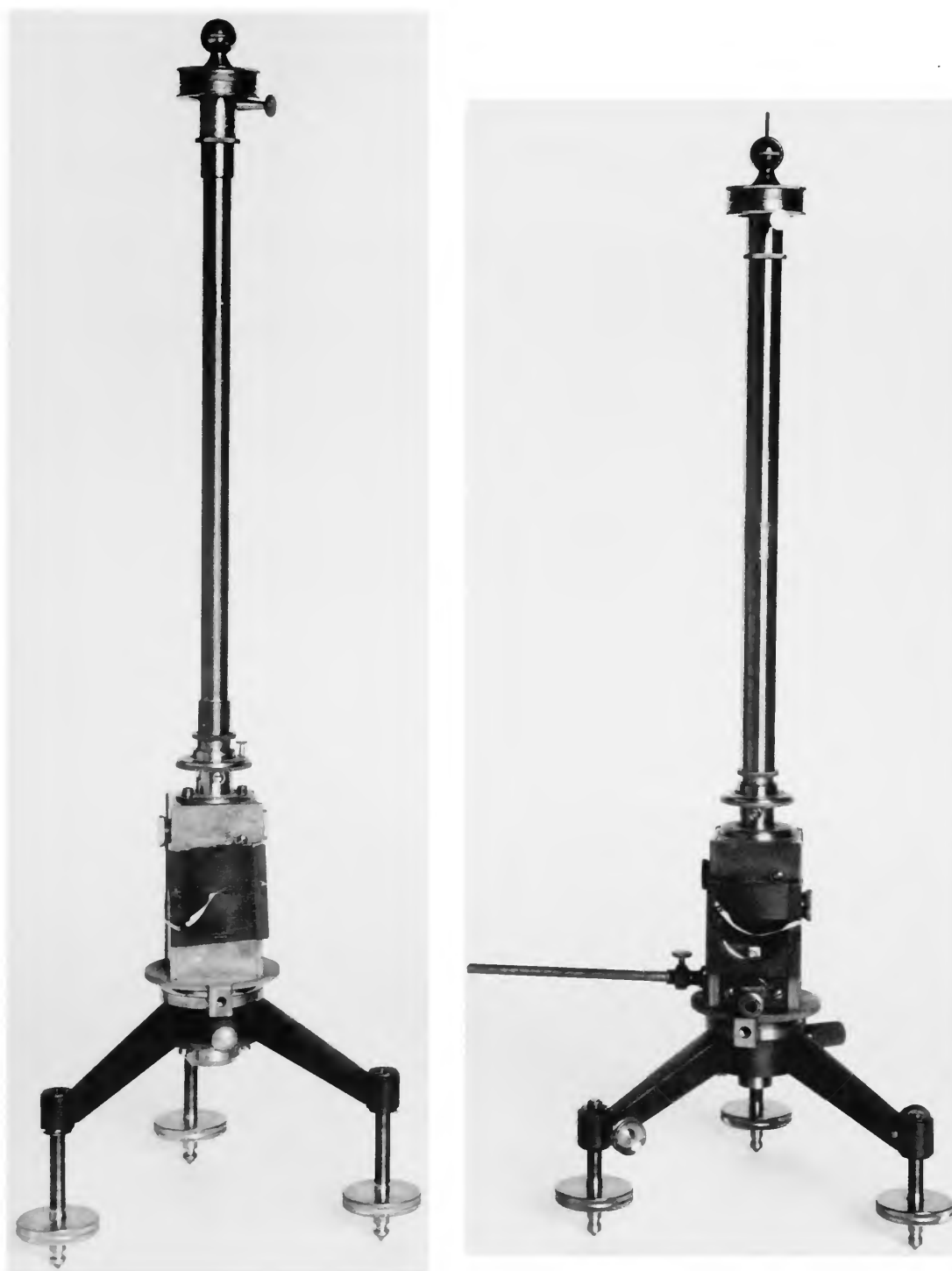
FIGURE 53.—No. 24, Variometers, Eschenhagen-Toepfer, ca. 1900.
