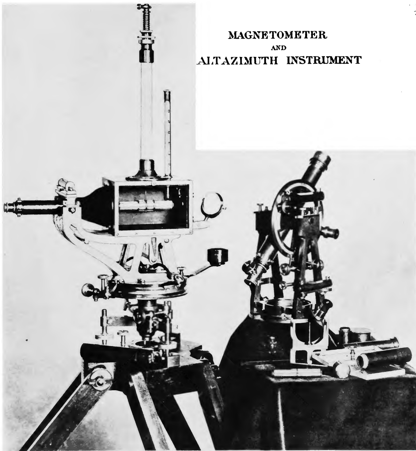
FIGURE 27.—Magnetometer and "altazimuth instrument" (theodolite) used by the Coast Survey in 1894, as illustrated in its Report for that year. No. 11 (Figure 39) in the present collection is an instrument of this type.
