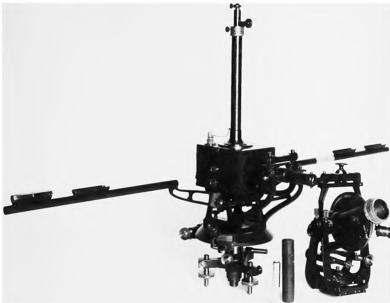
FIGURE 38 (facing page).—No. 10, Magnetometer, Brunner-Chasselton, ca. 1884.
