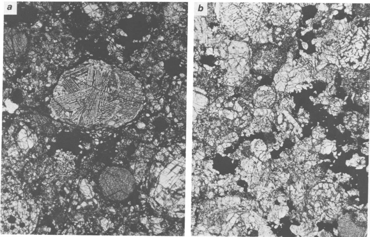
FIGURE 25.—H5 chondrites: a , ALHA77102, photomicrograph of thin section (width of field is 2.0 mm); note two juxtaposed barred olivine chondrules apparently fused together. b , ALHA77264, photomicrograph of thin section (width of field is 2.0 mm).
