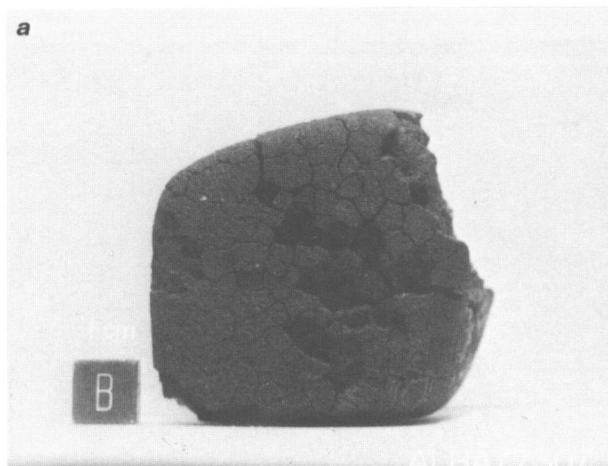
FIGURE 9.—ALHA77307, C3 chondrite: a , Fusion crust is crazed and broken away in places. b , Photomicrograph of thin section (width of field is 2.0 mm); irregular grains, aggregates, and rare chondrules of olivine and pyroxene (white or light gray) in dark brown to opaque matrix (black).
