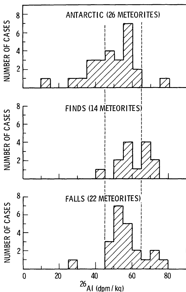
FIGURE 38.— ^{26}\text{Al} content of H- and L-type chondrites normalized to L-type composition.
