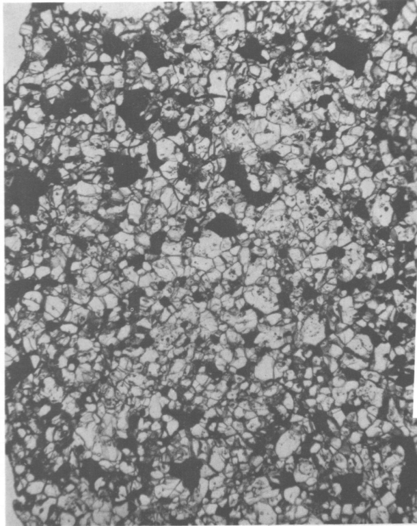
FIGURE 31.—ALHA77081, H?, photomicrograph of thin section (width of field is 2.0 mm); an equigranular aggregate consisting mainly of olivine and orthopyroxene (white to gray) with accessory nickel-iron, troilite, and chromite (black).
