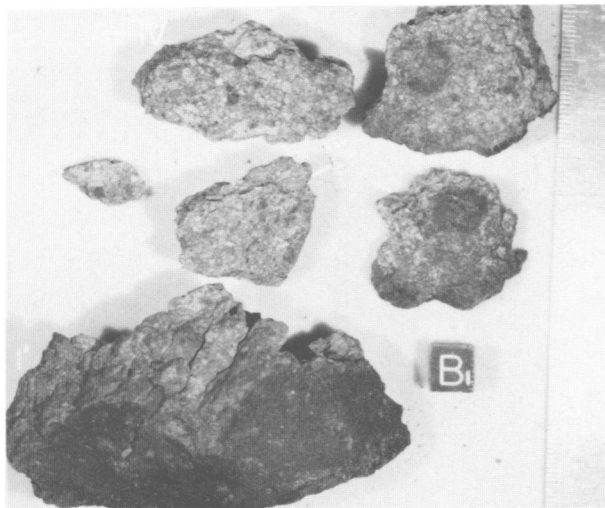
FIGURE 22.—ALHA77252, L4 chondrite; the stone broke into numerous fragments during transport from Antarctica, and light gray chondrules and lithic clasts are visible in the darker gray matrix; the largest fragment is partly covered with fusion crust.
