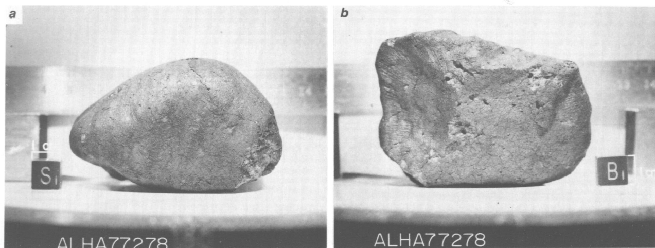
FIGURE 16.—ALHA77278, LL3 chondrite: a , Note conical form. b , Posterior surface showing radial flow lines in fusion crust.
