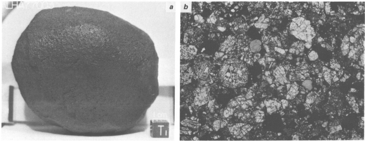
FIGURE 10.—H3 chondrites: a , ALHA77003, upper surface, showing fusion crust. b , ALHA 77299, photomicrograph of thin section (width of field is 2.0 mm); a closely packed mass of chondrules and irregular aggregates mainly of olivine and pyroxene set in a minor amount of dark matrix.
