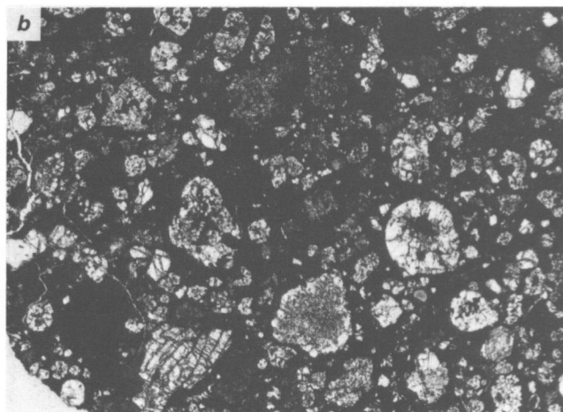
FIGURE 9.—ALHA77307, C3 chondrite: a , Fusion crust is crazed and broken away in places. b , Photomicrograph of thin section (width of field is 2.0 mm); irregular grains, aggregates, and rare chondrules of olivine and pyroxene (white or light gray) in dark brown to opaque matrix (black).
