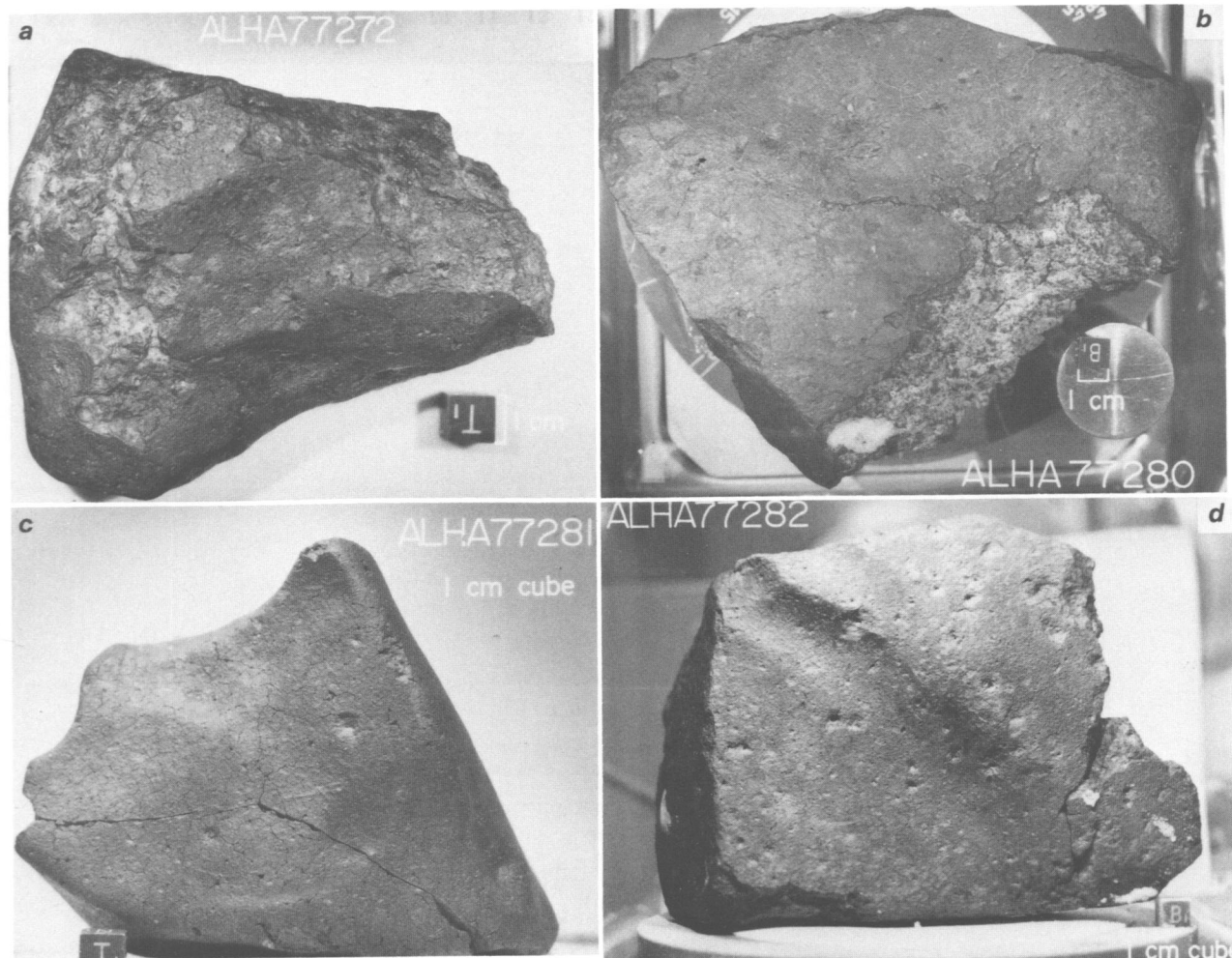
FIGURE 29.—L6 chondrites: a , ALHA77272, angular stone, partly coated with fusion crust. b , ALHA77280, stone with fusion crust partly spalled away. c , ALHA77281, a completely crusted stone showing some fracturing. d , ALHA77282, an incompletely crusted stone.
