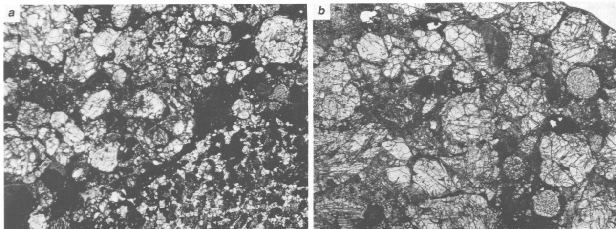
FIGURE 12.—L3 chondrites: a , ALHA77140, photomicrograph of thin section (width of field is 2.0 mm); chondritic material encloses a granular nonchondritic enclave. b , ALHA77160, photomicrograph of thin section (width of field is 2.0 mm); a close-packed aggregate of chondrules characteristic of type 3 chondrites.
