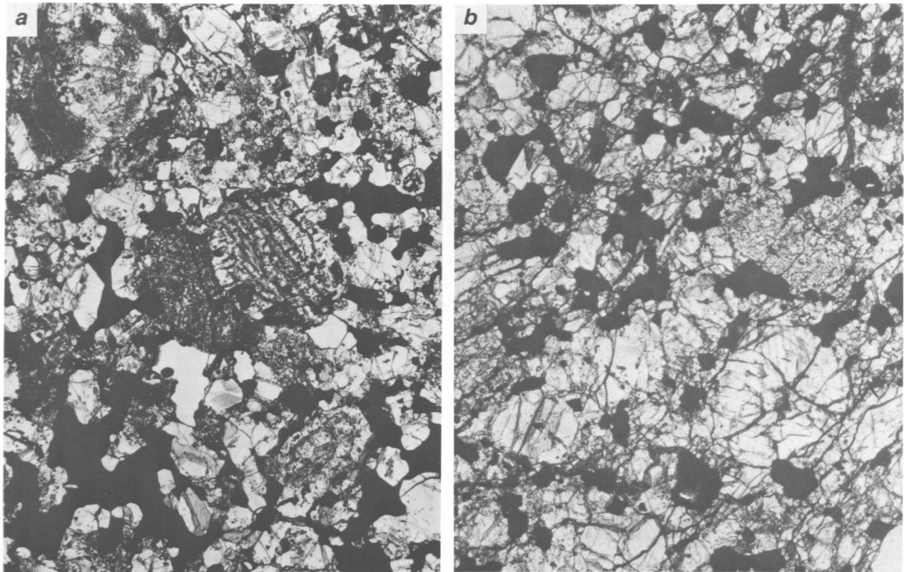
FIGURE 28.—H6 chondrites: a , ALHA77271, photomicrograph of thin section (width of field is 2.0 mm); chondrules are sparse and tend to merge with the granular matrix. b , ALHA77288, photomicrograph of thin section (width of field is 2.0 mm); chondrites are scarcely discernible from the granular matrix.
