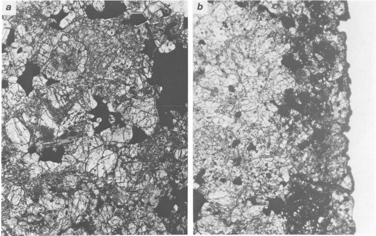
FIGURE 30.—L6 chondrites: a , ALHA77277, photomicrograph of thin section (width of field is 2.0 mm); chondrules are sparse and tend to merge with the granular matrix. b , ALHA77281, photomicrograph of thin section (width of field is 1.7 mm); note fusion crust on one edge, and almost total absence of chondritic structure.
