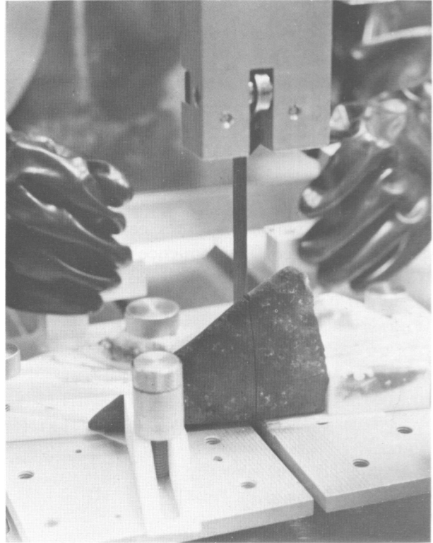
FIGURE 7.—An Antarctic meteorite being sawed with a band saw inside a stainless steel cabinet with a nitrogen atmosphere; no coolants are used.
