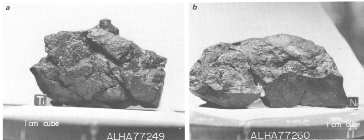
FIGURE 15.—L3 chondrites: a , ALHA77249, deeply fractured stone with remnants of fusion crust (lower right). b , ALHA77260, a fractured stone with fusion crust on the lower part.
