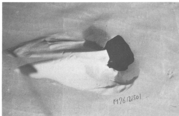
FIGURE 1.—Meteorite fragment found near Mt. Baldr. Eddy-current deposit of ice crystals has occurred downwind of the specimen; wind scooping has occurred at the sides.
