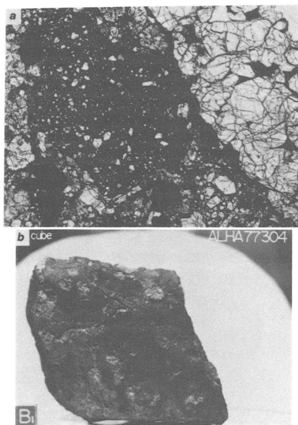
FIGURE 17.—LL3 chondrites: a , ALHA77278, photomicrograph of thin section (width of field is 2.0 mm); the center of the photograph is occupied by the carbonaceous(?) enclave described on p. 22, and also shows part of the granular olivine-orthopyroxene enclave. b , ALHA77304, fusion crust covers most of the surface, but has spalled off in small areas, revealing matrix material with numerous chondrules and lithic clasts.
