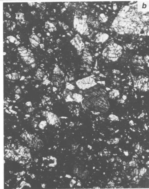
FIGURE 32.—ALHA77302, eucrite: a , Most of the surface is coated with black glassy fusion crust. b , Photomicrograph of thin section (width of field is 2.0 mm); an aggregate of plagioclase (white) and pigeonite (light to dark gray) clasts in a comminuted groundmass largely made up of the same minerals.
