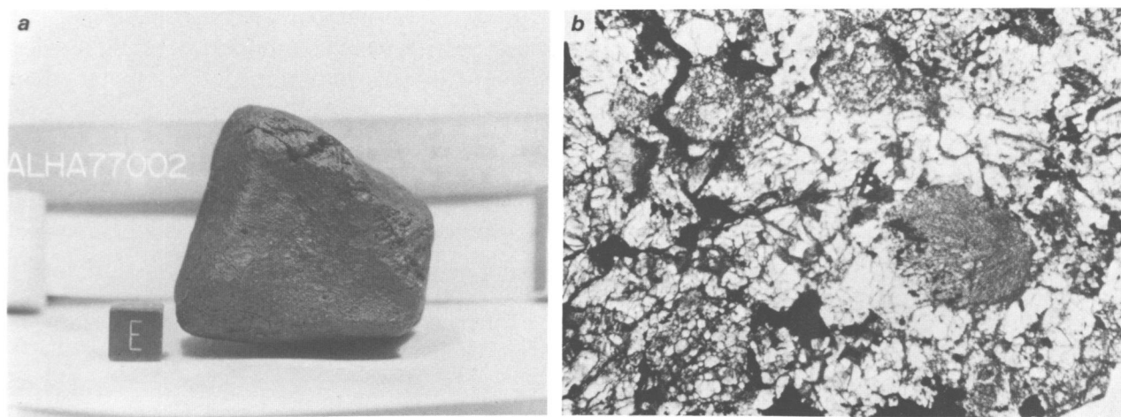
FIGURE 26.—L5 chondrites: a , ALHA77002, angular stone completely covered with fusion crust. b , ALHA77002, photomicrograph of thin section (width of field is 2.0 mm); prominent chondrules in a granular matrix.
