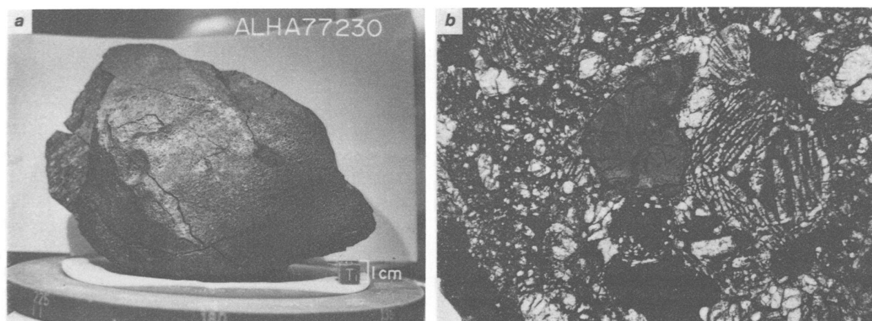
FIGURE 21.—ALHA77230, L4 chondrite: a , Stone with well-preserved fusion crust. b , Photomicrograph of thin section (width of field is 2.0 mm), showing large barred olivine chondrule and dark gray angular grain, possibly devitrified glass.
