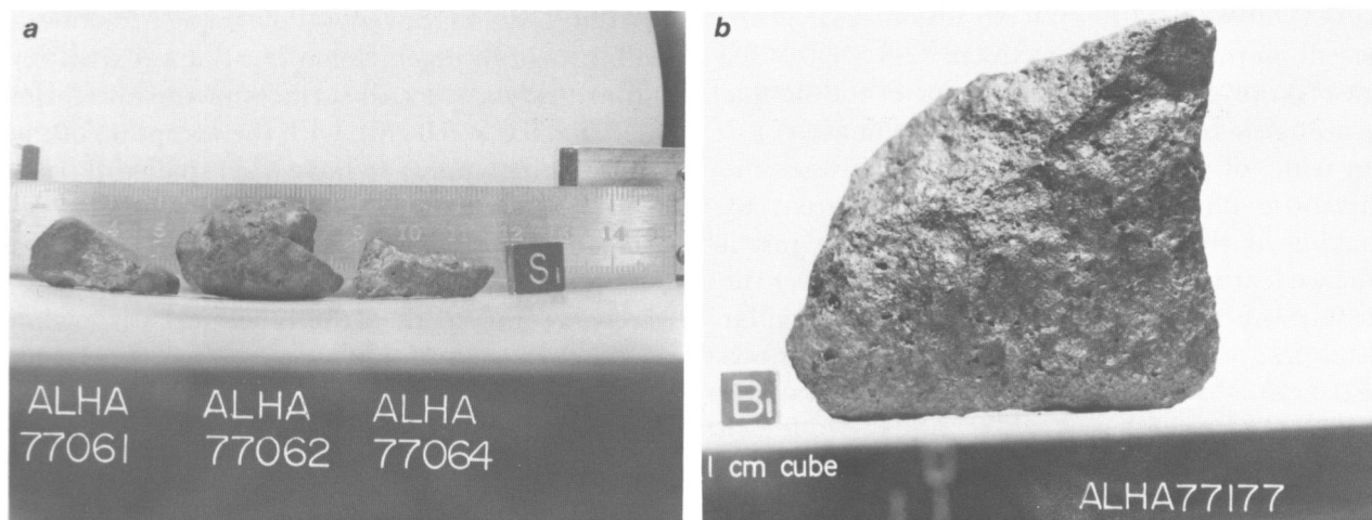
FIGURE 23.—H5 chondrites: a , ALHA77061, 77062, 77064; pebble-sized chondrites. b , ALHA77177, an angular stone with a pitted surface, probably produced by the weathering out of chondrules and lithic clasts.
