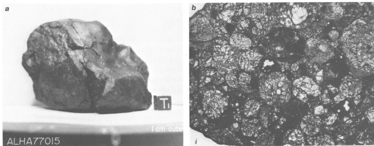
FIGURE 11.—L3 chondrites: a , ALHA77015, part on the right is coated with fusion crust; the part on the left is a fracture surface. b , ALHA77033, photomicrograph of thin section (width of field is 2.0 mm); a close-packed aggregate of chondrules characteristic of type 3 chondrites.
