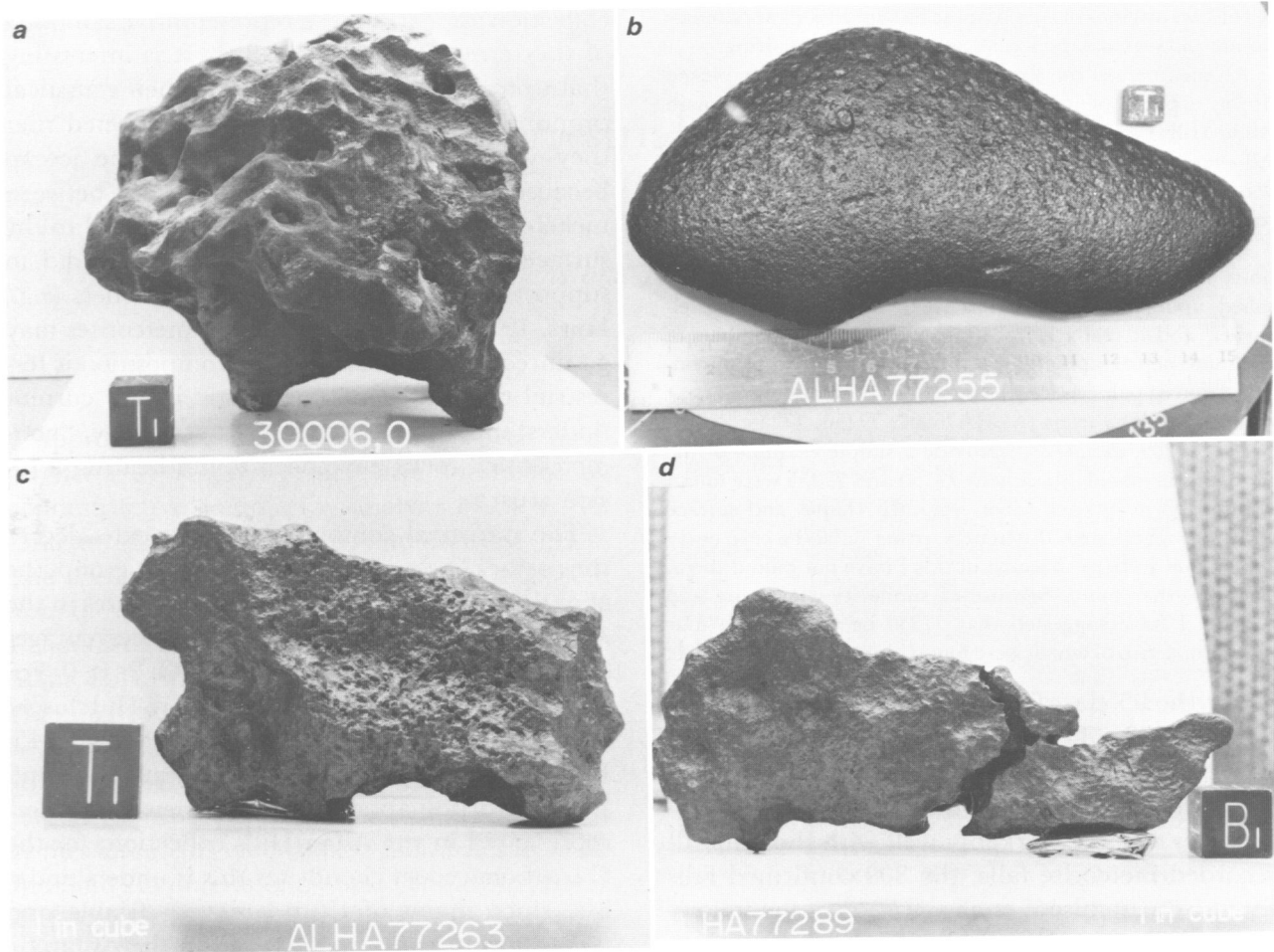
FIGURE 37.—Irons: a , PGPA77006, Purgatory Peak (width of specimen is 19 cm); the bright areas at the upper right are the sand-abraded surfaces; the lighter colored area on the lower left is the originally buried portion of the meteorite. b , ALHA77255, thin rounded specimen with small regmaglypts on the surface. c , ALHA77263, an irregular angular meteorite with a pitted surface (the surface illustrated was in contact with the ice at the time of collection). d , ALHA77289, an angular elongated meteorite with a deep fissure, probably a zone of preferential melting and ablation.
