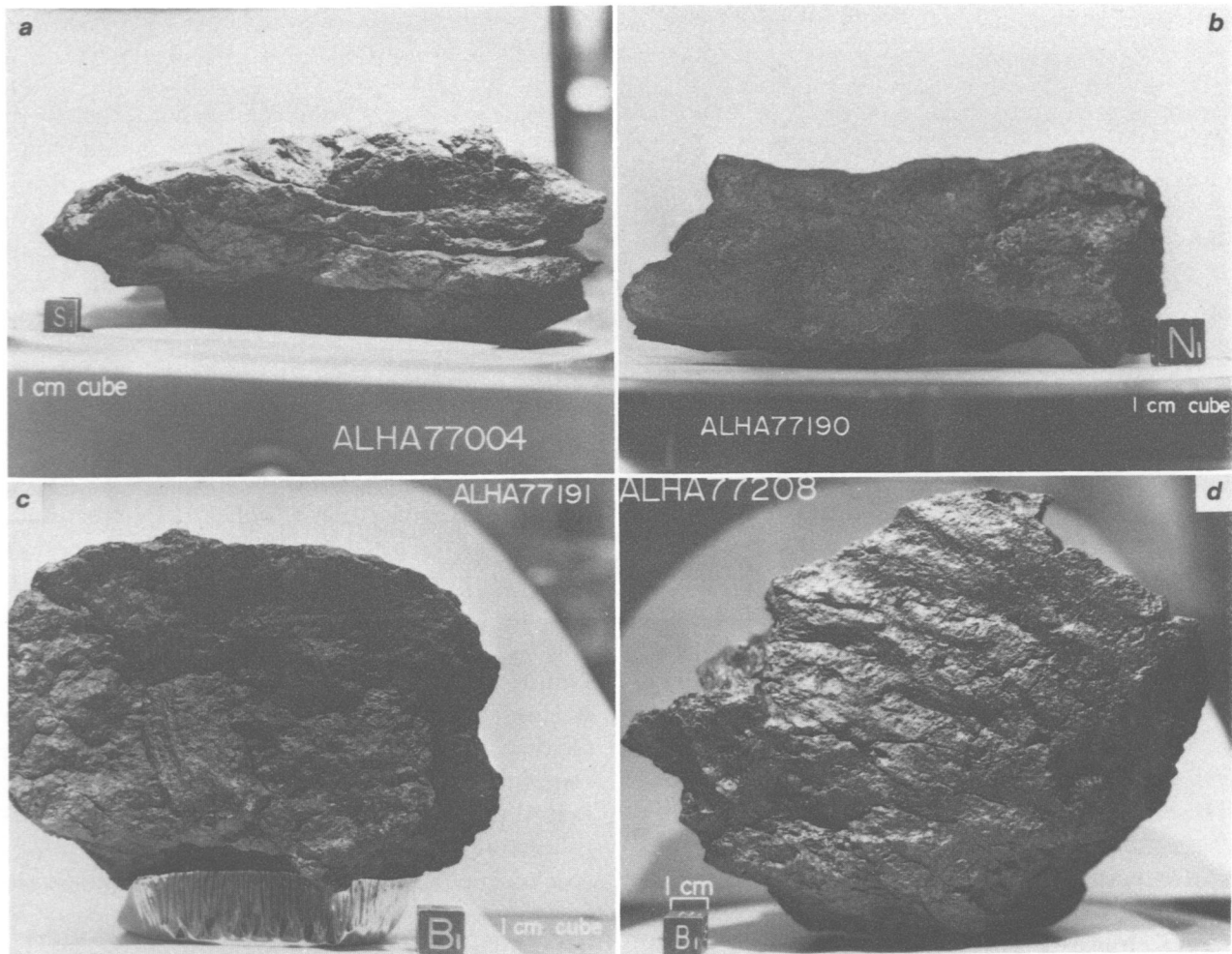
FIGURE 18.—H4 chondrites: a , ALHA77004, severely weathered stone with deep parallel fractures. b , ALHA77190, a tabular specimen with patchy remnants of dull black fusion crust. c , ALHA77191, the area photographed is a concave fracture surface, stained red-brown with iron oxides produced by weathering. d , ALHA77208, a severely weathered and deeply fractured stone, without fusion crust.
