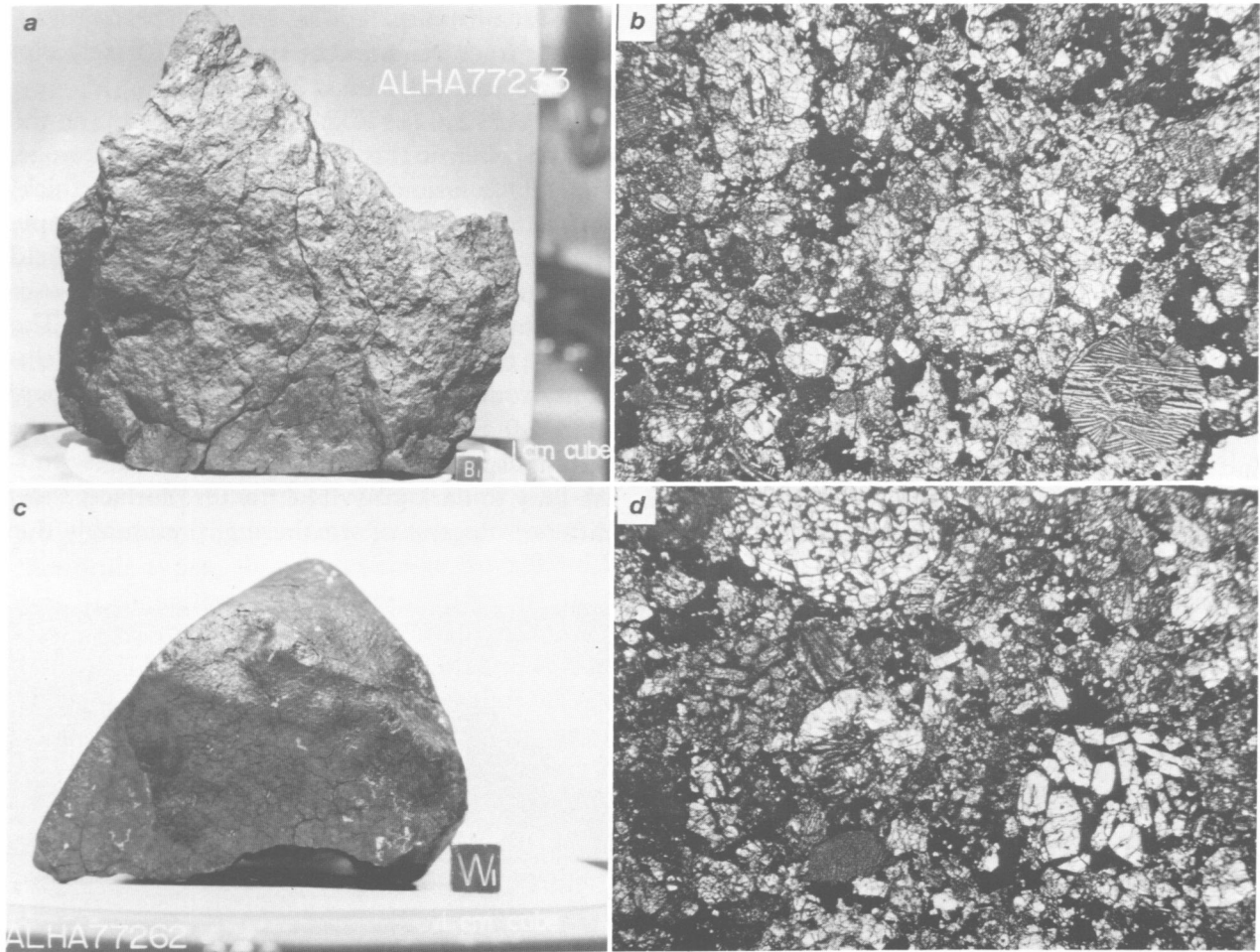
FIGURE 19.—H4 chondrites: a , ALHA77233, severely weathered and moderately fractured stone; b , photomicrograph of thin section (width of field is 2.0 mm), showing well-developed chondrules in a granular matrix. c , ALHA77262, angular, roughly conical stone covered with fusion crust except on the base; d , photomicrograph of thin section (width of field is 2.0 mm), showing large porphyritic and granular olivine chondrules.
