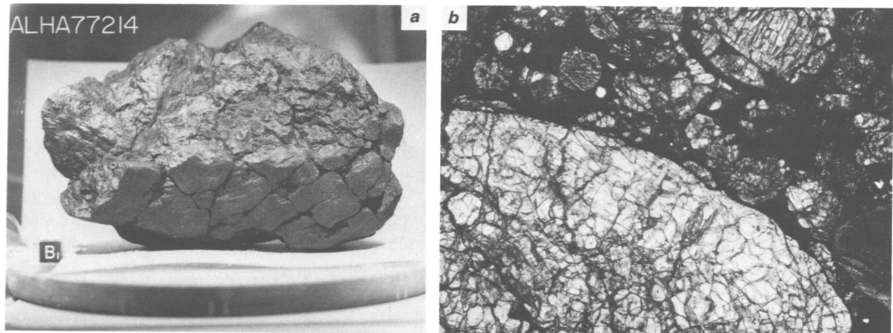
FIGURE 14.—ALHA77214, L3 chondrite: a , Note well-developed fissuring and remnants of original surface on lower part. b , Photomicrograph of thin section (width of field is 2.0 mm), showing part of elliptical granular inclusion (p. 20).
