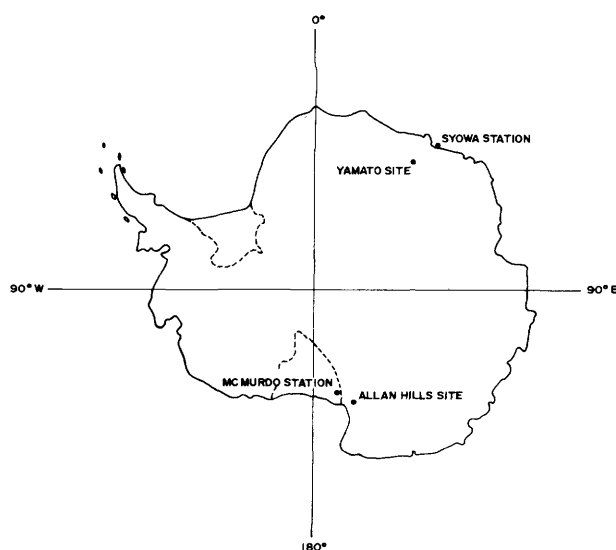
FIGURE 3.—Map of Antarctica, indicating the Yamato and the Allan Hills sites.
