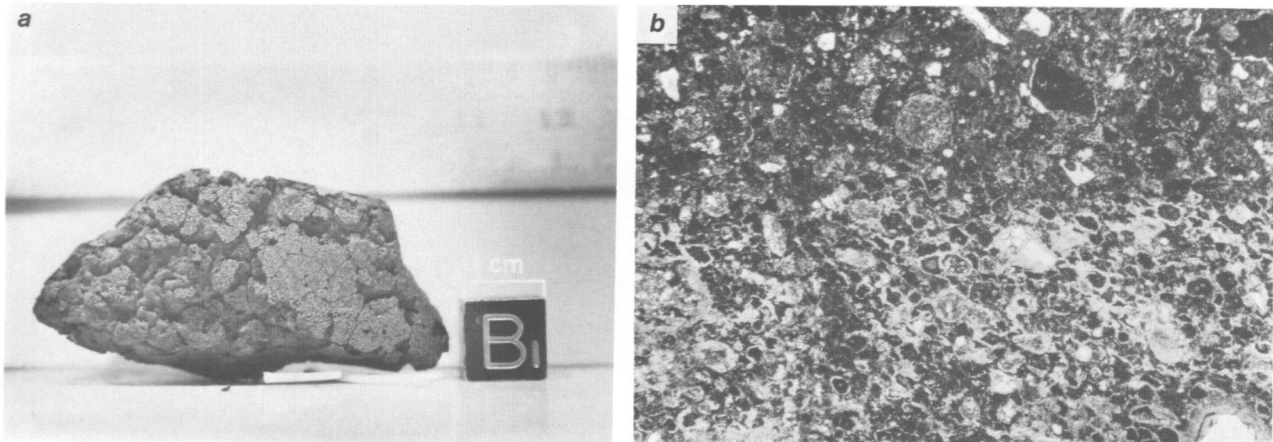
FIGURE 8.—ALHA 77306, C2 chondrite: a , A partial coating of fusion crust (lighter gray) is present. b , Photomicrograph of thin section (width of field is 2.0 mm); irregular grains and rare chondrules, mainly of olivine (white to light gray) in opaque to translucent matrix (dark gray to black).
