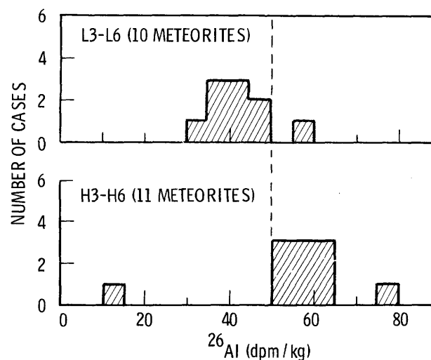
FIGURE 39.— ^{26}\text{Al} content of Allan Hills chondrites by class normalized to L-type composition.
