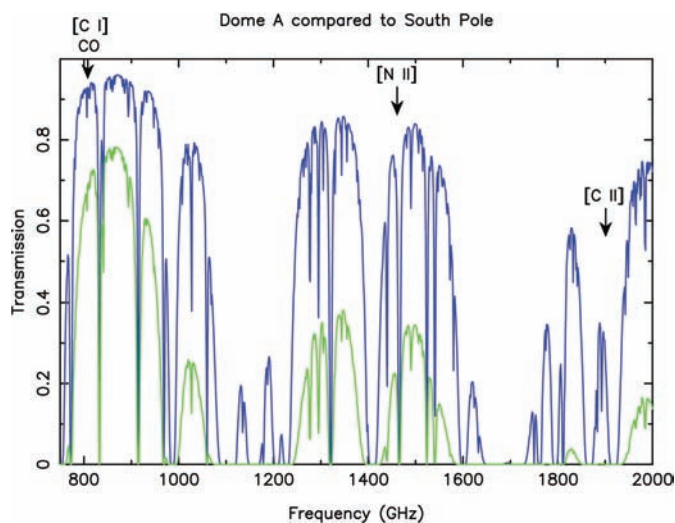
FIGURE 5. Terahertz atmospheric transmission for good (twenty-fifth percentile) winter conditions for the South Pole (bottom line) and Dome A (top line), derived from PWV measurements at the South Pole, atmospheric models from Lawrence (2004), and actual automatic weather station data collected during 2005 from Dome A. The PWV content for each model atmosphere is 210 and 50 micrometers, respectively. Arrows indicate the wavelengths of the [N II], [C II], and CO/[C I] lines.
