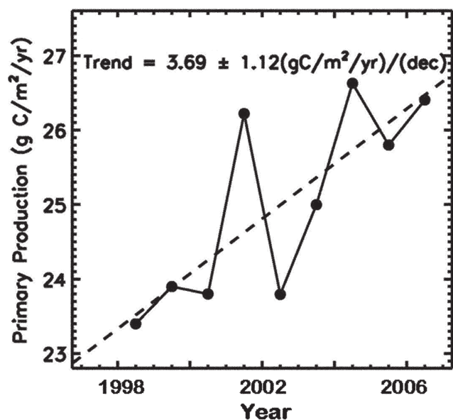
FIGURE 5. The temporal pattern of productivity for the entire Southern Ocean as derived from satellite data and a productivity model (from Smith and Comiso, 2008). The trend is derived from a linear regression of all points and is highly significant.
