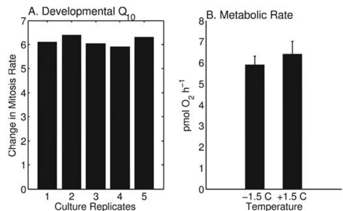
FIGURE 1. Temperature Q 10 for developmental rates and energy utilization in the Antarctic sea urchin Sterechinus neumayeri . (A) Embryogenesis at +1.5^{\circ}\text{C} was much faster than at -1.5^{\circ}\text{C} and was equivalent to a 6-fold rate change per 10^{\circ}\text{C} (i.e., Q10 estimate). (B) The metabolic rates of hatching blastulae at these two temperatures did not reveal any impact of temperature (i.e., Q10 \sim 0 ).
