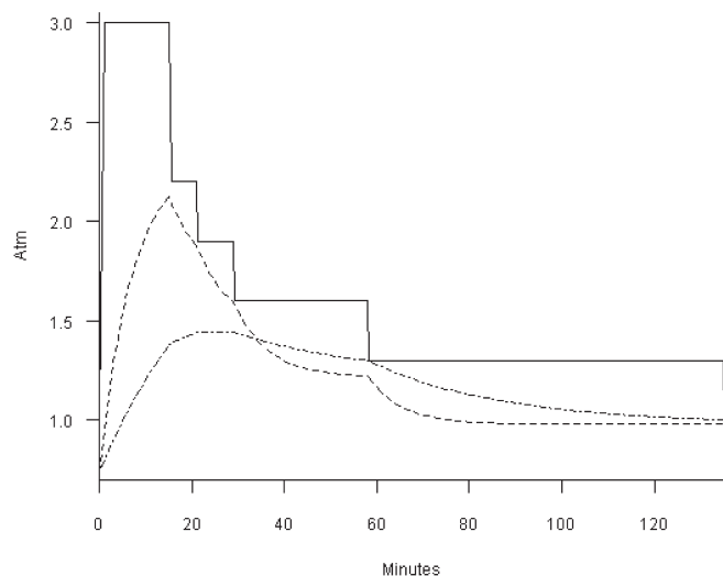
FIGURE 1. Ambient pressure (solid line) versus time and the corresponding total gas pressures ( \Sigma P_{tis.inert} ) in two compartments (half-times of 5 and 20 minutes) for an air breathing dive. Classical decompression is scheduled to keep dissolved gas pressure in k modeled compartments less than or equal to a maximum permissible value, P_{tis.maxk} \leq a_k P_{amb} + b_k . For simplicity, the above figure shows only two compartments and sets a = 1 and b = 0 , so that the ‘safe ascent depth’, P_{amb.min} = \max((P_{risk} - b)/a) , is equal to \max(P_{risk}) . In Haldane and colleagues algorithm, compartment half times were 5, 10, 20, 40, and 75. The Haldane “2:1 tissue ratio” arises from treating air as an inert gas and setting the safe ascent depth as P_{amb} = \max(P_{risk}/2) . By convention, decompression stops are taken at increments of 10 fsw (0.3 atm abs) deeper than sea level.
