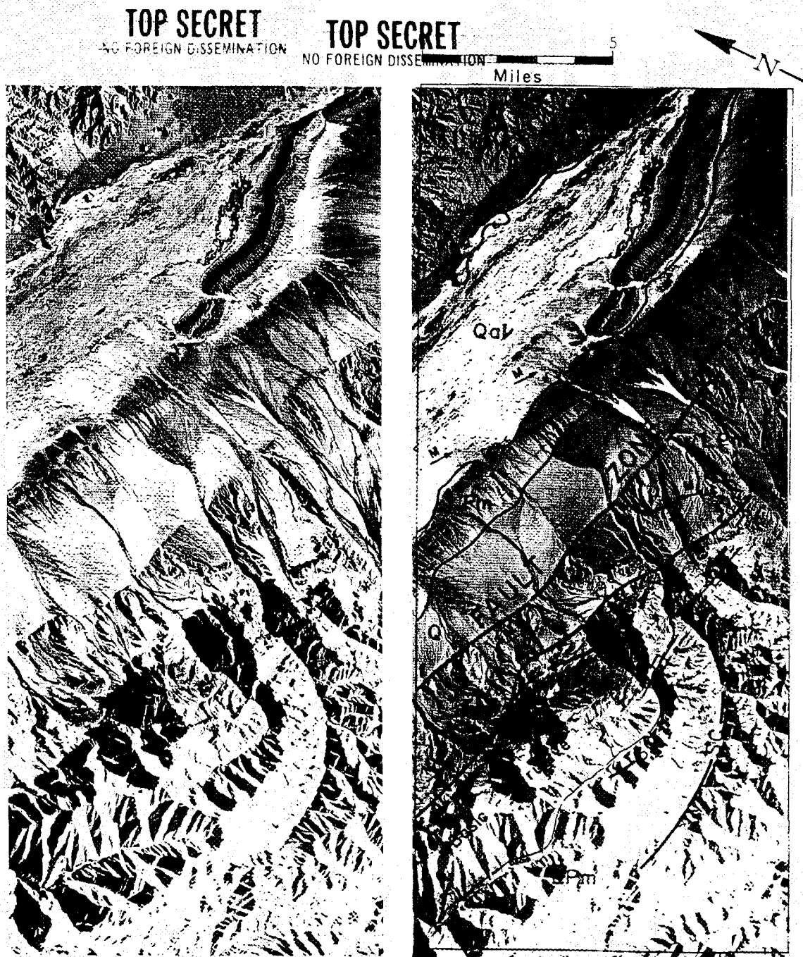
Fig. 5-4 — 3404 and SO-242 records showing apparent mineralization (red stains) in vicinity of igneous intrusion
