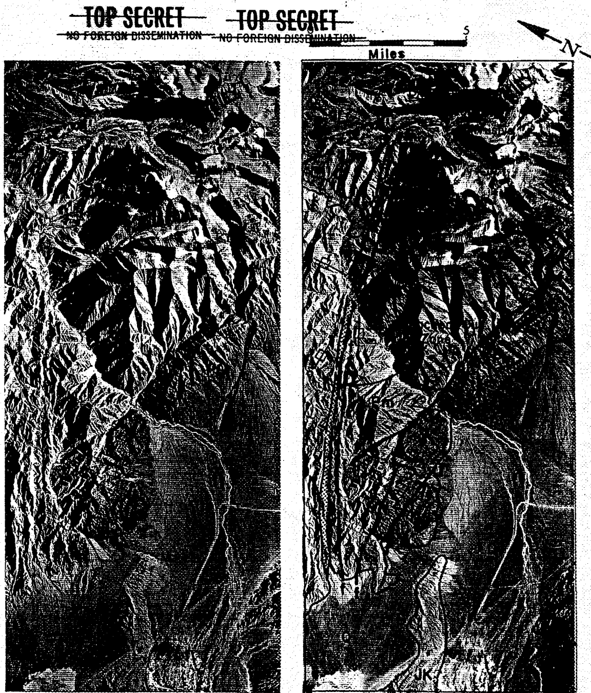
Fig. 5-3 — 3404 and SO-242 records showing possible mineralized zone along fault or dike
