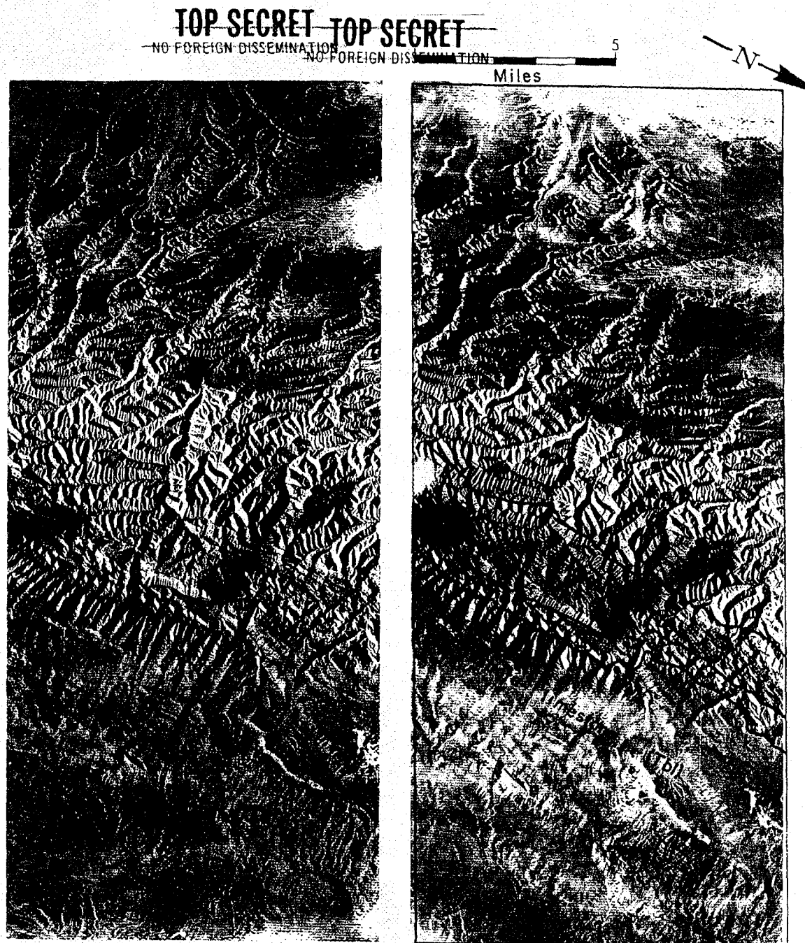
Fig. 6-2 — 3404 and SO-242 records showing typical sedimentary section, Kafirnigan—Pyandzh area
