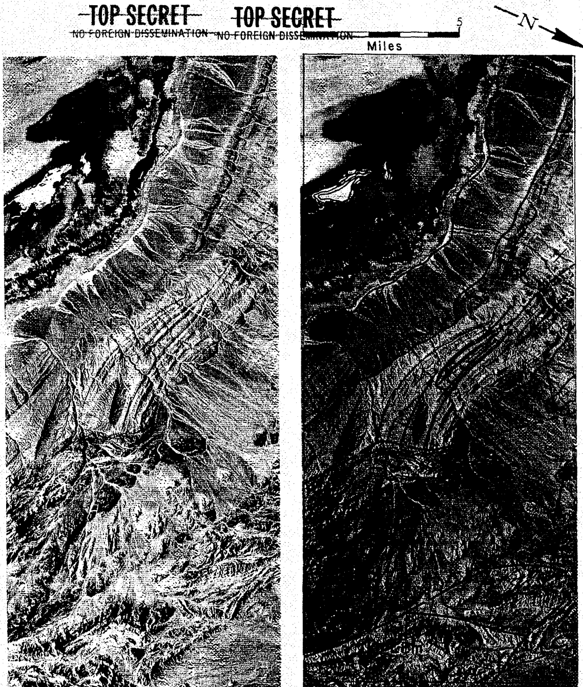
Fig. 5-2 — 3404 and SO-242 records showing contact zone and tight fold structures in Jurassic-Cretaceous
