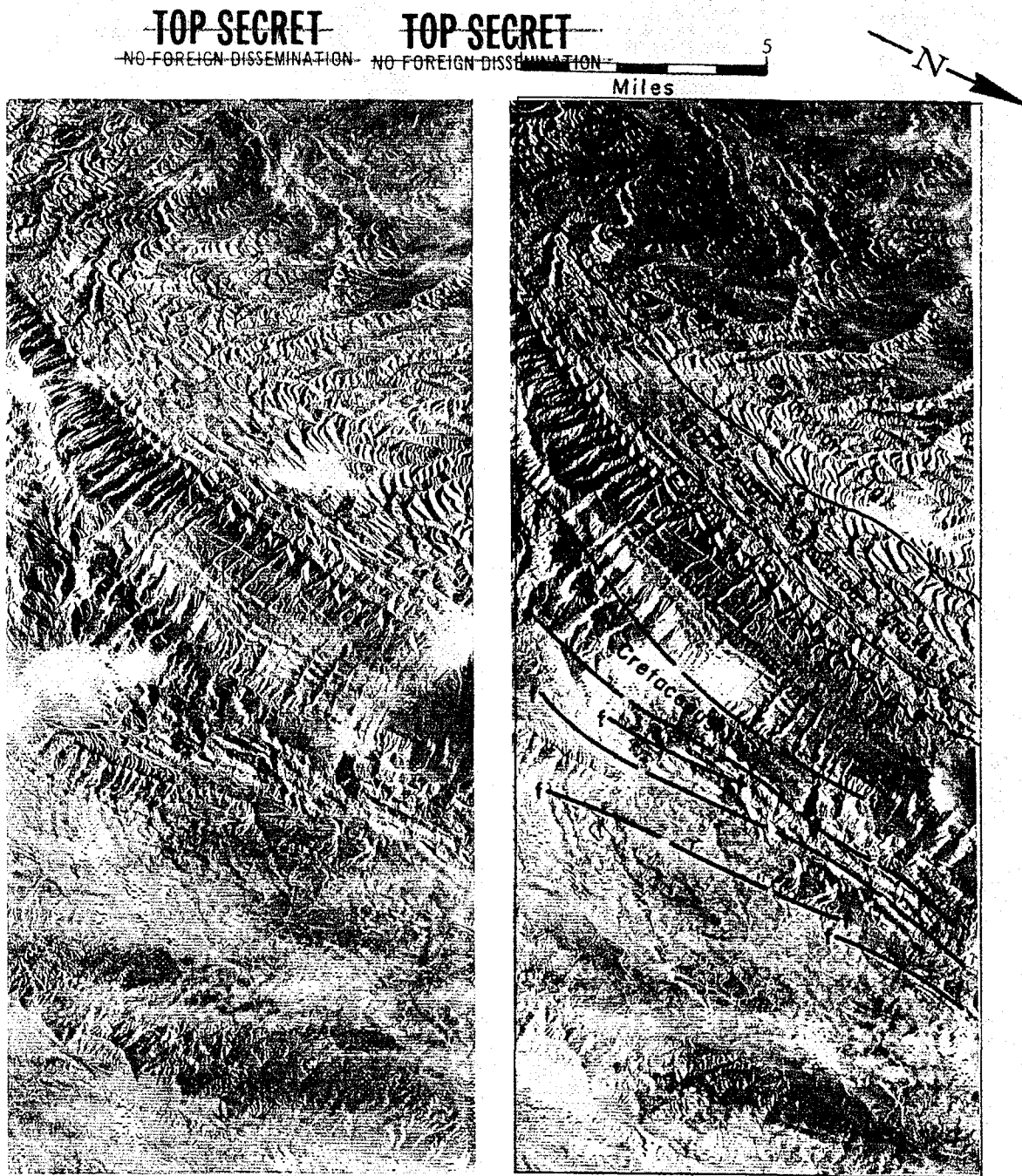
Fig. 6-3 — 3404 and SO-242 records showing sedimentary section, Kafirnigan—Pyandzh area
