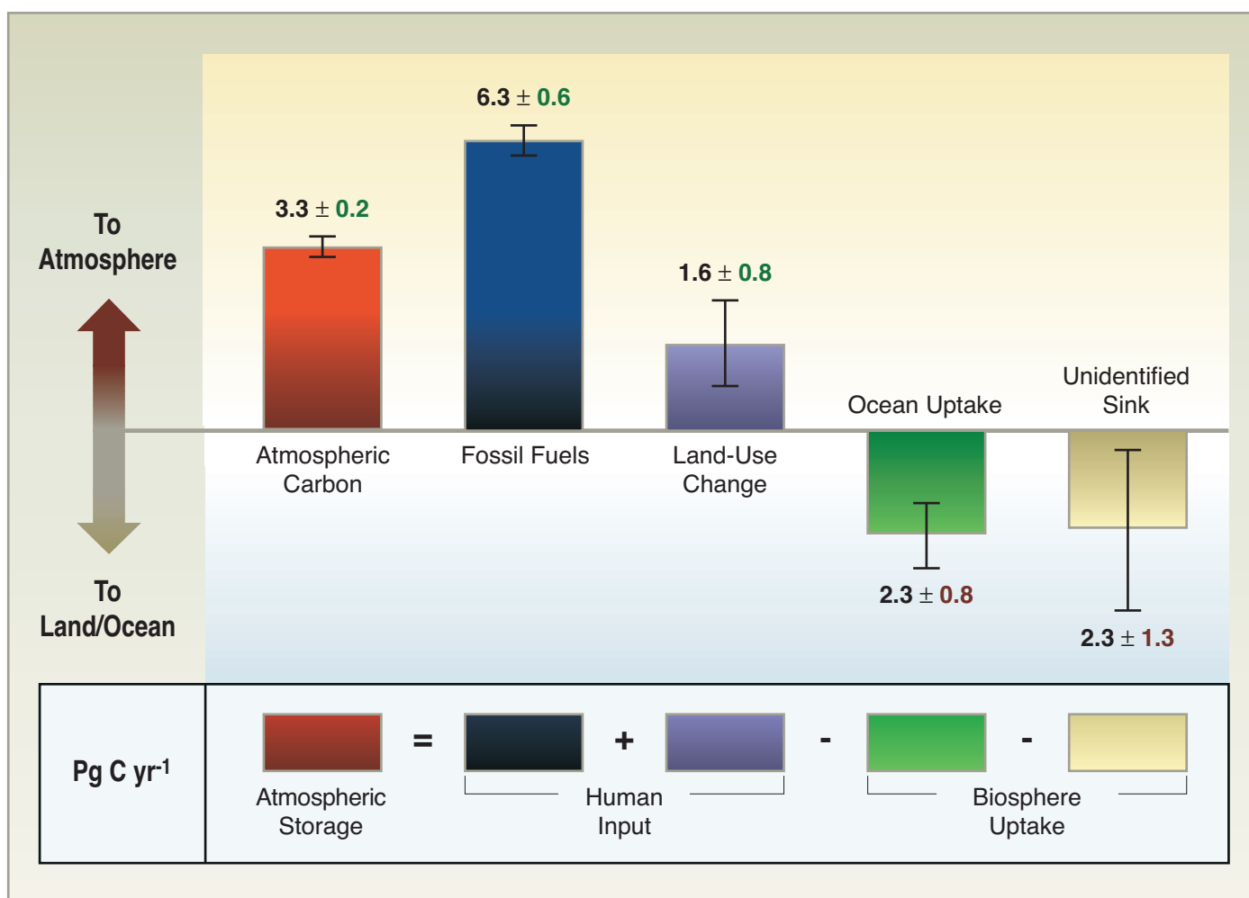
Figure 7-2: Average annual global budget of \text{CO}_2 and uncertainties for 1989 to 1998 expressed in \text{PgC yr}^{-1} . Error bounds correspond to a 90% confidence interval. The numbers reported here are from Land Use, Land-Use Change, and Forestry , a special report of the Intergovernmental Panel on Climate Change (IPCC, 2000a). There is compelling evidence that a large fraction of the “unidentified sink” may be accounted for by uptake in the temperate and/or boreal zones of the terrestrial Northern Hemisphere. Source: F. Hall, Office of Global Carbon Studies, NASA Goddard Space Flight Center.
