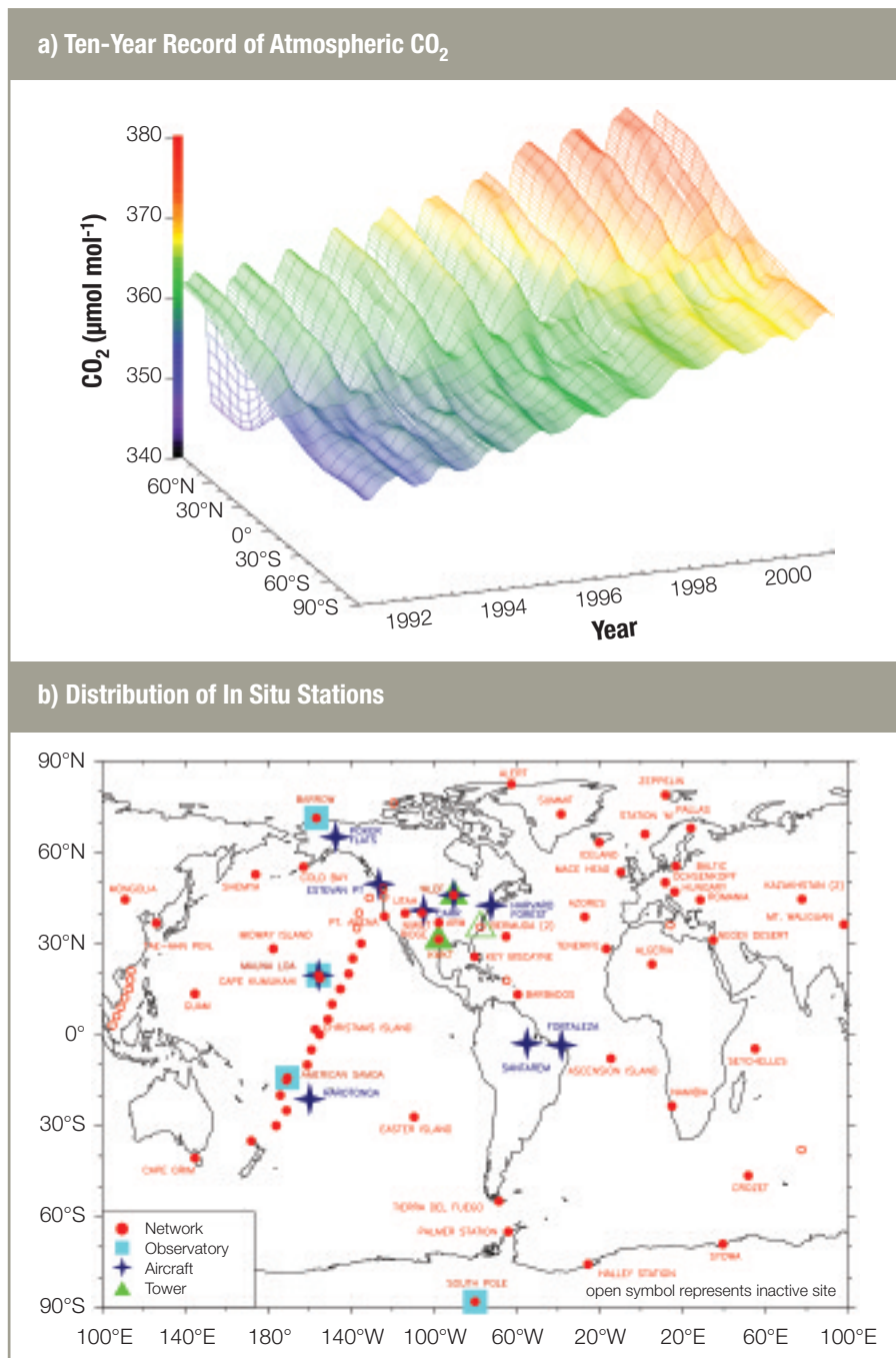
Figure 12-1: (a) Ten-year record of atmospheric carbon dioxide (CO 2 ) at a variety of stations as a function of latitude, and (b) distribution of in situ stations collecting data on CO 2 and other greenhouse gases. Source: Pieter Tans, NOAA CMDL. For more information, see Annex C.
