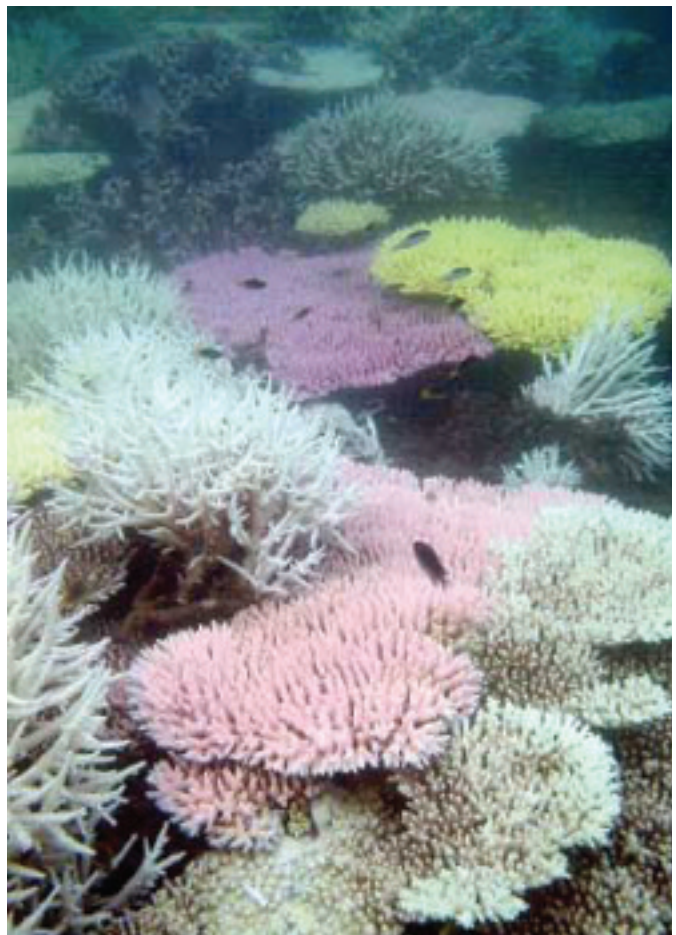
Figure 8-3: When stressed, corals frequently expel their symbiotic algae en masse, leaving coral bereft of pigmentation and appearing nearly transparent on the animal's white skeleton, a phenomenon referred to as coral bleaching. This image of bleached coral colonies was obtained during the January-March 2002 coral bleaching event in Great Barrier Reef, Australia, the worst bleaching event on record for this reef. Bleaching events reported prior to the 1980s were generally attributed to local phenomena (e.g., major storm events, sedimentation, or pollution); but, since then, a direct relationship between bleaching events and elevated ocean temperature (see Figure 8-4) was found. Source: Ray Berkelmans, Australian Institute of Marine Science.
