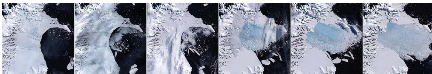
A series of satellite images of the Antarctic Peninsula record the catastrophic breakup of a massive portion of the Larsen B Ice Shelf—an area larger than the state of Rhode Island—in 2002. The first scene, from January 31, 2002, shows the shelf in late austral summer, with dark bluish melt ponds dotting its surface. In the next two scenes, minor retreat takes place, amounting to about 800 square kilometers (300 square miles), during which several of the melt ponds well away from the ice-front drain through new cracks in the shelf. The main collapse is seen in the last two scenes, on March 7 and 17th, with thousands of sliver icebergs and a large area of very finely divided icebergs where the shelf formerly lay. Brownish streaks within the floating chunks mark areas where rocks and morainal debris are exposed from the former underside and interior of the shelf. The last phases of the retreat totaled about 2,600 square kilometers (1,000 square miles). Credit: MODIS images from NASA's Terra satellite supplied by Dr. Ted Scambos; National Snow and Ice Data Center, University of Colorado, Boulder
