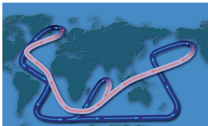
The global ocean circulation system, often called the "ocean conveyor," transports heat throughout the planet. Light sections represent warm surface currents. Dark sections represent deep, cold currents. Credit: Illustration by Jayne Doucette, Woods Hole Oceanographic Institution
