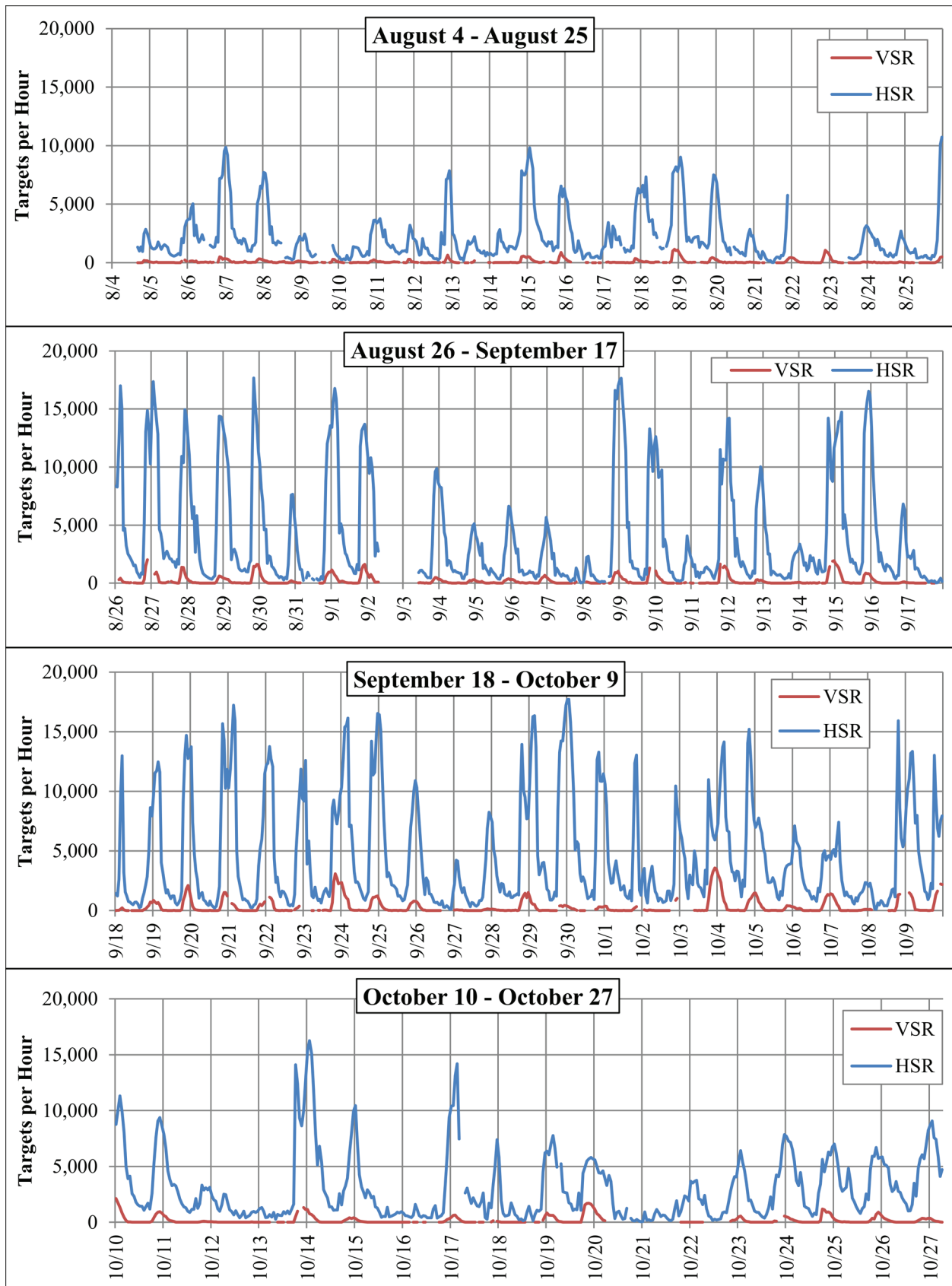
Figure 17. Hourly target counts in Jefferson County by horizontal and vertical radars from August 4 – October 27, 2016 Jefferson County. Vertical lines represent midnight.
