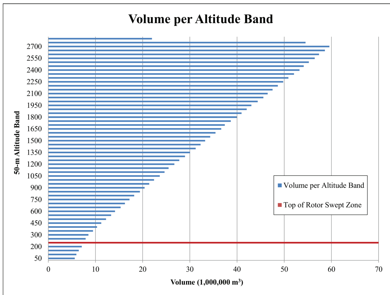
Figure 7. Volume of 50 m altitude bands within the standard front. Volumes were estimated with Monte Carlo integration. Altitude band intervals represent the upper band limit. Target counts provided by the vertical scanning radar are limited to the structure of the standard front. The red line represents the top of the rotor swept zone at 200 m.
