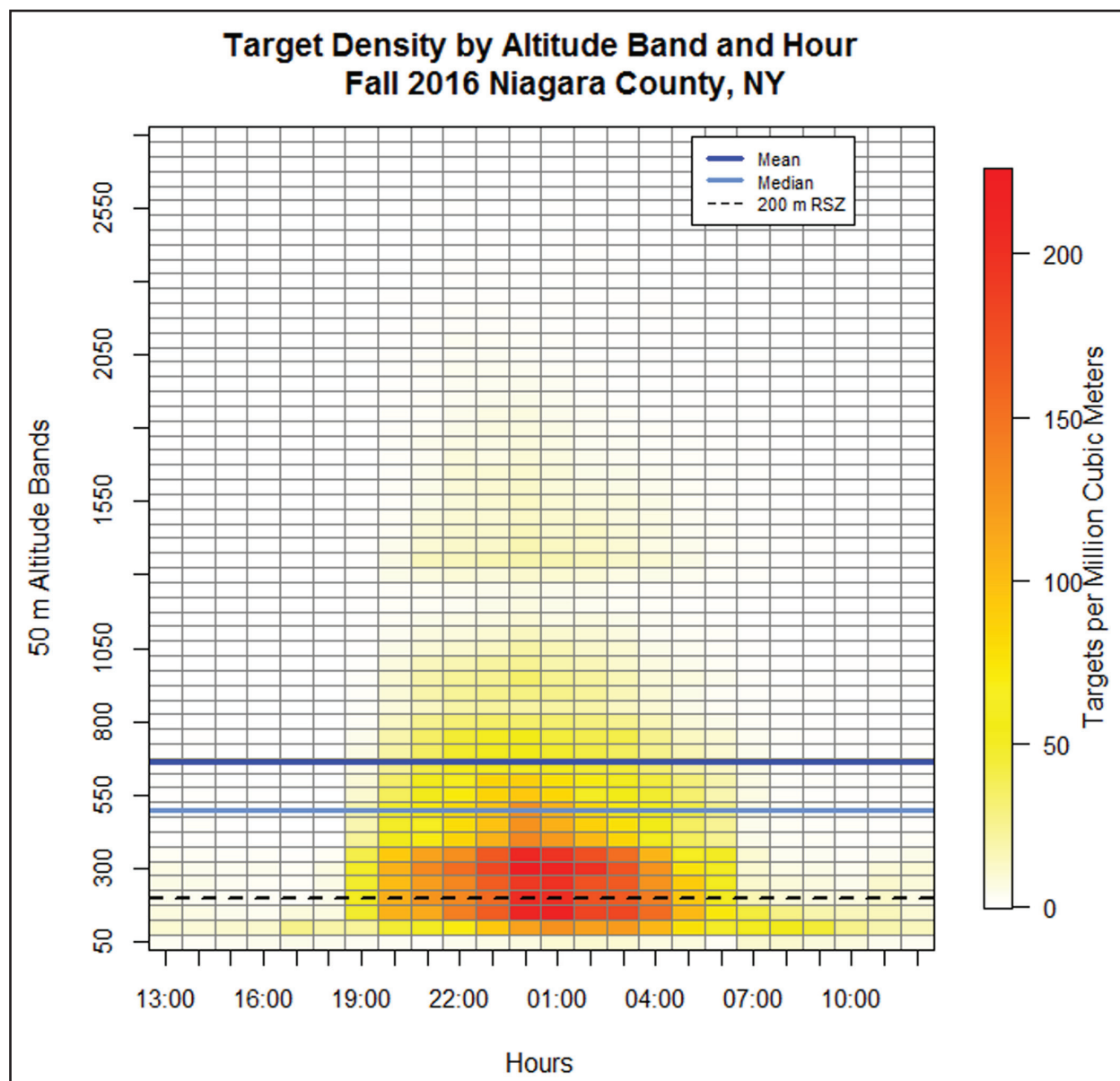
Figure 36. Heatmap for Niagara County, representing variation in flight altitudes based on target density (targets per million cubic m). Altitude bands are in meters and labels represent the max value of each altitude band. Density of targets is in targets per million cubic meters. Colors shown in each rectangle indicate the relative density observed for that altitude (key shown on the right) and time. The dark blue and light blue lines represent the nocturnal mean and median target heights, respectively. The black line at 200 m represents the max height of a turbine with a RSZ of 30 – 200 m. Note the difference in density scale used in Figures 34 and 35.
