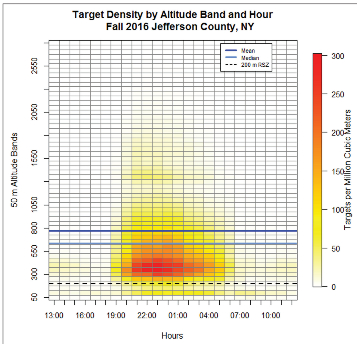
Figure 34. Heatmap for Jefferson County, representing variation in flight altitudes based on target density (targets per million cubic m). Altitude bands are in meters and labels represent the max value of each altitude band. Density of targets is in targets per million cubic meters. Colors shown in each rectangle indicate the relative density observed for that altitude (key shown on the right) and time. The dark blue and light blue lines represent the nocturnal mean and median target heights, respectively. The black line at 200 m represents the max height of a turbine with a RSZ of 30 – 200 m. Note the difference in density scale used in Figures 35 and 36. Some of the lack of low-altitude activity at this site may be attributable to relatively high clutter on the vertical antenna, which can be seen as white areas on the clutter map in Figure 4.
