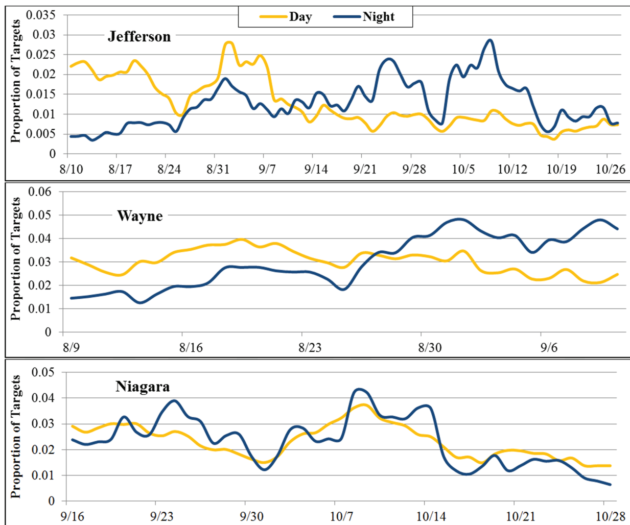
Figure 24. Proportional diurnal and nocturnal seven-day moving means at Jefferson (top), Wayne (middle), and Niagara (bottom) sites, New York during fall 2016. Proportions (single day or night target count divided by the sum of day or night target counts for the entire season) are used rather than TPR to account for the large difference between nocturnal and diurnal flight intensity, allowing comparisons between daytime and nighttime relative activity levels over the course of the season.
