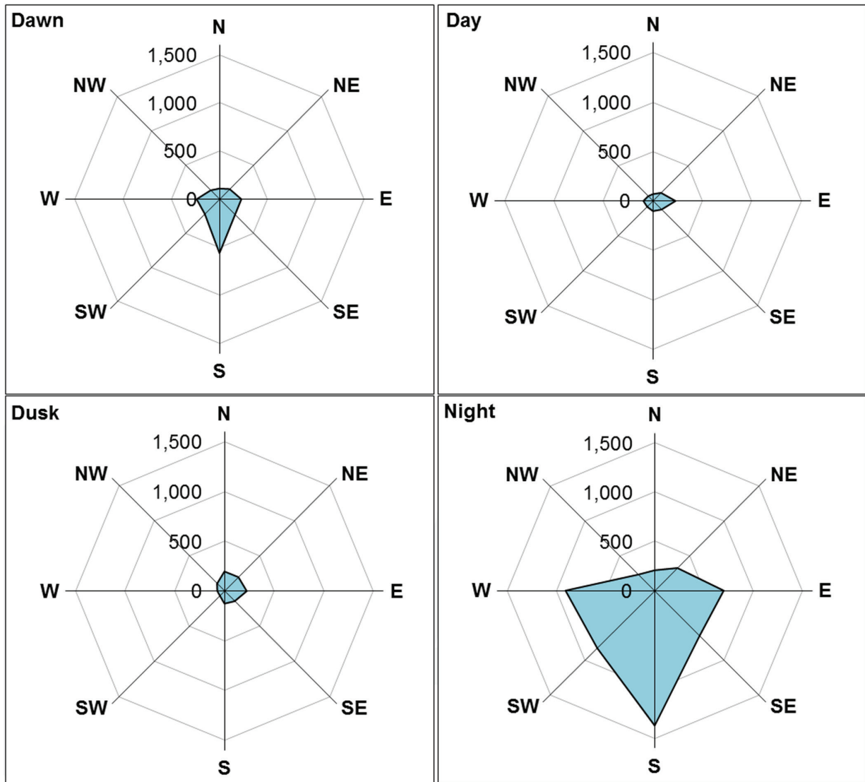
Figure 12. Direction of targets during Dawn, Day, Dusk, and Night at the Wayne County site. Each point on the perimeter of the rose graph indicates the average number of targets per hour moving in each of the eight directions. Axis scale is fixed, so the area of polygons also represents the relative amount of target activity during that period.
