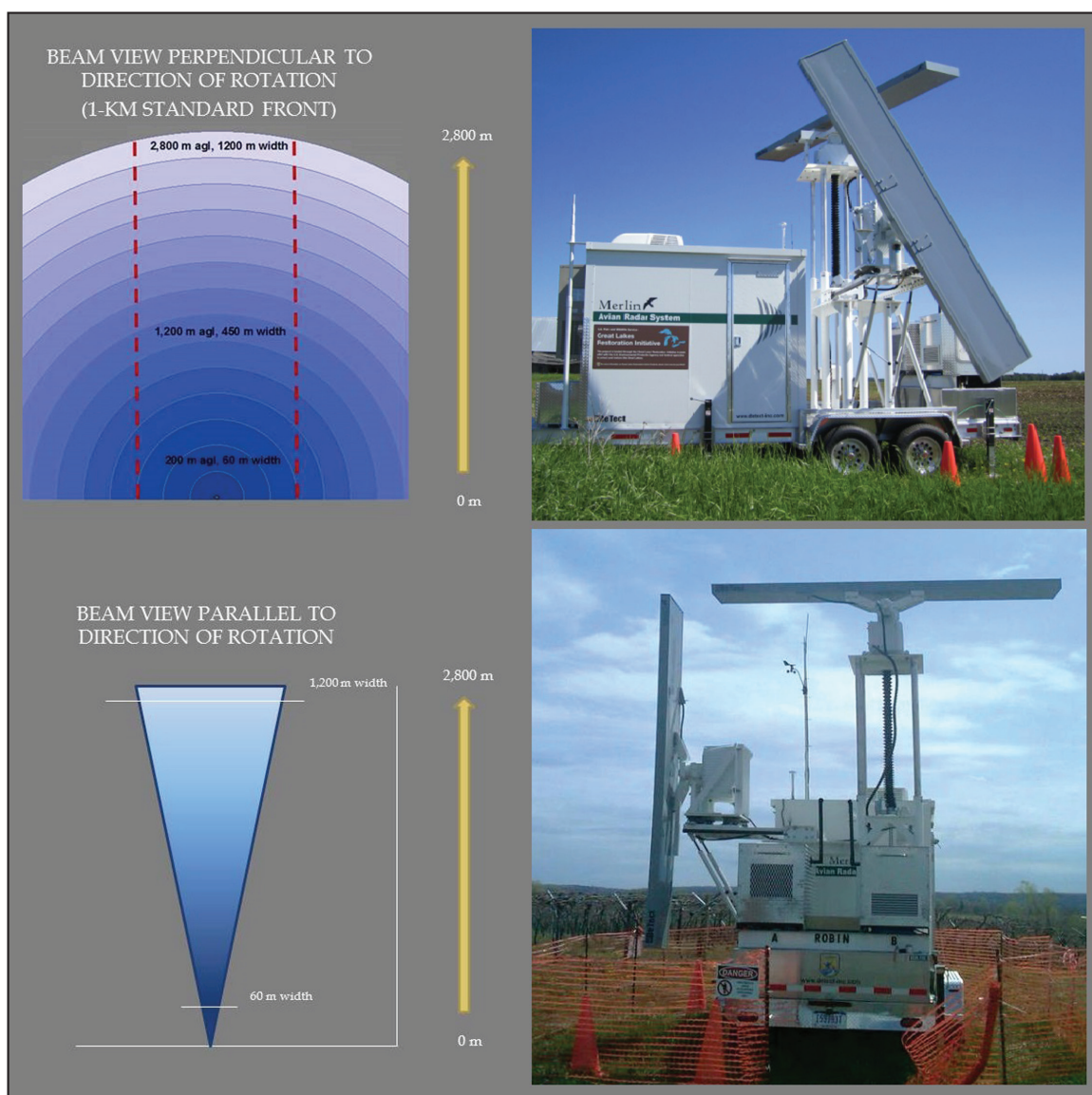
Figure 5. Schematic of vertical scanning radar beam. Graphical representations (left) pair with photos (right) of the radar unit aligned perpendicular (top) and parallel (bottom) to rotational plane. The standard front used for data analysis is marked on the top left image. The standard front extends to 500 m on either side of the radar and up to a height of 2800 m. In this graphic the radar is situated at the bottom center and the red dashed lines represent the lateral limits of the standard front. In the bottom graphic the radar rotation is suspended so that the beam emits directly upward; this view is an approximation of the beam dispersion as it travels away from the radar unit (schematic not drawn to scale).
