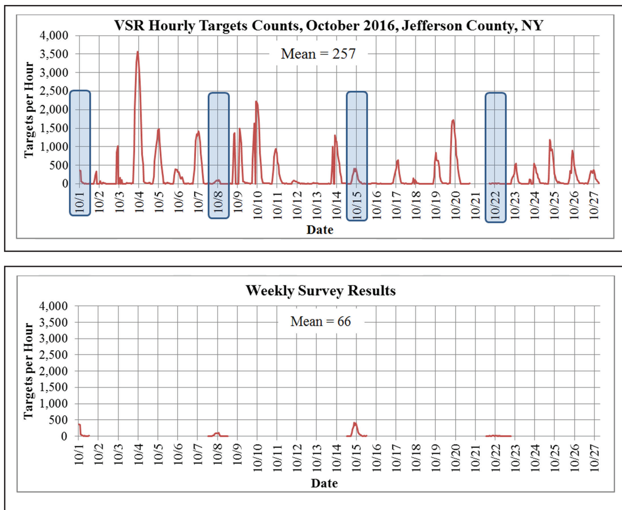
Figure 38. Results of hypothetical non-continuous sampling schedule where data were collected on a continuous sampling schedule (top graphic) versus a weekly sampling schedule (bottom graphic). Red lines represent the number of targets counted per hour by the vertical scanning radar in October 2016 in Jefferson County, New York.
