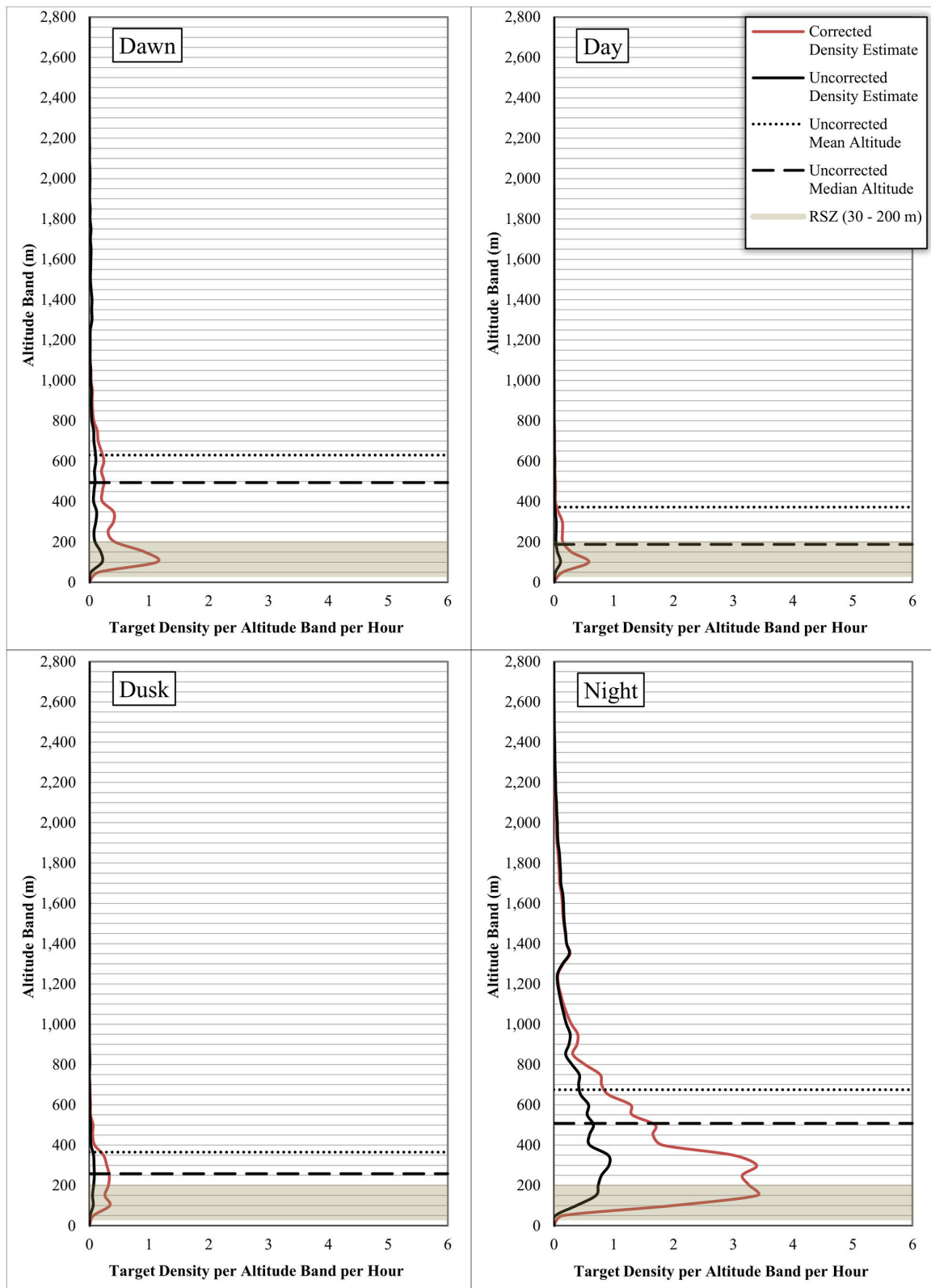
Figure 27. Altitude profile of targets at Niagara County. Corrected lines depict target density (targets/1,000,000 m 3 ) within each 50-m altitude band per hour after adjusting for the sample volume within the band. Uncorrected lines depict target density per 50-m altitude band per hour without adjusting for volume (i.e., under the assumption that each band's volume is equal to the total volume divided by the number of bands). Shaded area represents the rotor swept zone (RSZ) between 30 - 200 m. Y-axis labels represent the top of the altitude band.
