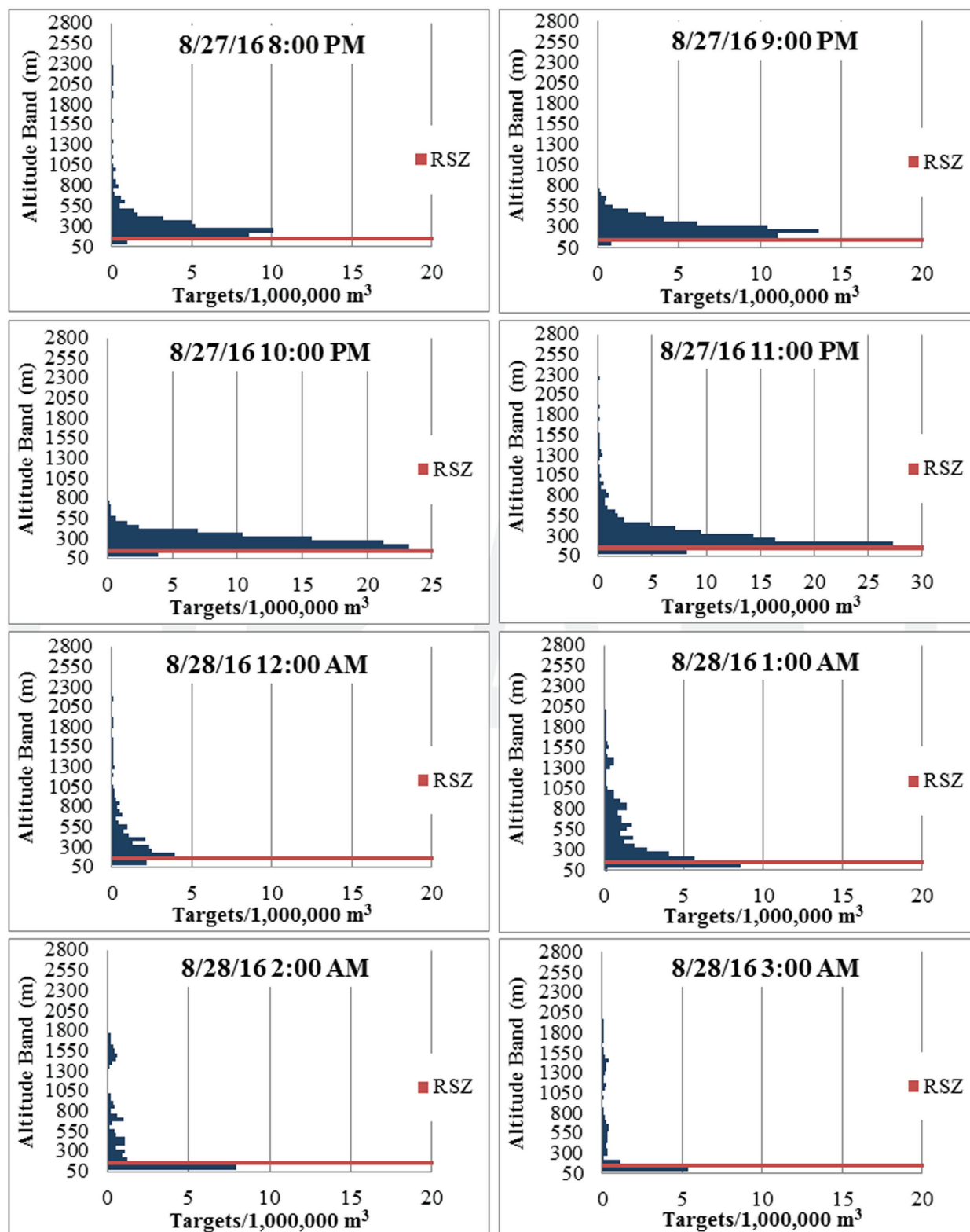
Figure 29. A sample of hourly altitude profiles in Wayne County, corrected for the shape of the sample volume From August 27 – 28, 2016. The x-axis represents target density. The red line represents the top of the rotor swept zone from 150 m to 200 m. Y-axis labels represent the top of the altitude band.
