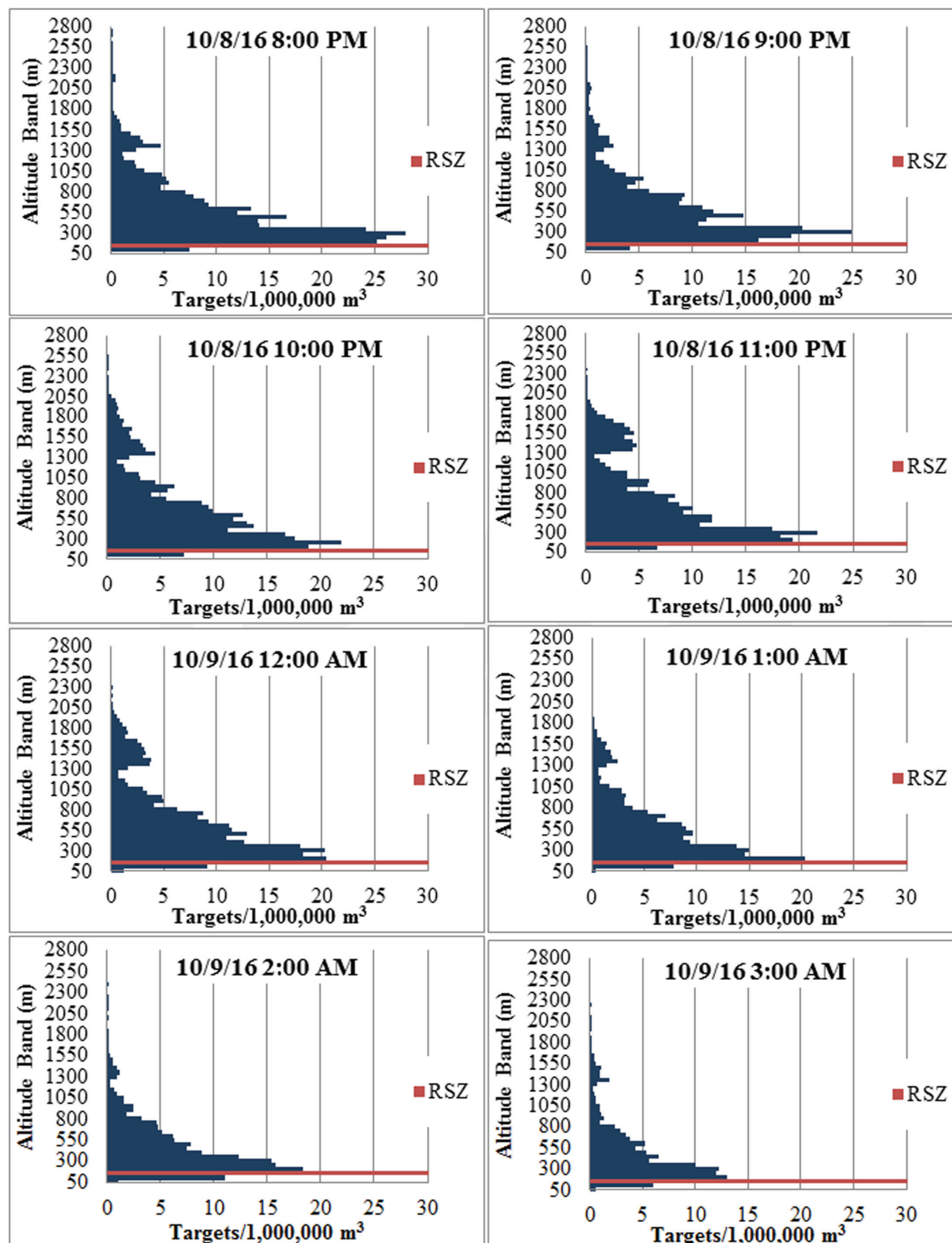
Figure 30. A sample of hourly altitude profiles in Niagara County, corrected for the shape of the sample volume on October 8 – 9, 2016. The x-axis represents target density. The red line represents the top of the rotor swept zone from 150 m to 200 m. Y-axis labels represent the top of the altitude band.
