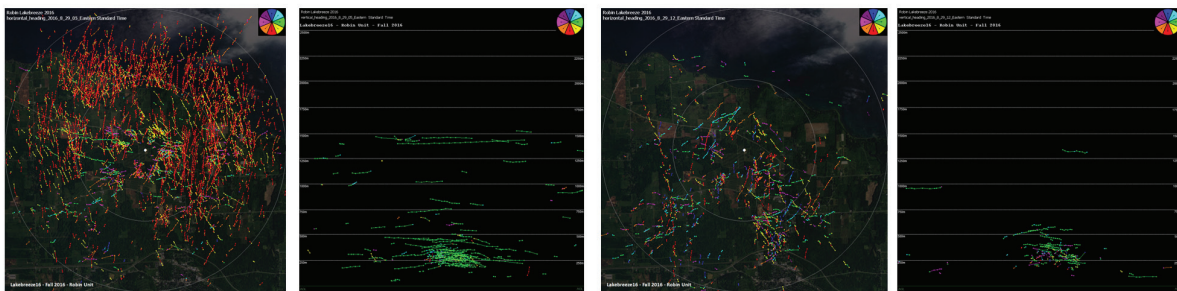
Figure 9. Sample Trackplots at WayneCounty. Flight tracks during 1 hour increments recorded by horizontal (first and third columns) and vertical (second and fourth columns) radars during a migration event at the study site in Wayne County. Colors on the horizontal radar images show direction of flights as indicated on the color wheel (dark blue indicates a direction of travel to the north and red travel to the south). Vertical radar images show target heights (colors do not indicate direction). The coastline is highlighted in white on the first horizontal image.
