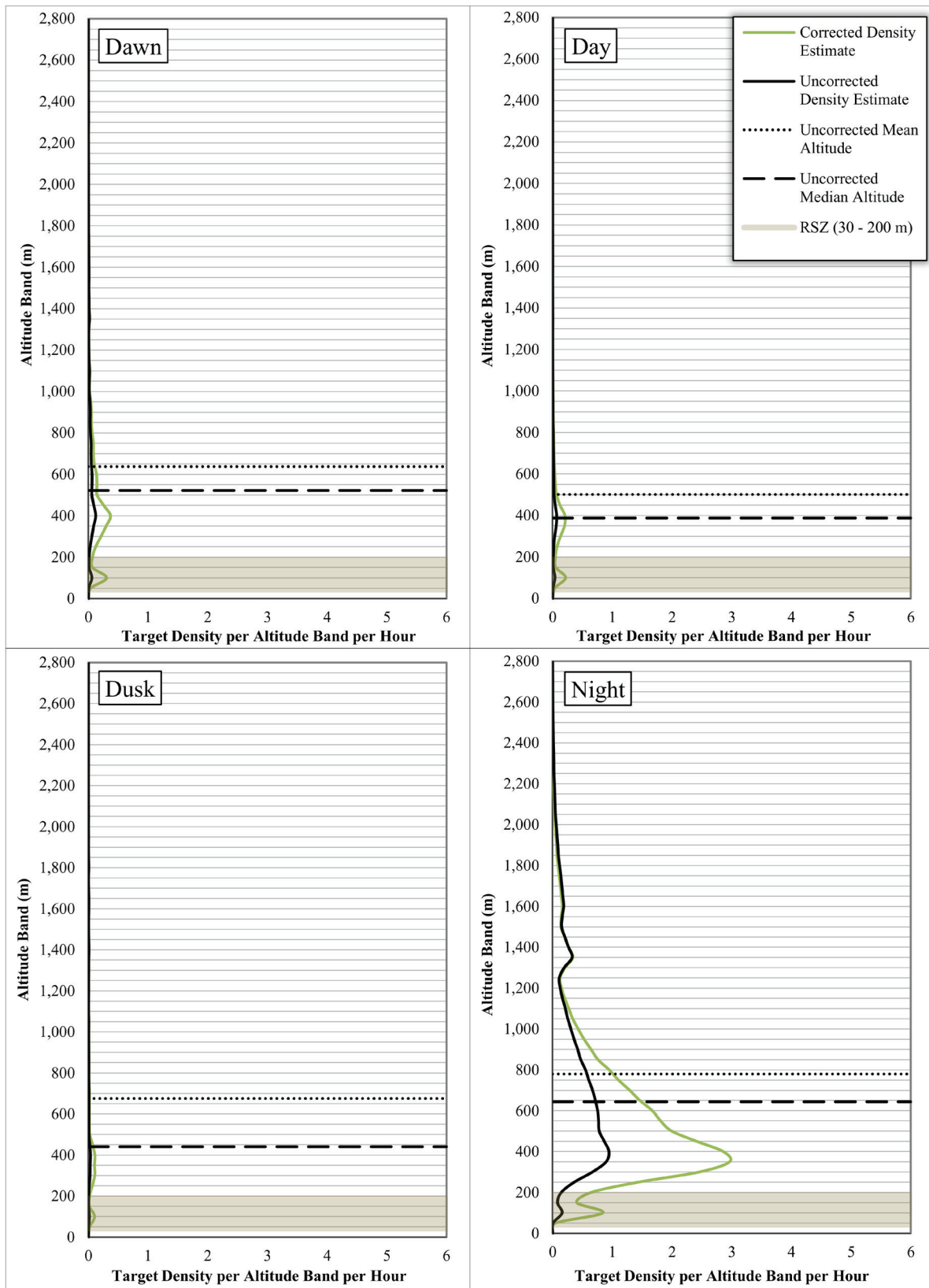
Figure 25. Altitude profile of targets at Jefferson County. Corrected lines depict target density (targets/1,000,000 m 3 ) within each 50-m altitude band per hour after adjusting for the sample volume within the band. Uncorrected lines depict target density per 50-m altitude band per hour without adjusting for volume (i.e., under the assumption that each band's volume is equal to the total volume divided by the number of bands). Shaded area represents the rotor swept zone (RSZ) between 30 - 200 m. Y-axis labels represent the top of the altitude band.
