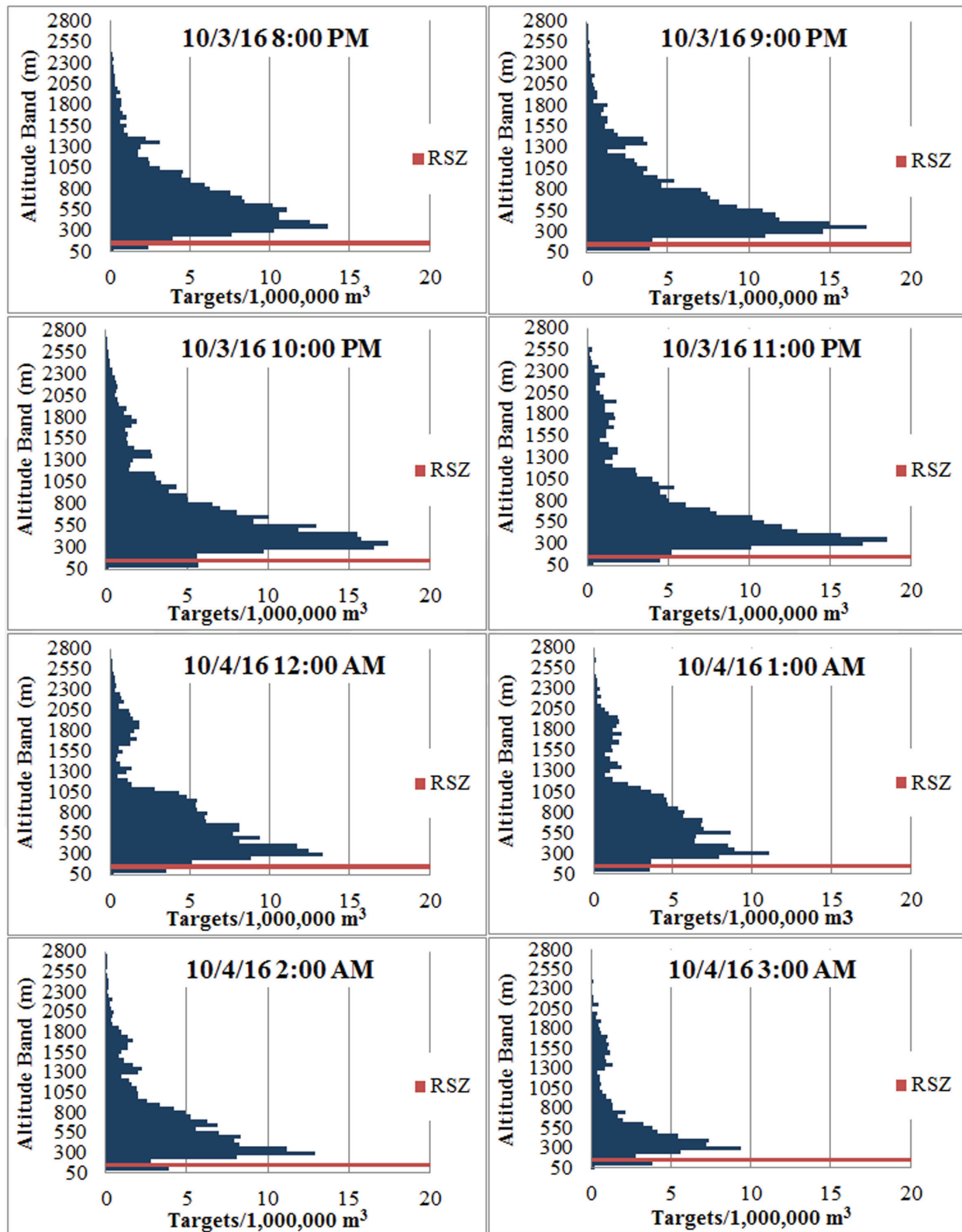
Figure 28. A sample of hourly altitude profiles in Jefferson County, corrected for the shape of the sample volume from October 3 – 4, 2016. The x-axis represents target density. The red line represents the top of the rotor swept zone from 150 m to 200 m. Y-axis labels represent the top of the altitude band.
