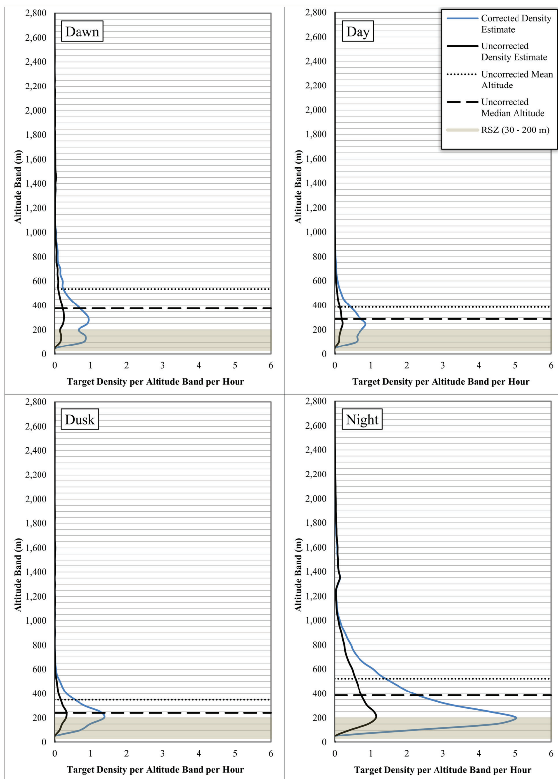
Figure 26. Altitude profile of targets at Wayne County. Corrected lines depict target density (targets/1,000,000 m 3 ) within each 50-m altitude band per hour after adjusting for the sample volume within the band. Uncorrected lines depict target density per 50-m altitude band per hour without adjusting for volume (i.e., under the assumption that each band's volume is equal to the total volume divided by the number of bands). Shaded area represents the rotor swept zone (RSZ) between 30 - 200 m. Y-axis labels represent the top of the altitude band.
