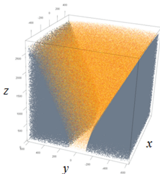
Figure 6. Sample volume estimation for the vertical scanning radar within the standard front. In this graphic the radar unit is located at the origin and the radar beam extends to 500 m on either side of the radar unit (x-axis) and up to a maximum height of 2800 m (z-axis). The y-axis represents the spread of the radar beam as it extends away from the origin. The orange semi-transparent points represent the volume contained by the structure of the radar beam. Dark gray points represent the volume that is within the box but are not included in the volume of the radar beam.
