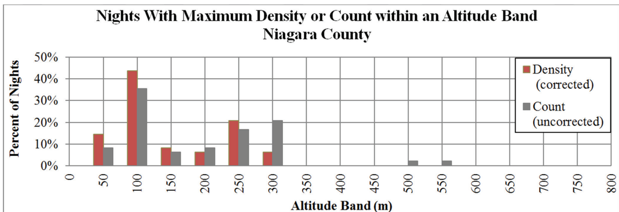
Figure 32. Maximum density by night. Percent of nights when the maximum density (targets/1,000,000 m 3 /altitude band) or count (targets/altitude band) occurred within 50-m altitude bands in Jefferson, Wayne, and Niagara County study sites during fall 2016. X-axis labels represent the top of the altitude band.
