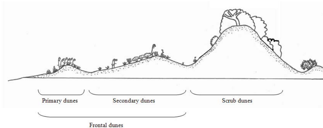
Figure 4. Generalized dune system profile for the Gulf Coast.
