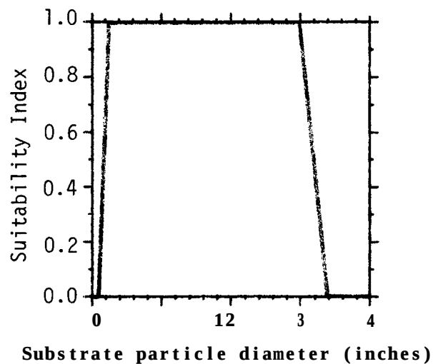
Figure 2. Category one SI curves for brown trout spawning and egg incubation velocity, depth, substrate, and temperature suitability.
