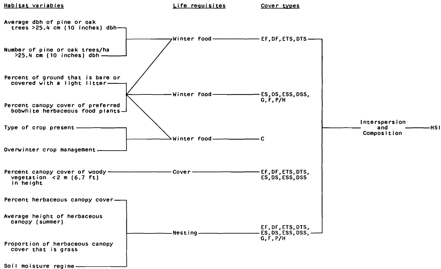
Figure 7. Relationships of habitat variables, life requisites, cover types, and the HSI in the bobwhite model.
