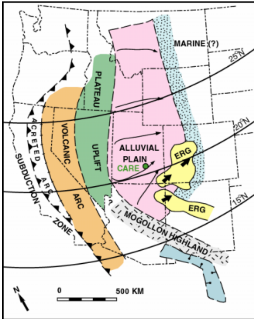
Figure 17. Upper Jurassic paleogeography. Thin arrows indicate fluvial dispersal. Thick arrows indicate wind directions. Saw teeth indicate the location of the subduction zone with the teeth on the overriding, upper lithospheric plate. Note the possible marine environment to the east where continental environments were previously established. The alluvial plain expanded to the east with time. CARE: Capitol Reef National Park. Modified from Lawton (1994).
