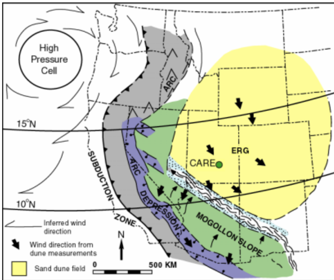
Figure 15. Lower Jurassic paleogeography. Thick arrows indicate eolian transport of sand. Thin arrows on Mogollon Slope indicate fluvial transport of sediments. Gray shading shows the location of the volcanic arc. Saw teeth indicate the location of the subduction zone with the teeth on the overriding, upper lithospheric plate. CARE: Capitol Reef National Park. Modified from Lawton (1994).
