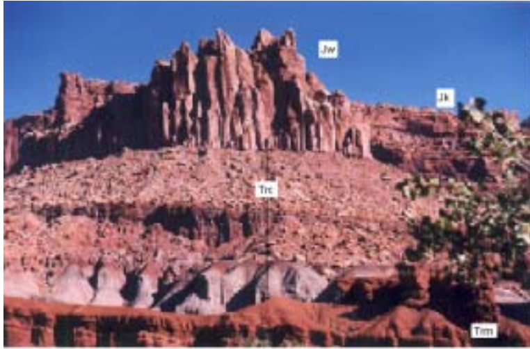
Figure 8. The red rock at the lower part of this photograph of “the Castle” from the Visitors Center parking lot is the Moody Canyon Member of the Triassic Moenkopi Formation (Trm). The Shinarump Conglomerate that normally overlies the Moody Canyon is absent at this locality. Above the Moody Canyon are the gray and purple beds of the Monitor Butte Member of the Chinle, the slope-forming red siltstone and sandstone of the Petrified Forest Member with the resistant “Capitol Reef bed” capping this member (ledge in the middle of the slope). The Owl Creek Member of the Chinle Formation (Trc) comprises the upper slope of mudstone, siltstone, and fine sandstone. “The Castle” is fractured Jurassic Wingate Sandstone (Jw). The Jurassic Kayenta Formation (Jk) caps the Wingate on the skyline. Photograph from Morris and others (2000).
