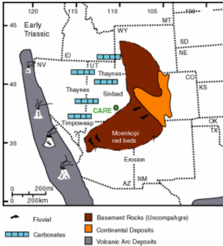
Figure 13. Paleogeographic map of the Lower Triassic, Moenkopi Formation during the second transgressive episode of the Early Triassic (Black Dragon and Sinbad Limestone members). CARE: Capitol Reef National Park. Modified from Dubiel (1994).
