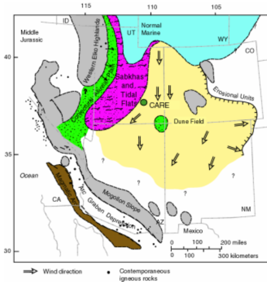
Figure 16. Middle Jurassic paleogeography during deposition of the Entrada Sandstone. Note that the northern marine environments have eliminated the sand source to the north (compare with Figure 18), yet Entrada ergs are widespread. CARE: Capitol Reef National Park. Modified from Peterson (1994).
