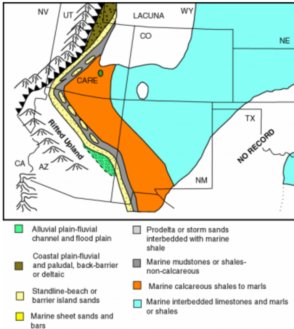
Figure 19. Upper Cretaceous paleogeography at the time of deposition of the Tununk Shale Member of the Mancos Shale. Saw teeth mark the leading edge of thrust faulting with the teeth on the overriding plate. Modified from Elder and Kirkland (1994).
