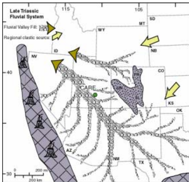
Figure 14. Paleogeographic map of the fluvial system in the Upper Triassic. CARE: Capitol Reef National Park. UN: Uncompahgre uplift; SL: San Luis uplift; FR: Front Range uplift. Highlands are shaded a solid gray. Modified from Dubiel (1994).
