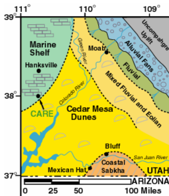
Figure 11. Lower Permian depositional environments in southeastern Utah during deposition of the Cedar Mesa Sandstone. CARE: Capitol Reef National Park. Modified from Huntoon and others (2000).
