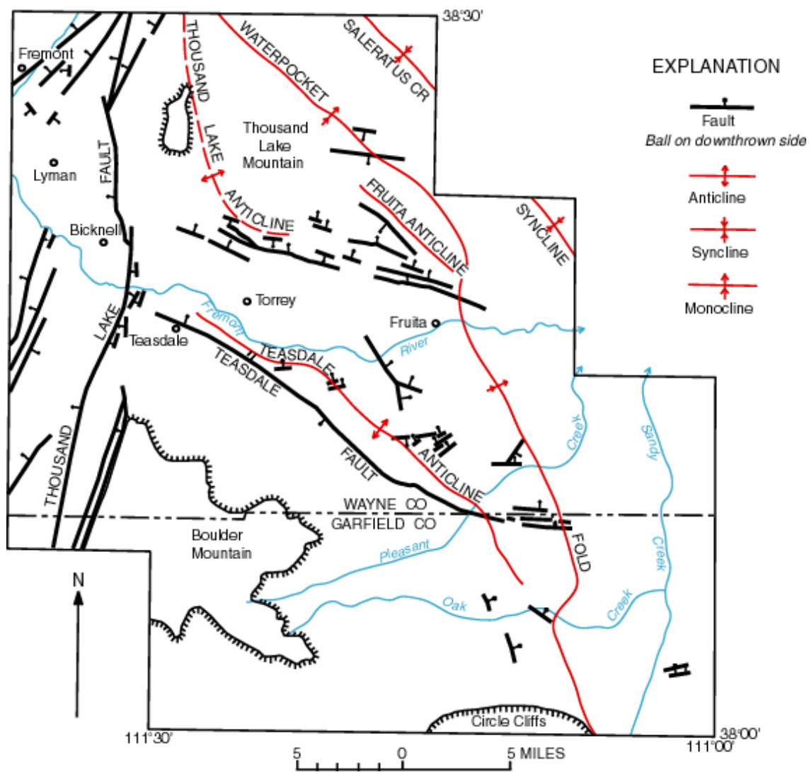
Figure 3. Major structural features in the Capitol Reef area. Modified from Smith and others, 1963.
