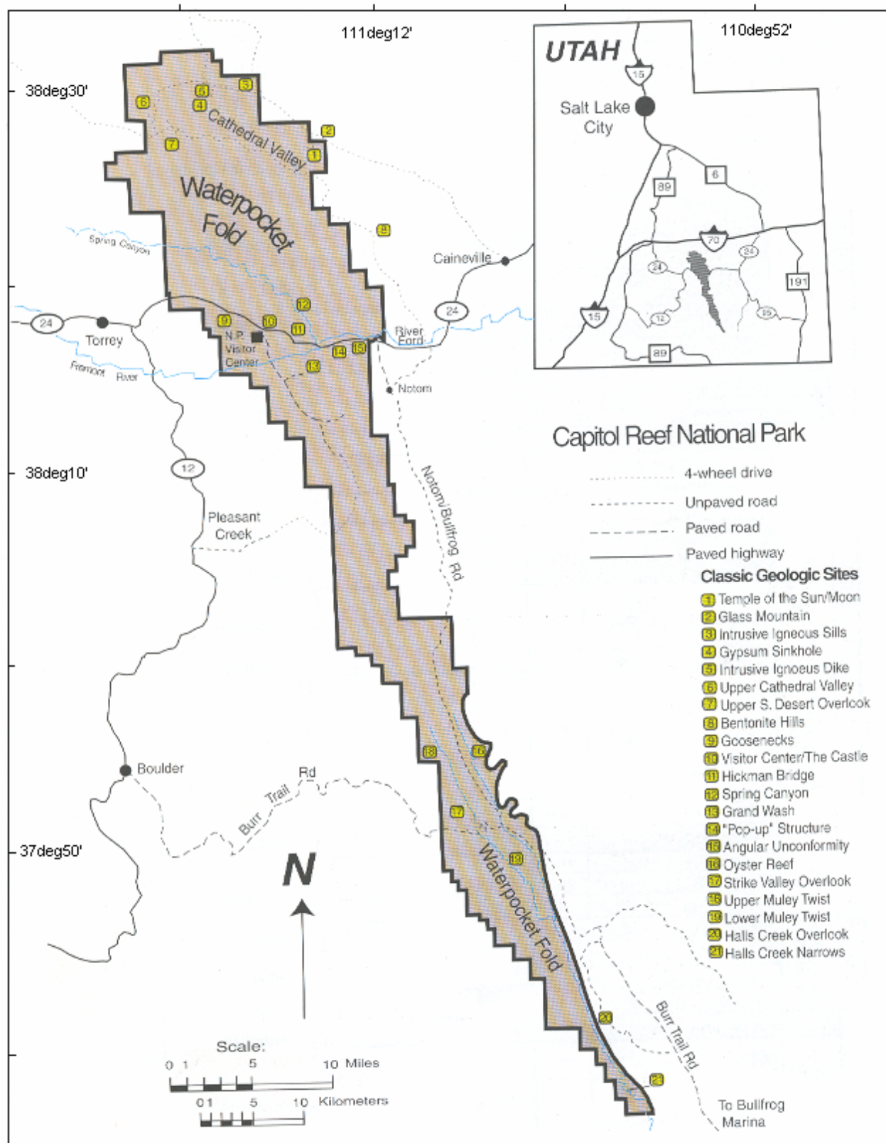
Figure 1. Location map of Capitol Reef National Park. From Morris and others, 2000.
