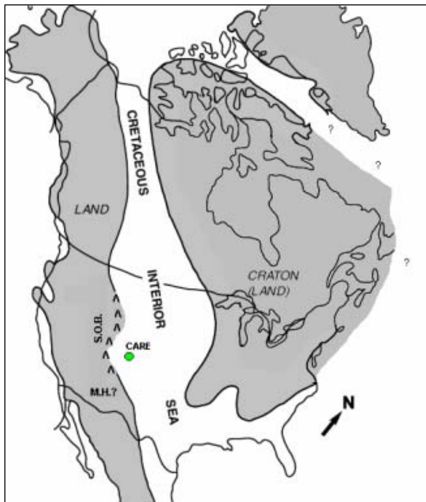
Figure 18. Location of the Cretaceous Period, Western Interior Seaway. Shaded areas indicate land above sea level. North indicates the Cretaceous north. Modified from Rice and Shurr (1983).
