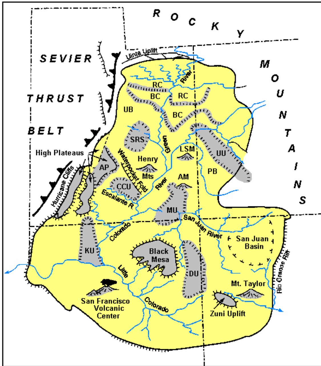
Figure 2. The Colorado Plateau physiographic province, showing some of the significant uplifts, basins, faults, volcanic centers, and rivers. High areas are shown in gray: AM, Abajo Mts.; AP, Aquarius Plateau; BC, Book Cliffs; CCU, Circle Cliffs Uplift; DU, Defiance Uplift; KU, Kaibab Uplift; LSM, La Sal Mts.; MU, Monument Upwarp; RC, Roan Cliffs; SRS, San Rafael Swell; UU, Uncompahgre Uplift. Basins: PB, Paradox Basin; UB, Uinta Basin. Capitol Reef National Park is located on the Waterpocket Fold. Leading edge of Sevier Thrust Belt is shown with sawteeth on upper, overriding thrust plate. Modified from Kiver and Harris, 1999.
