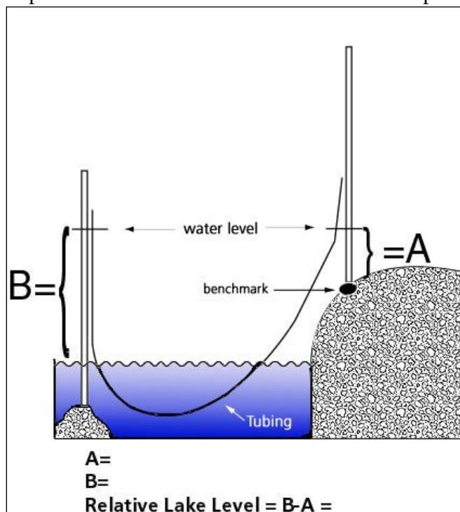
Figure 5.2. Set-up diagram of the “water level” method of lake level determination.
