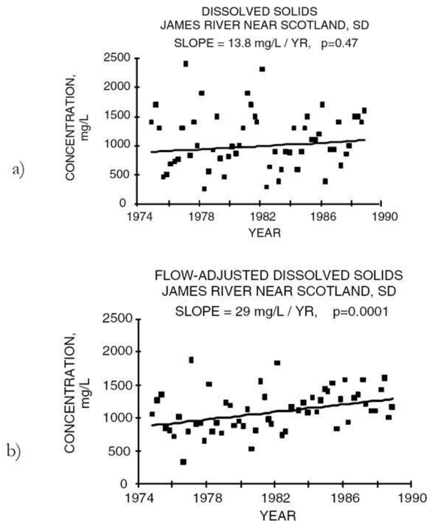
Figure 21.13. Comparison of Seasonal Kendall tests for trends in dissolved solids concentrations, before (a) and after (b) removing the effects of flow. The Sen estimate of linear trend associated with the Seasonal Kendall test is shown by the solid line. The trend in unadjusted data (a) is not statistically significant ( p=0.47 ). Using the same data, the trend following the removal of flow-related variability in dissolved solids concentrations is highly significant ( p=0.0001 ). The estimate of the magnitude of trend in flow-adjusted concentrations is about twice the estimate of the trend magnitude in raw concentrations. From Hirsch et al. 1991.
