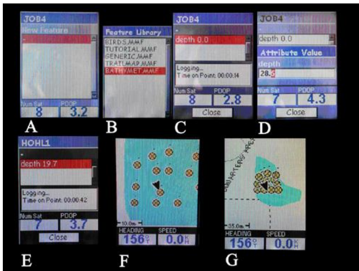
Figure 4.1. A-G: Screen captures from MobileMapper GPS unit illustrating key screens for conducting bathymetry.
