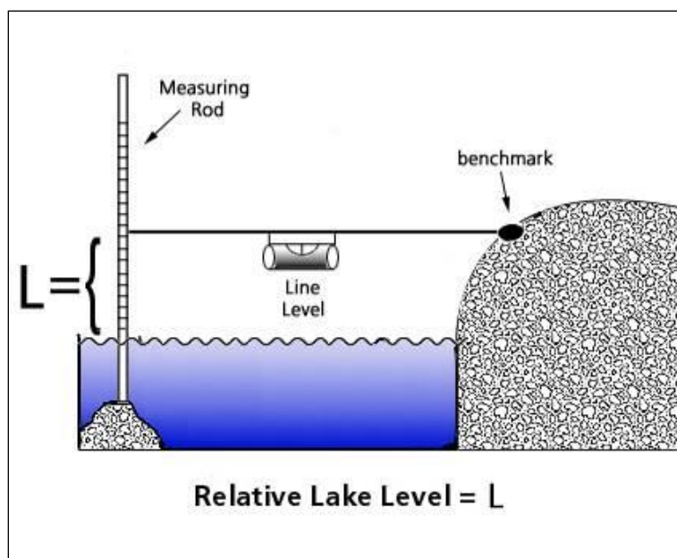
Figure 5.3. Set up diagram of the “Line Level” method of lake water level determination.
