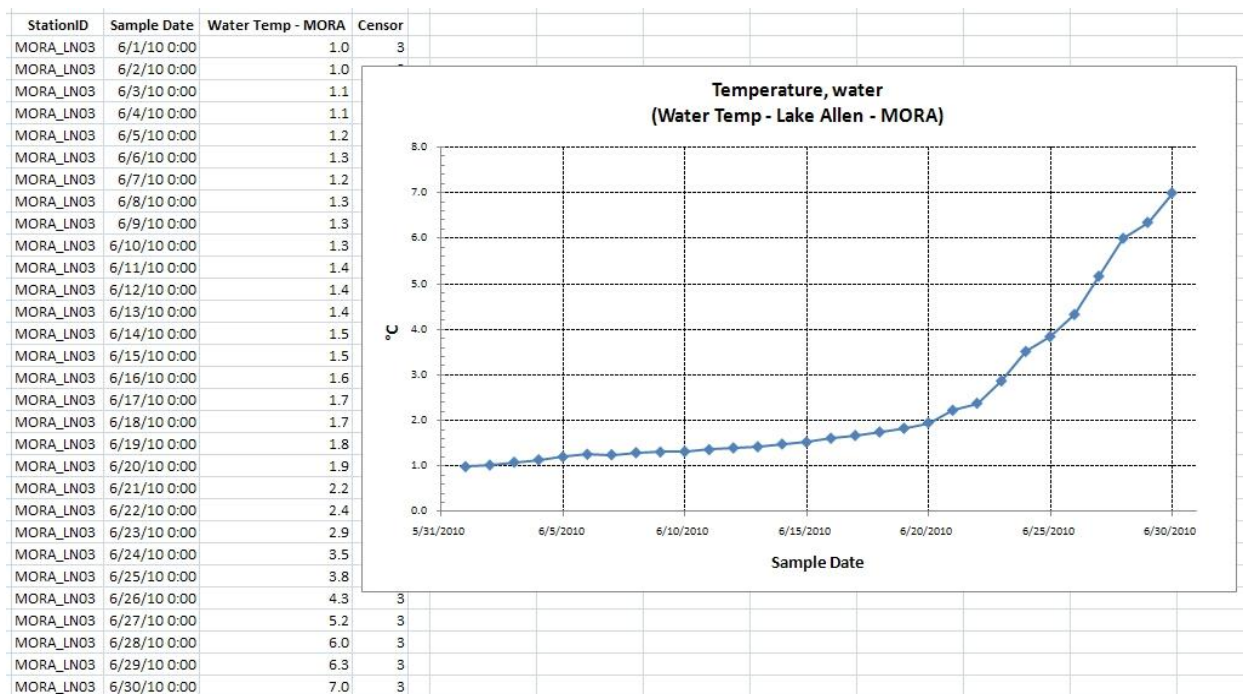
Figure 22.3. North Coast and Cascades Network water temperature graph generated from NPSTORET.
