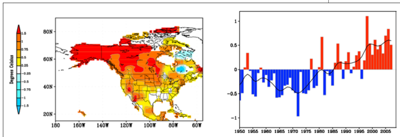
Figure 19. Observed annual average North American surface temperature, 1950–2007 (left) and the time series of the annual values of surface temperature averaged over North America (right). Annual anomalies are with respect to a 1971–2000 reference. The smoothed curve (black line) indicates low frequency variations. (Data source: UK Hadley Center’s CRUv3 global monthly gridded temperatures.) Source: Ray et al. 2008; reprinted with permission.
