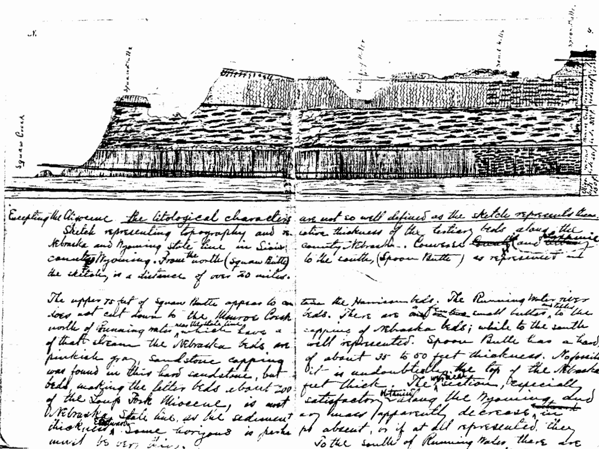
Fig. 1.2. Geological cross-section of the Hartville Table, from the Pine Ridge escarpment (Squaw Butte) to Spoon Butte, from 1904 field notes of O.A. Peterson, who indicated that the Arikaree tableland was made up of a sequence of superposed tabular rock units (Gering, Monroe Creek, Harrison, "Nebraska" [=Upper Harrison]). Line of section (north to south) nearly parallels Wyoming-Nebraska state boundary. The Niobrara River (Runningwater of Peterson) has cut the Niobrara Canyon at the center of the cross-section. In 1904, the faults that occur in the region (see Fig. 2.2) were not known to Peterson.
