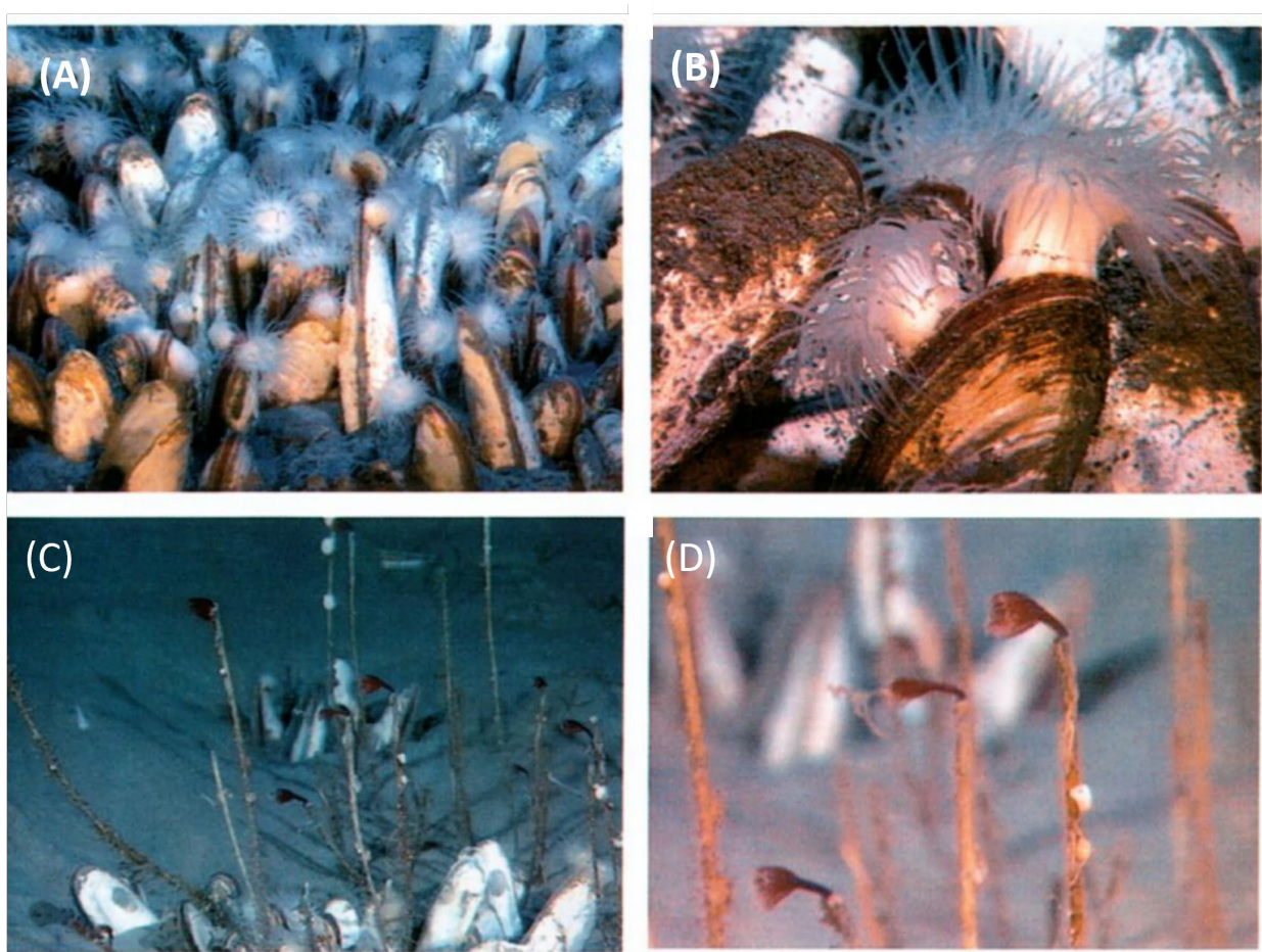
Figure 29. Drop camera photographs from Seep UAF073 showing (A-B) vesicomyid clams and (C-D) Pogonophoran tube worms (see white arrow Figure 25 for location).
