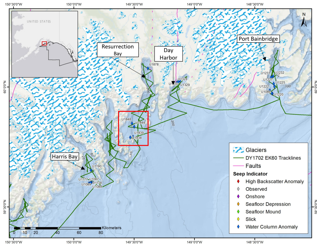
Figure 21. Seeps located within glacial fjords interpreted from EK60 water column data. Red box is location of Figure 22
