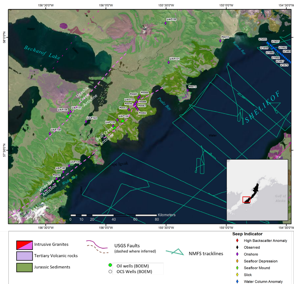
Figure 40. Satellite image of the Kanatak District with geologic units and exploratory wells.
