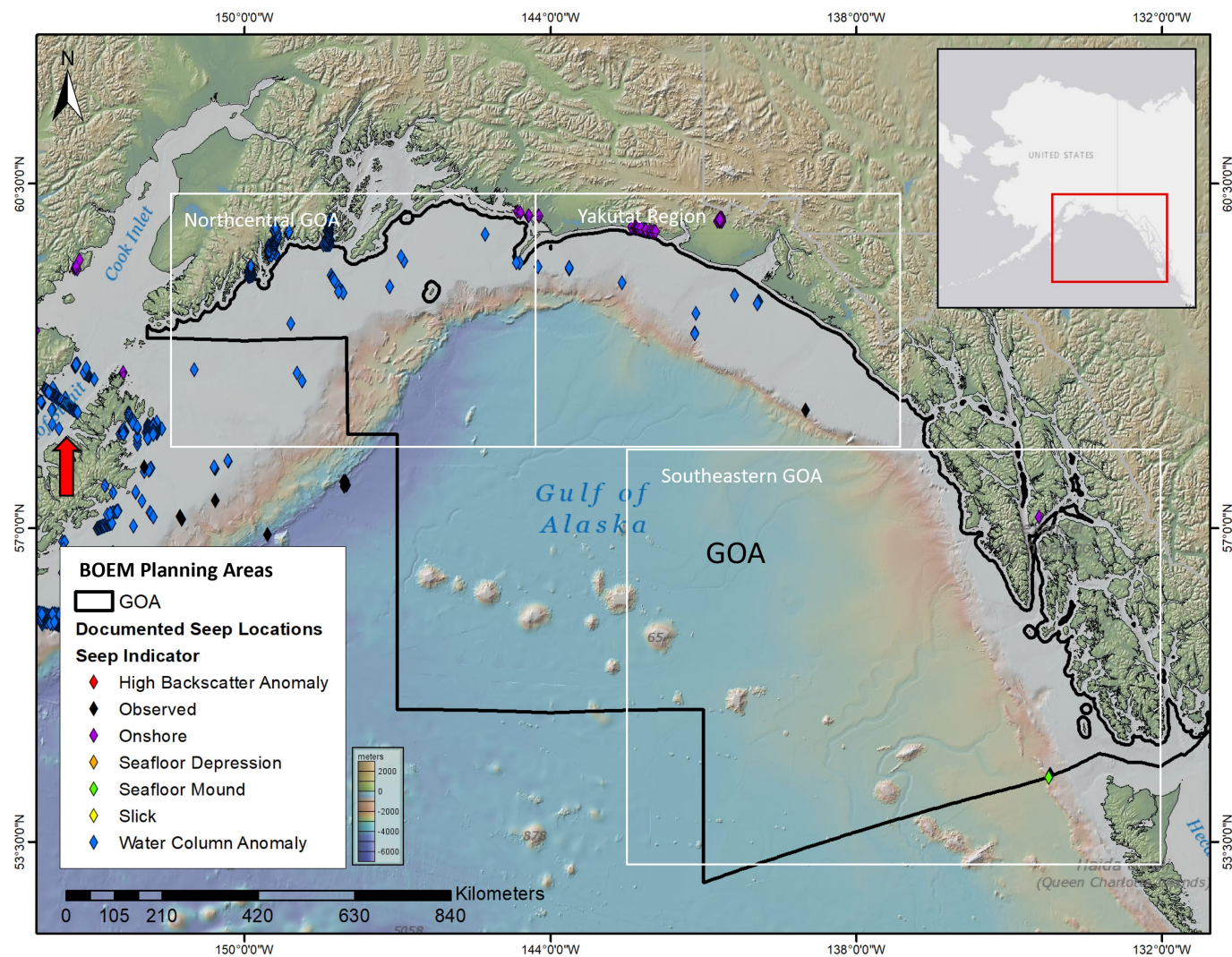
Figure 9. BOEM Gulf of Alaska (GOA) Planning Area with interpreted seep locations. White boxes are locations of overview sections below. Red arrow shows location of Figure 4.
