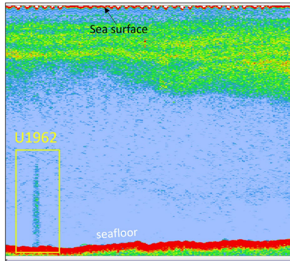
Figure 19. NOAA Fisheries single beam water column data (line DY1506_EK60-D20150810), showing water column anomalies interpreted as gas bubble plumes within the Bering Trough glacial valley (yellow box with associated seep number, see white arrow Figure 18 for seep location)
