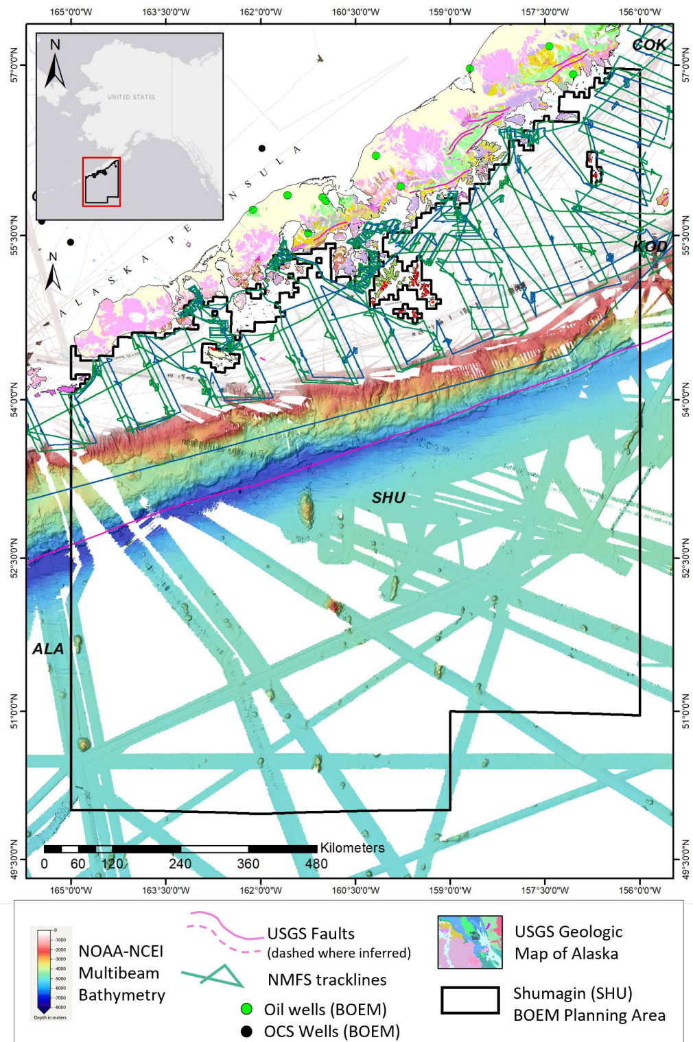
Figure 31. Data used in SHU for seep interpretation.
