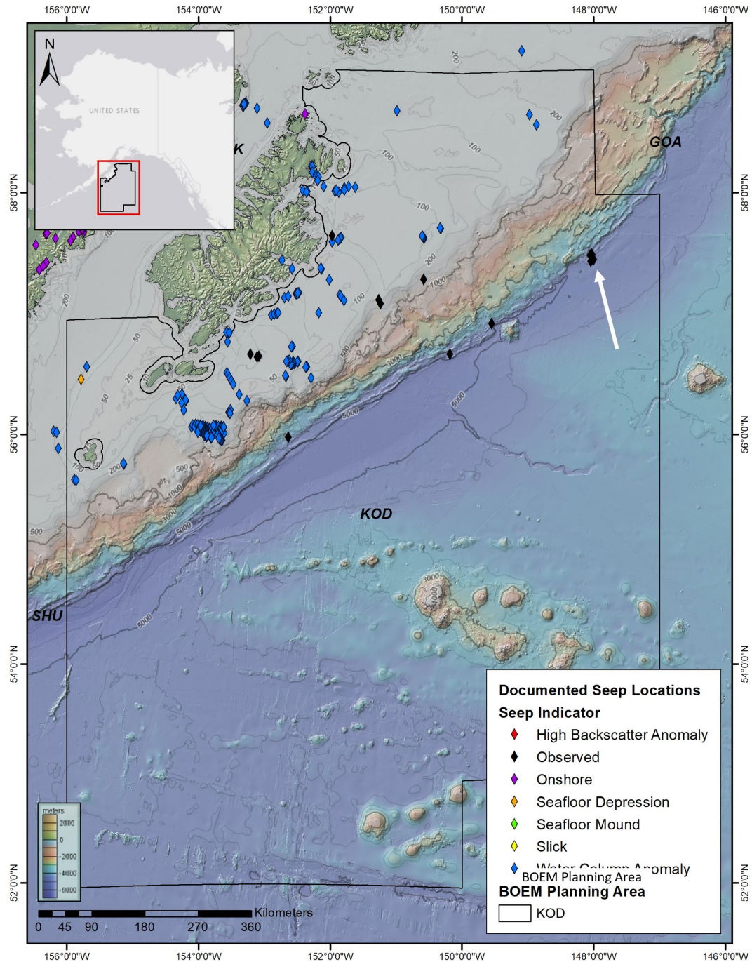
Figure 25. BOEM Kodiak (KOD) Planning Area with interpreted seep locations. White arrow shows location of seep #UAF073 discussed in text
