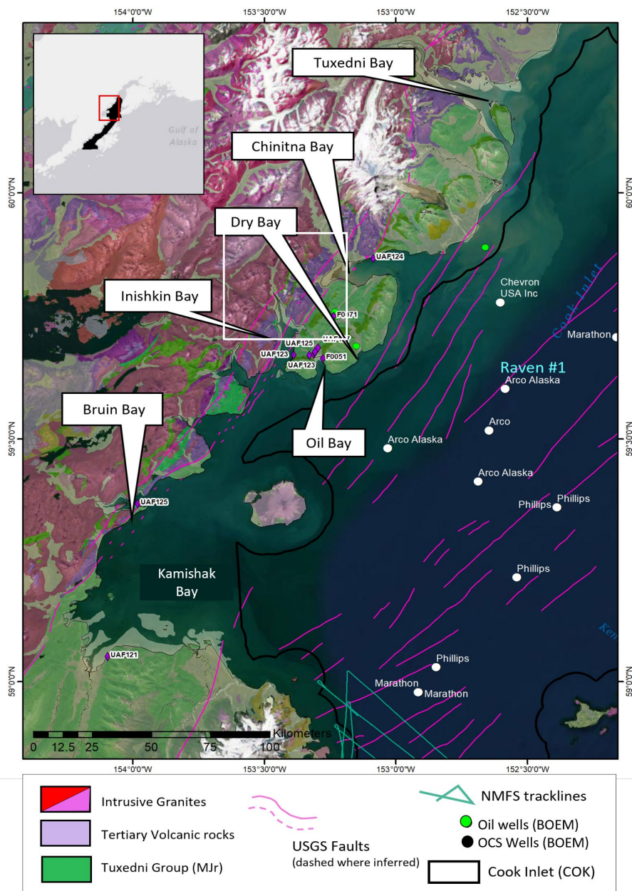
Figure 38. Satellite image of Chinitna District showing geologic units and exploratory wells. Numbered diamonds are seep locations from this study, white box is location of Figure 39.
