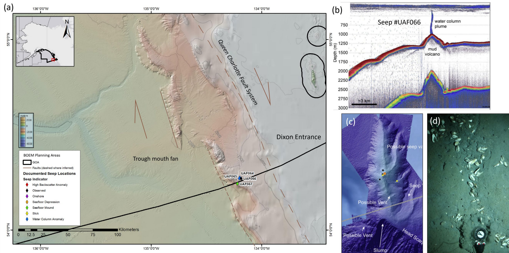
Figure 12. (a) Bathymetry at the Dixon Entrance along the Queen Charlotte Fault showing location of cold seeps and mud volcanos (see white box Figure 11 for location). (b) 18 kHz single beam echosounder and 3.5 kHz subbottom profile image of water column anomalies emanating from a mud volcano (seep #UAF066 in the accompanying data base). (c) multibeam image of the Dixon Entrance mud volcano, dots represent ROV dive locations (c-d modified from Greene et al. 2019). (d) chemosymbiotic clams at the top of the mud volcano.
