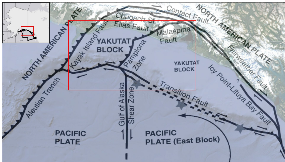
Figure 15. Geologic framework of the Gulf of Alaska, including major faults and regional subdivisions on the continental margin. Red box is location of Figure 18.
