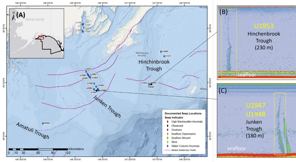
Figure 23. (A) Bathymetry of glacial troughs on the Northcentral GOA shelf showing fault locations (purple lines, dashed where inferred) interpreted by Liberty et al., 2019. (B-C) ME70 multibeam water column data (DY1307), showing water column anomalies interpreted as gas bubble plumes in Hinchinbrook and Junken Troughs (yellow boxes with seep numbers).
