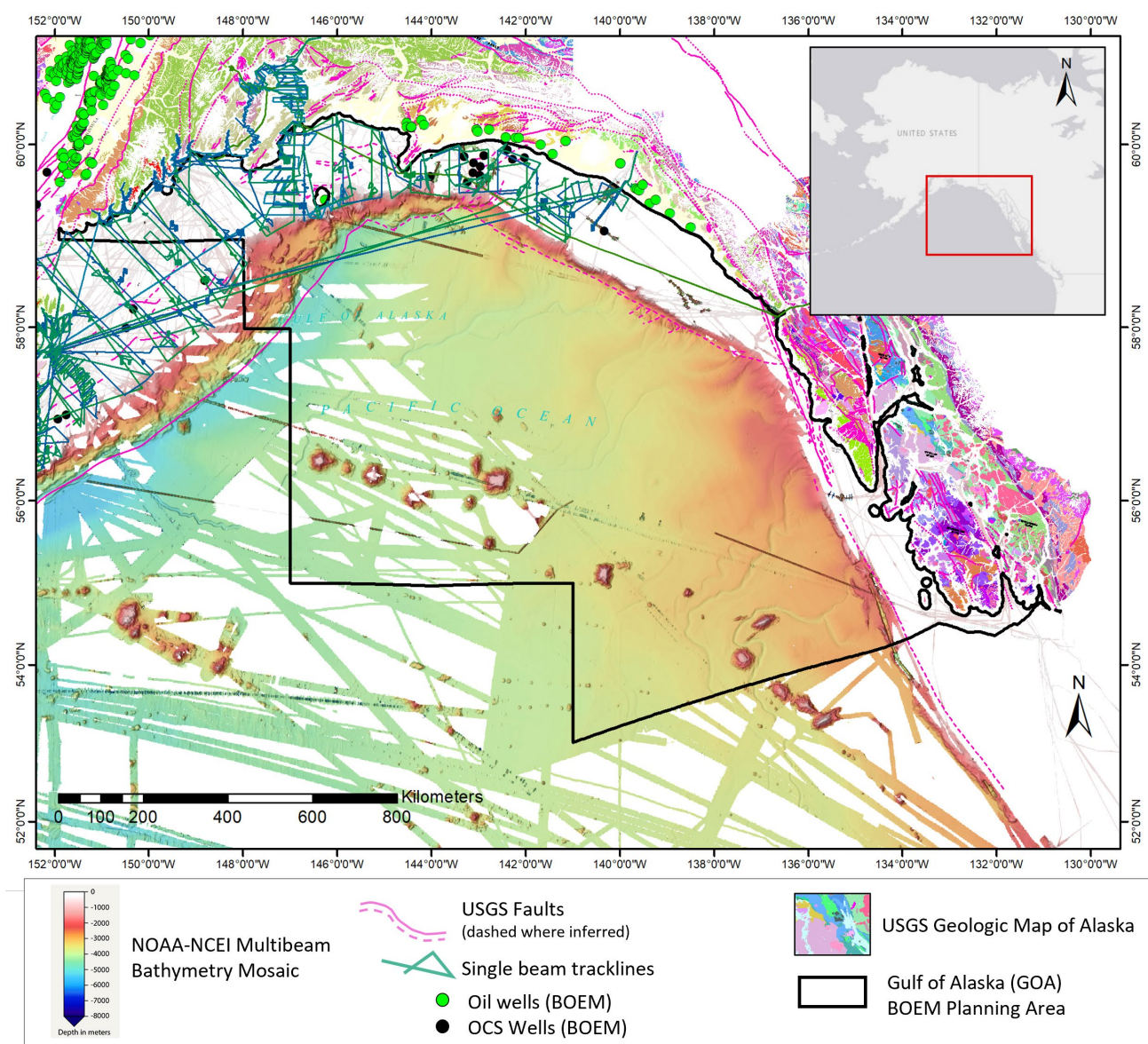
Figure 10. Data used in the GOA for seep interpretation.
