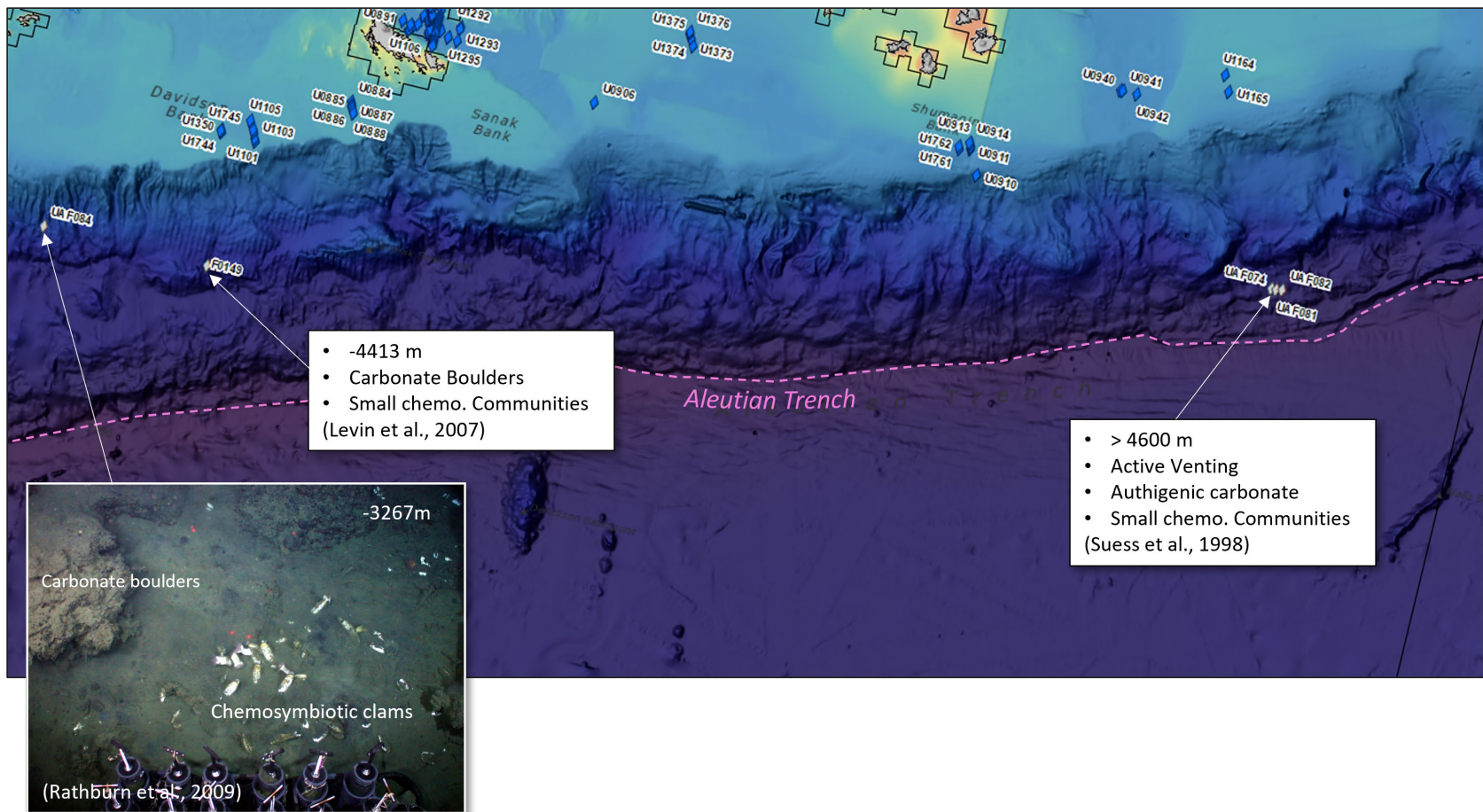
Figure 35. Seeps within the Aleutian subduction zone within the Shumagin Planning Area. Tow camera image . (Callout) from ROV Jason II aboard the R/V Revelle, July 2004.
