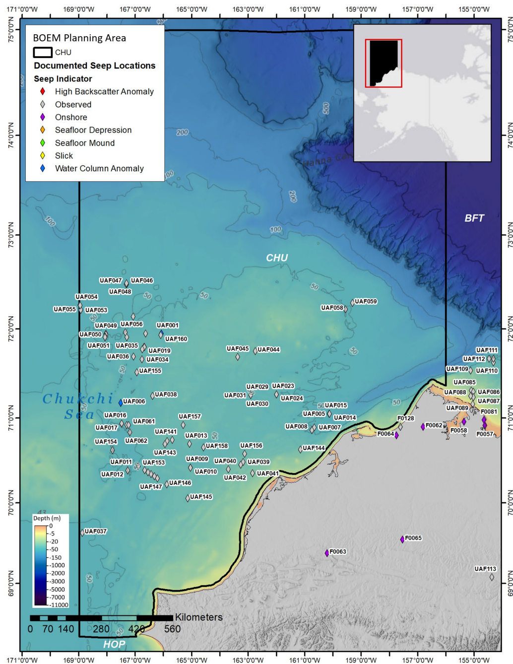
Figure 44. . Bathymetry within the BOEM Chukchi (CHU) Planning Area with interpreted seep locations Bathymetry from NOAA NCEI.
