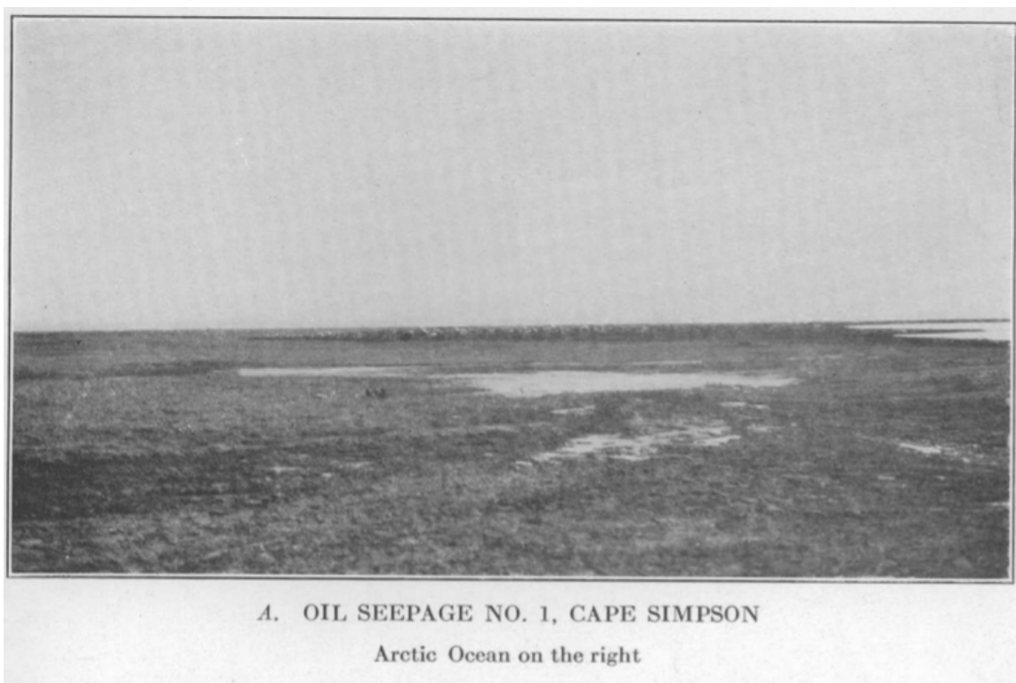
Figure 48 Photograph of “oil seepage No.1” near Cape Simpson.
