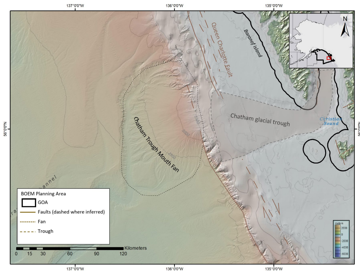
Figure 14. Chatham glacial trough and trough mouth fan along the Queen Charlotte Fault system (see black box Figure 11 for location.
