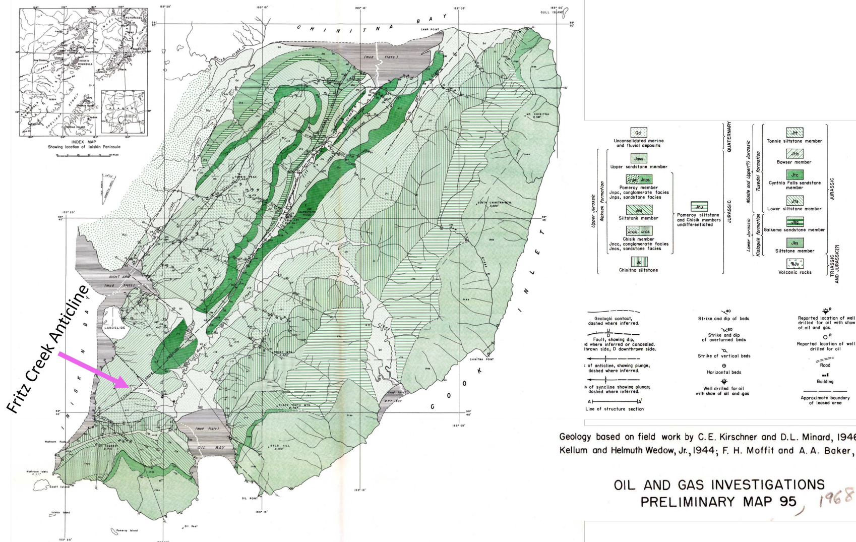
Figure 39. Geology of the Iniskin Peninsula showing Fritz Creek Anticline and folded Tuxedni sandstone (solid dark green unit).
