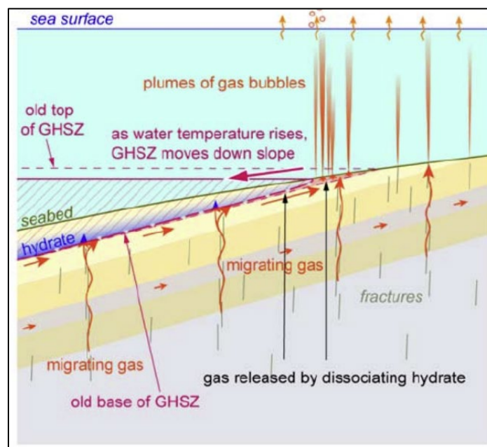
Figure 6. Profile of upper continental slope and location of gas hydrate stability zone (GHSZ) where gas is released on the seafloor at the shelf edge.
