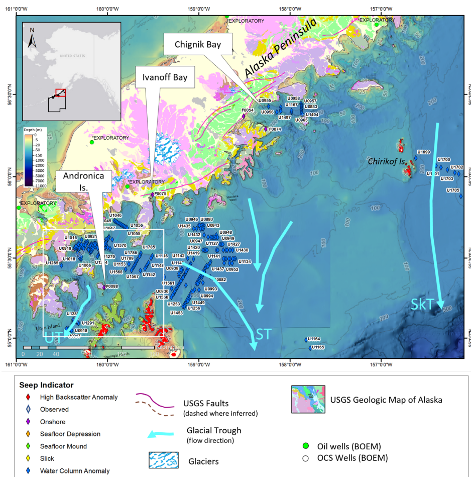
Figure 32. Bathymetry around Alaska Peninsula showing glacial troughs and flow directions; ST=Shumagin Trough; SkT=Shelikof Trough; UT=Unga Trough. White box is location of Figure 34. Bathymetry from NOAA-NCEI.
