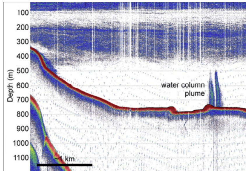
Figure 13. 18 kHz single beam echosounder and 3.5 kHz subbottom profile image of water column anomalies at the base of a submarine landslide glide block in the Southern GOA.
