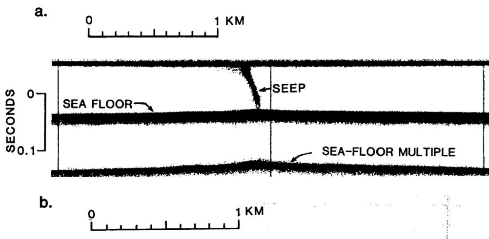
Figure 28. Seismic reflection image from Middle Albatross Bank showing water column anomaly interpreted as a gas seep.
