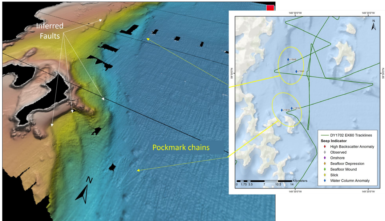
Figure 22. perspective view of bathymetry at the southern end of Resurrection Bay (see red box Figure 21 for location) showing pockmarked seafloor corresponding to gas bubble plumes interpreted from NMFS single beam data (yellow outlined areas on callout map).
