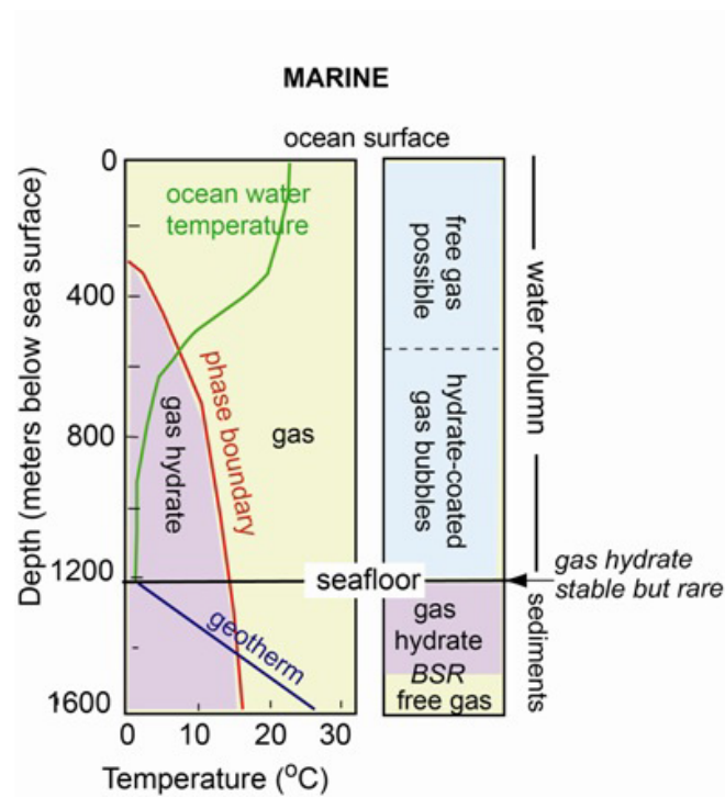
Figure 5. Phase diagram for gas hydrate stability in the marine environment.
