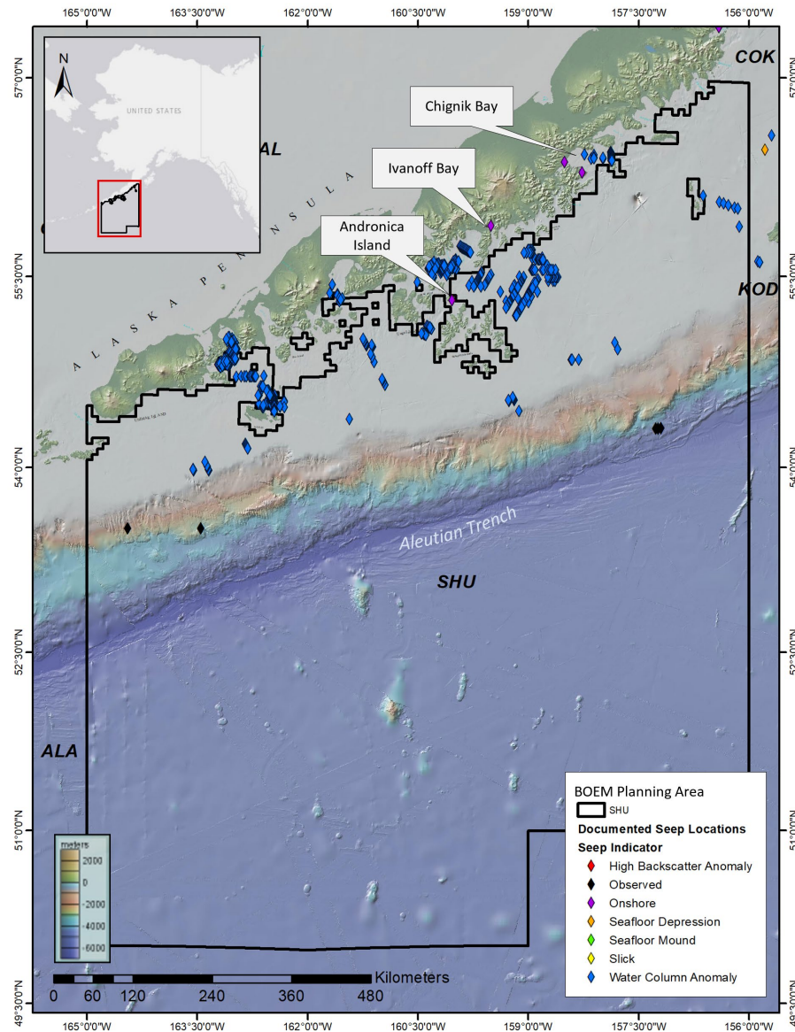
Figure 30. . Bathymetry within the BOEM Shumagin (SHU) Planning Area with interpreted seep locations
