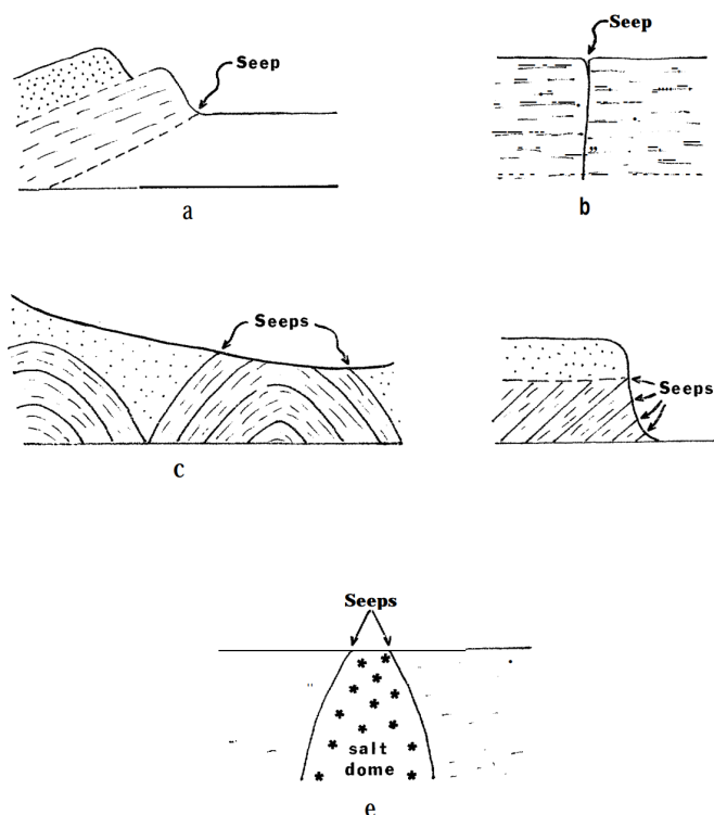
Figure 2. Types of oil seeps (a) fluids utilizing exposed tilted bedding planes (b) fluids feeding into fissures and fault planes (c-d) fluid accumulations exposed through erosion of unconformities (e) seeps associated with intrusions e.g. mud volcanos, salt.
