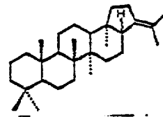
XXI. hop-21(22)-ene
