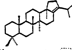
XXII. hop-17(21)-ene
