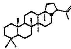
XX. diploptene
