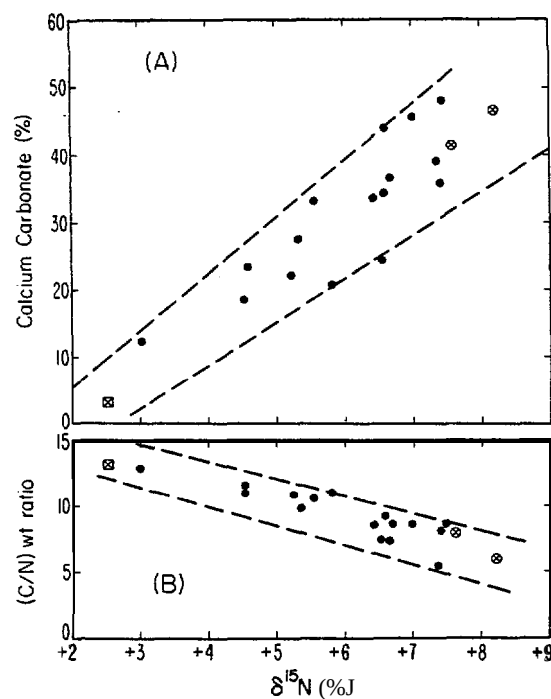
Fig. 3. Plot of \delta^{15}N(\text{‰}) versus calcium carbonate content (%) and C/N weight ratio for flocculent material. . San Pedro Shelf samples. \circ Catalina Harbour control station. \boxtimes Sewage effluent.
