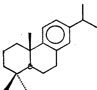
X* Dehydroabietane
