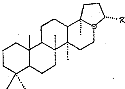
II. 17α(4)-Hopanes
