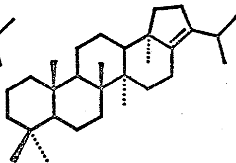
V. Hop-17(21)-ene
