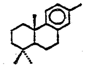
XIV. 13-methylpodocarpane-8,11,13-triene
