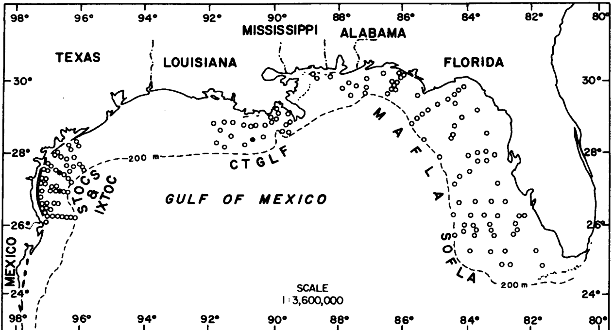
Figure 2-49. Distribution of Levinsenia reducta on the outer continental shelf of the northern Gulf of Mexico based on its occurrence (●) in BLM-OCS monitoring programs.
