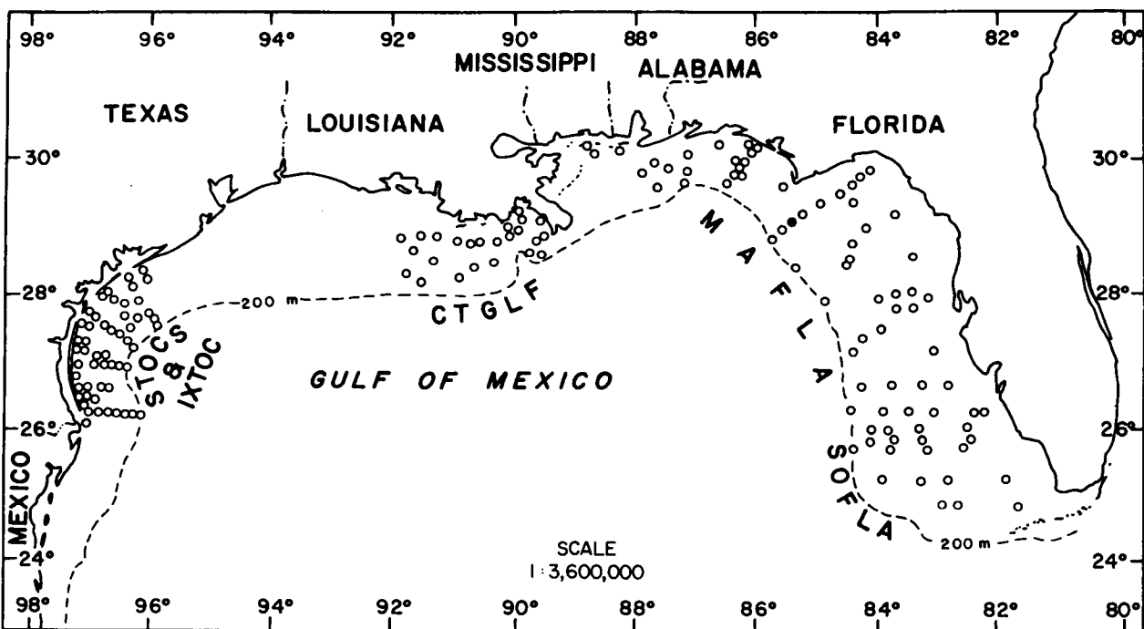
Figure 3-1. Distribution of Questa caudicifra on the outer continental shelf of the northern Gulf of Mexico based on its occurrence (●) in BLM-OCS monitoring programs.
