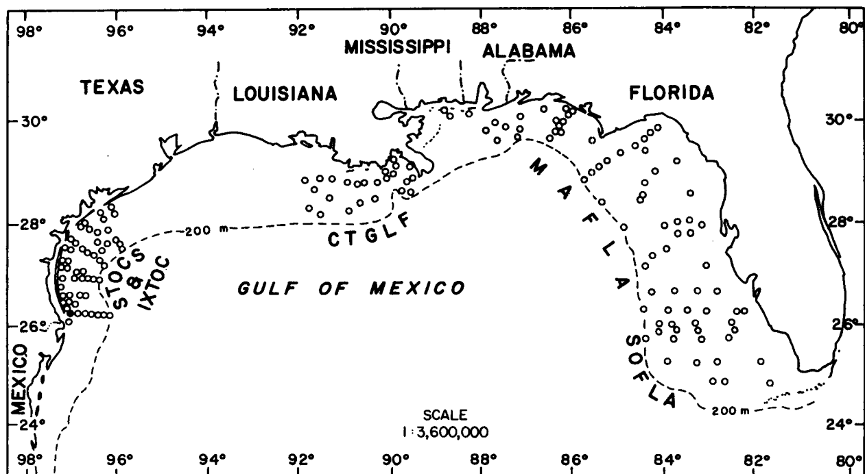
Figure 1-33. Distribution of Scoloplos sp. B on the outer continental shelf of the northern Gulf of Mexico based on its occurrence (●) in BLM-OCS monitoring programs.
