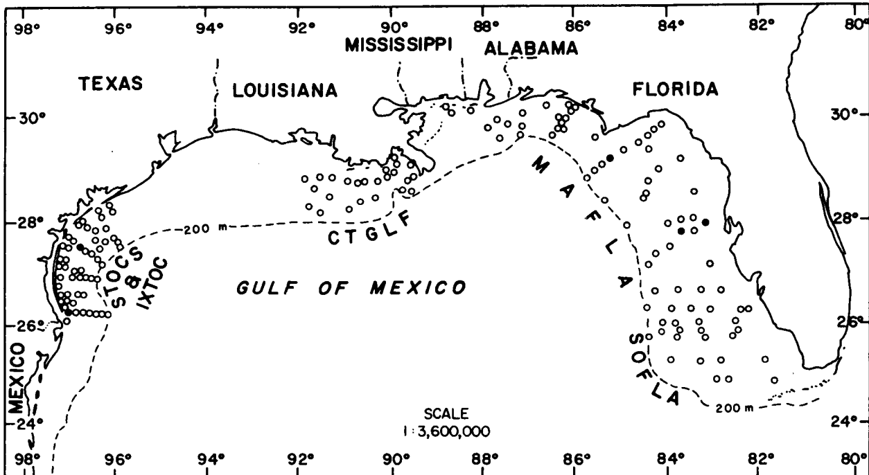
Figure 2-7. Distribution of Aricidea ( Aricidea ) wassii on the outer continental shelf of the northern Gulf of Mexico based on its occurrence (●) in BLM-OCS monitoring programs.
