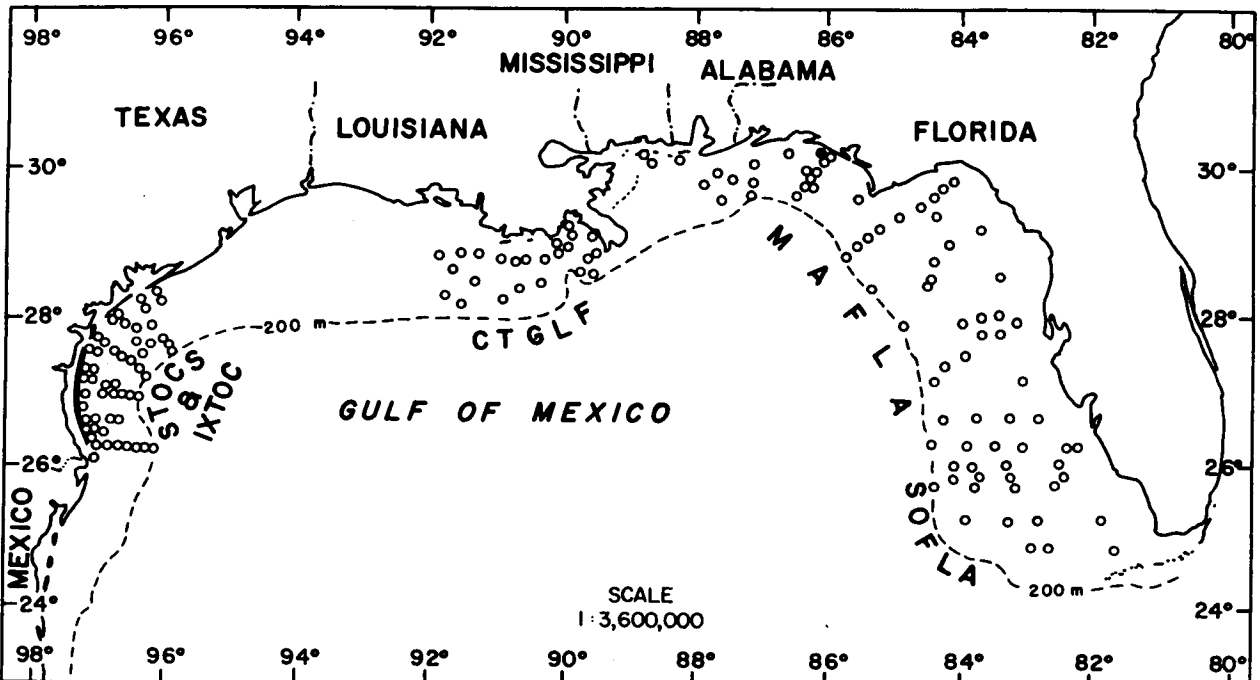
Figure 3-3. Distribution of Novaquestia trifurcata on the outer continental shelf of the northern Gulf of Mexico based on its occurrence (●) in BLM-OCS monitoring programs.
