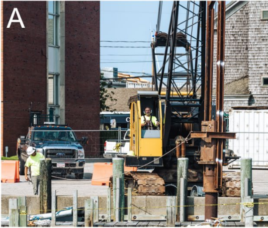
Figure 3. Picture of the impact (A) and vibratory (B) hammers used to drive the pile.
