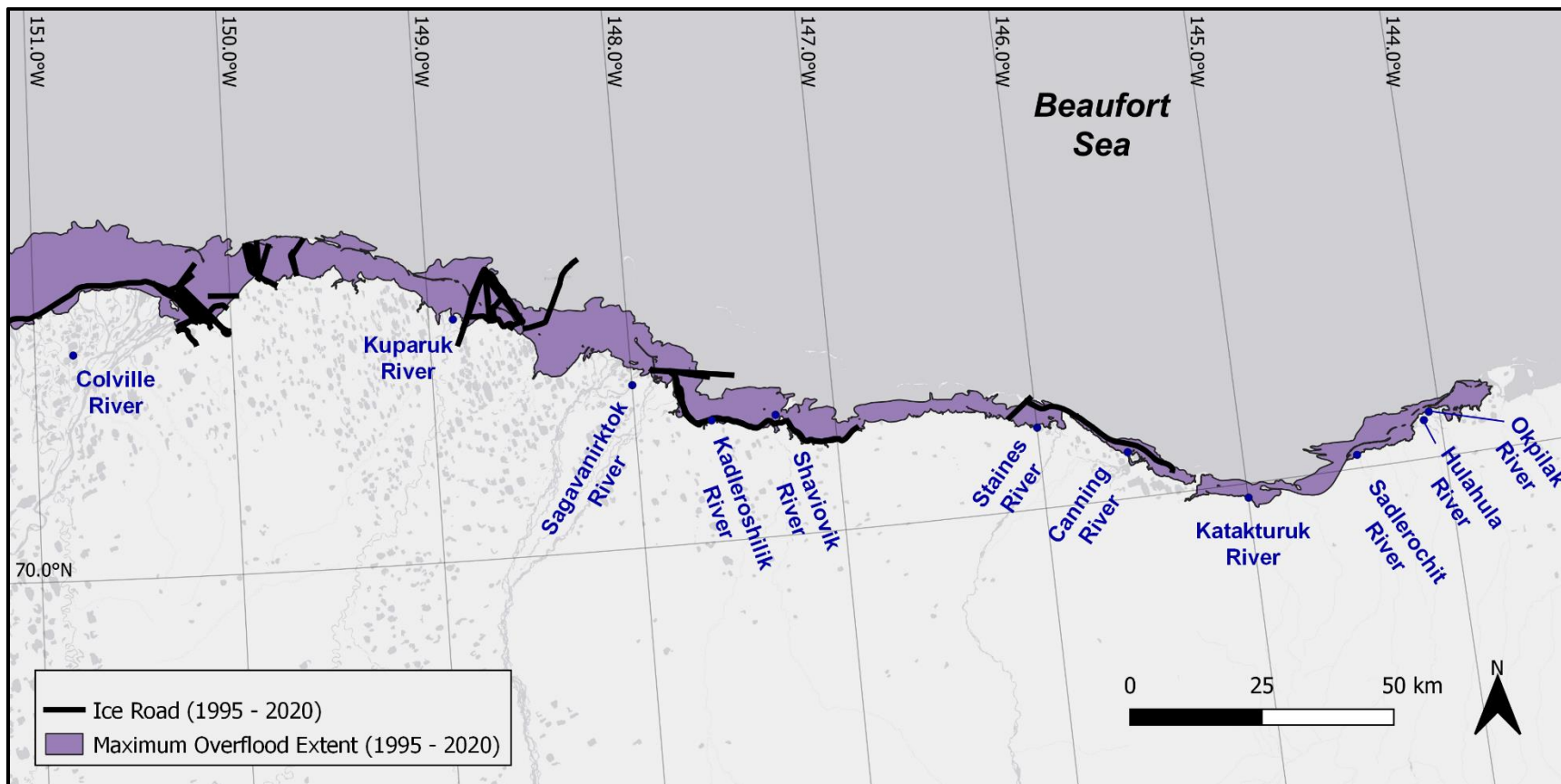
Figure 46. Ice road locations relative to maximum overflow extent, east study area, 1995–2020
