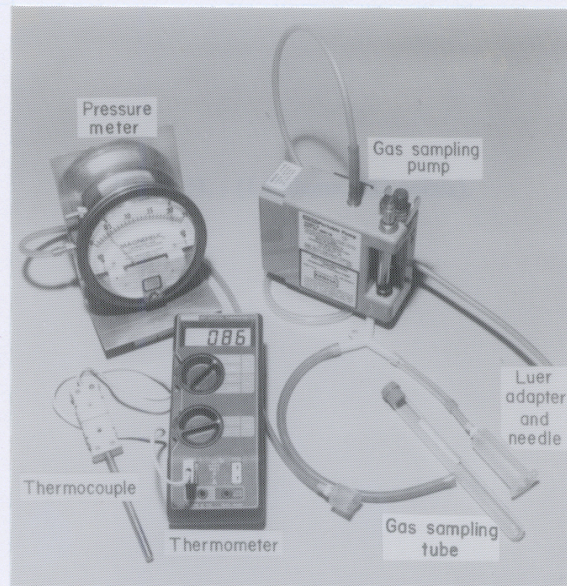
Figure 11.—Equipment used to measure borehole temperature and pressure and to obtain gas samples.
