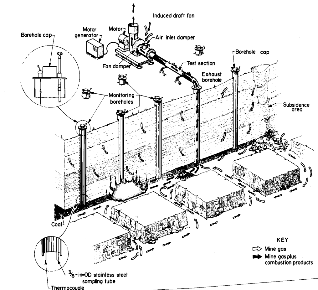
Figure 1.—Mine fire diagnostic technique applied to abandoned mine fire site (artist's depiction).
