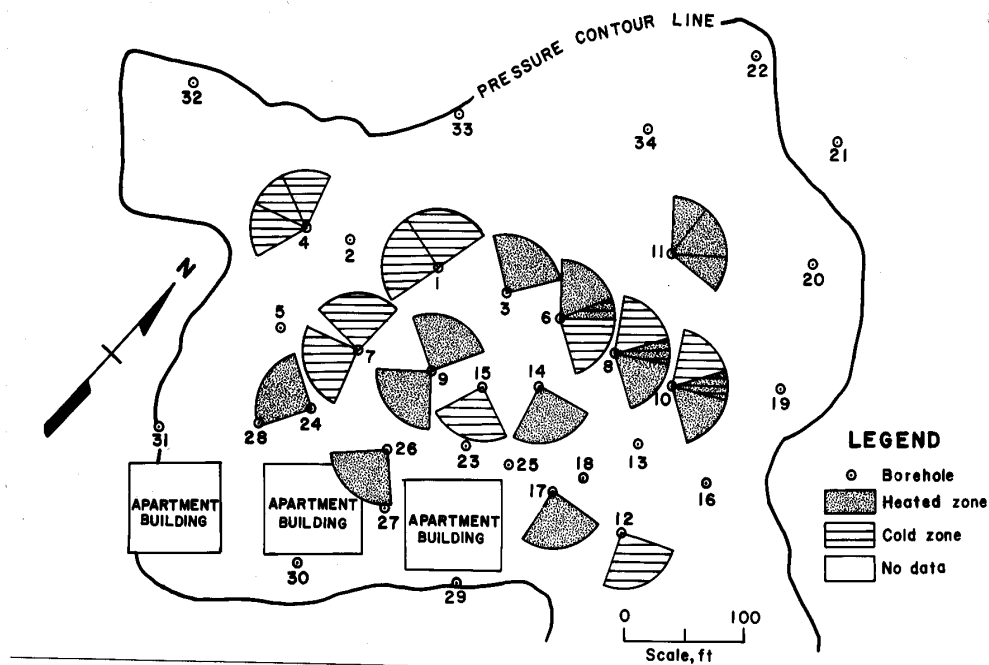
Figure 13.—Combined communication results from tests at boreholes 3 and 26.
