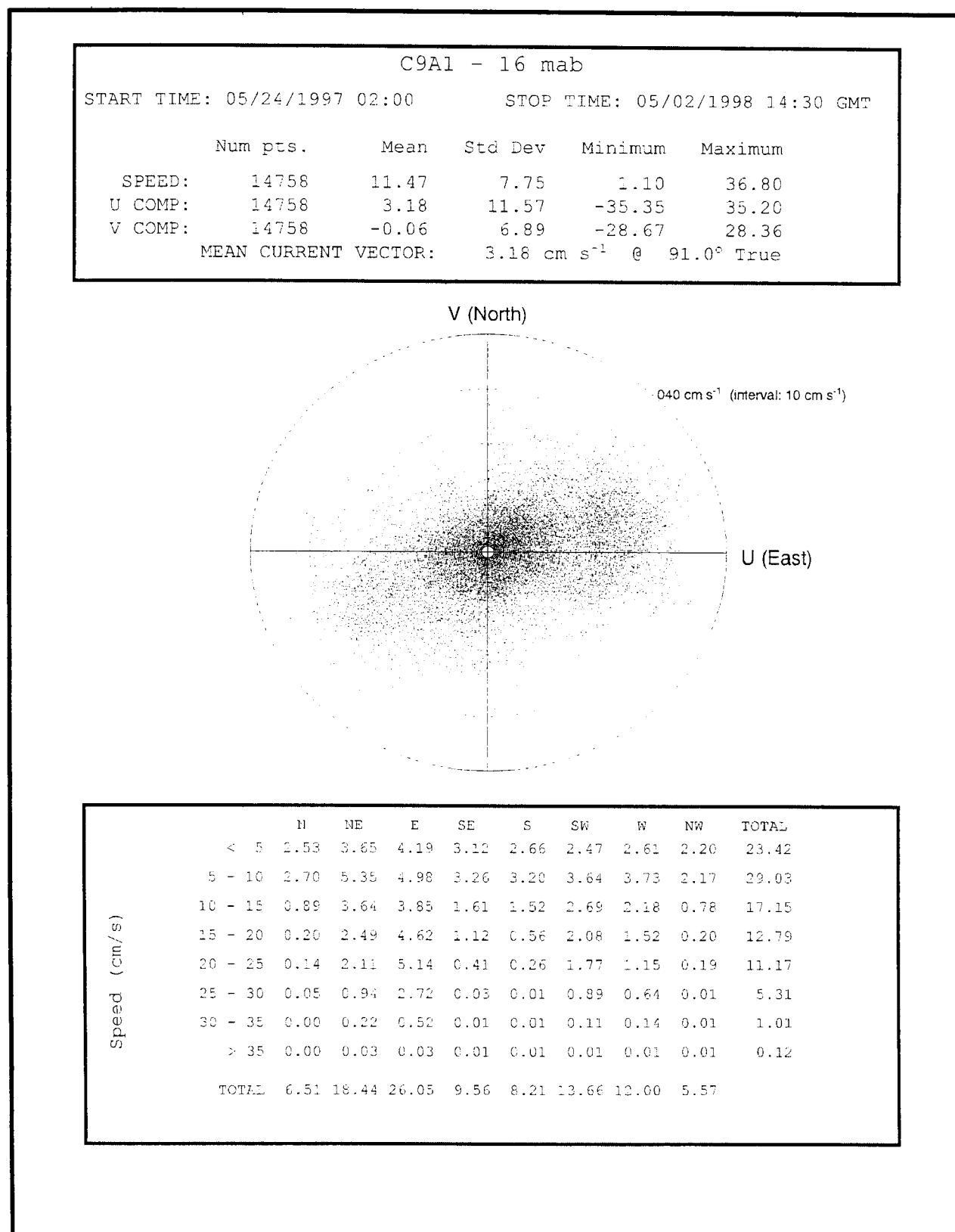
Fig. 7.8. Summary of current meter observations at Site 9A at 16 meters above the bottom (mab) for the period 24 May 1997 through 2 May 1998: basic statistics (top), scatter plot (middle), and percent joint occurrence of speed and direction (bottom).
