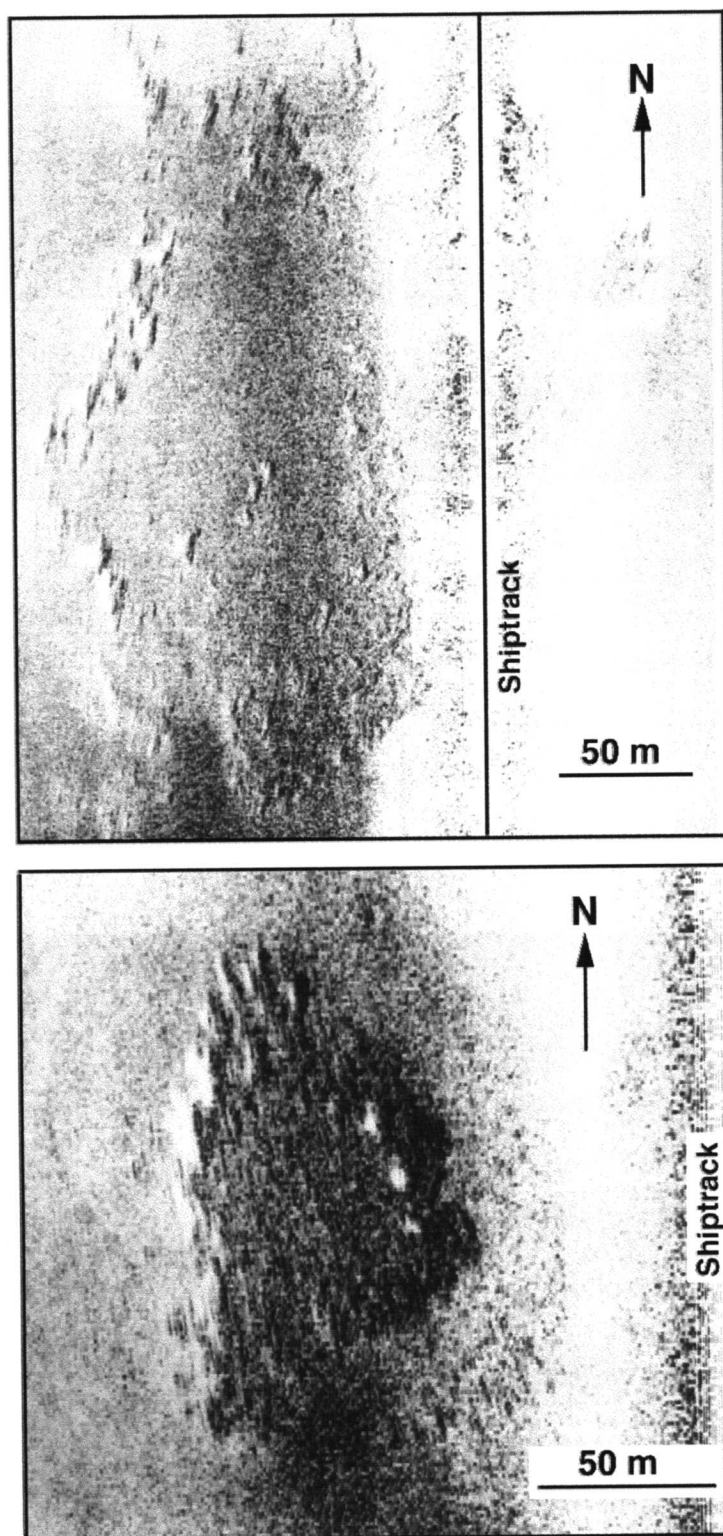
Fig. 4.18. Side-scan sonar images showing complex, irregular mounds from Megasite 2. Conventions as in Fig. 4.17.
