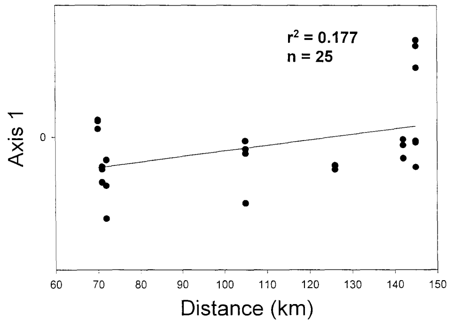
Fig. 9.3. Plots of Axis 1 scores from correspondence analysis against (a) water depth and (b) distance from the Mississippi River mouth. Lines determined by least squares linear regression.
