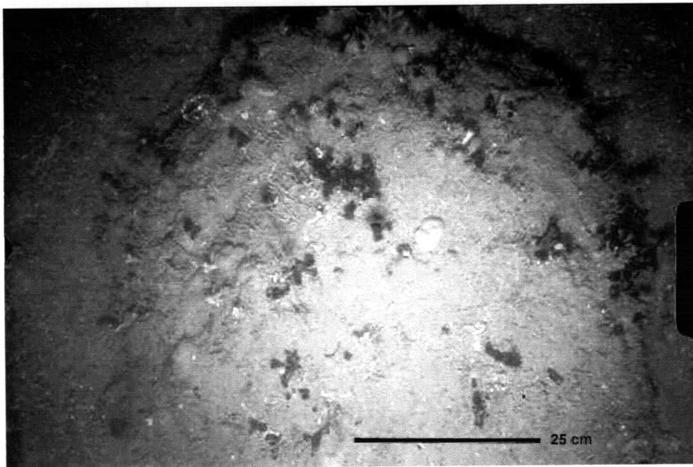
Figure 10.1. Examples of substrate classifications. A. Vertical outcrop, no sediment cover and large-scale perforation with medium surface roughness. B. Mounded outcrop, moderate silty veneer and no sand-fill.
