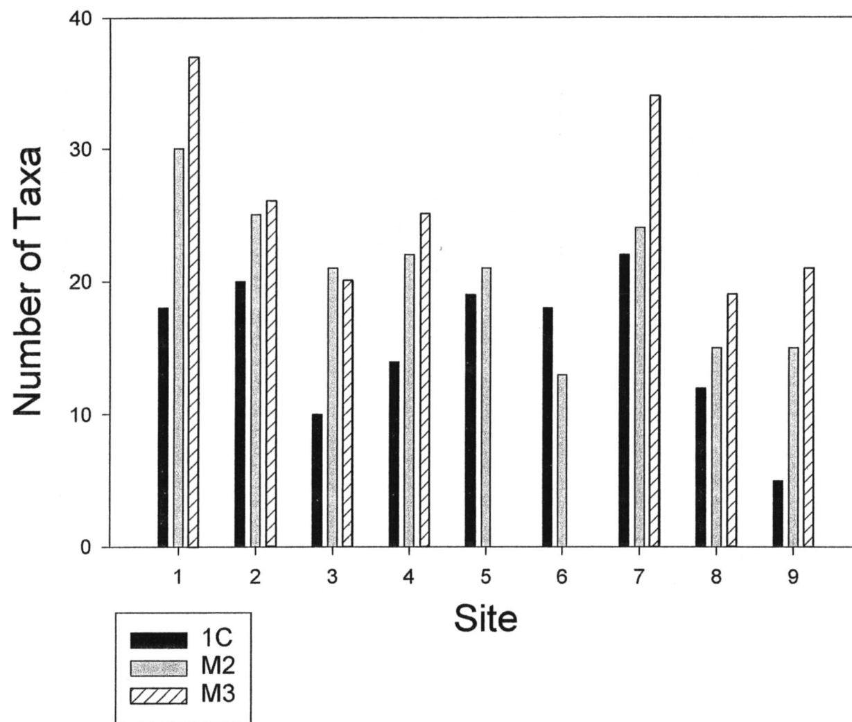
Fig. 9.1. Total fish taxa observed in video transects across study Sites 1 through 9 for Cruises 1C, M2, and M3.
