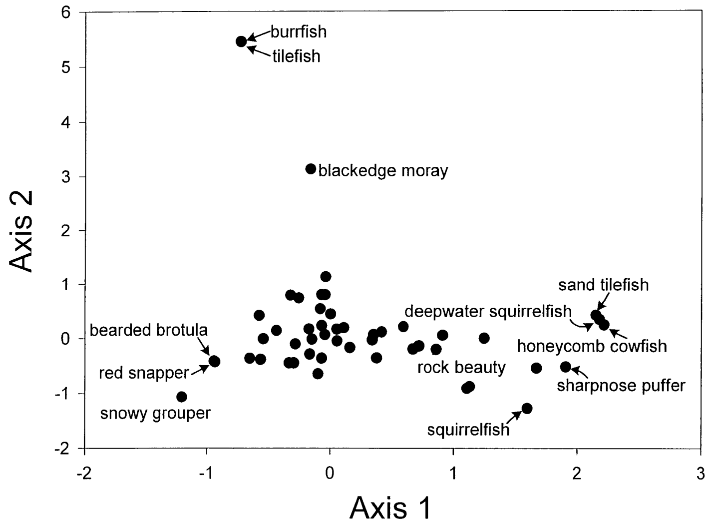
Fig. 9.4. Taxa scores from correspondence analysis of a taxa-by-samples matrix based on video transects plotted on Axes 1 and 2.
