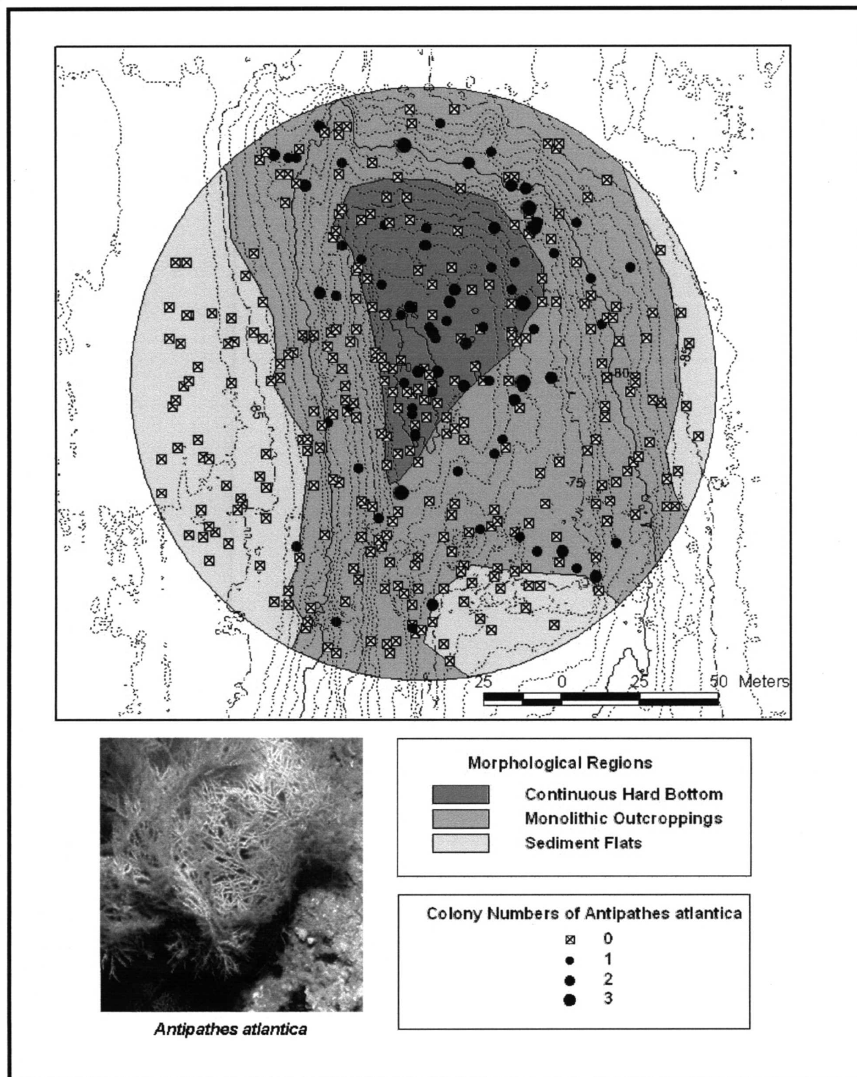
Figure 10.6. Numbers of Antipathes atlantica in random photo stations from Site 7. Contiguous morphological regions were derived from a combination of video and photo analysis, but correspond to attributes in the photos.
