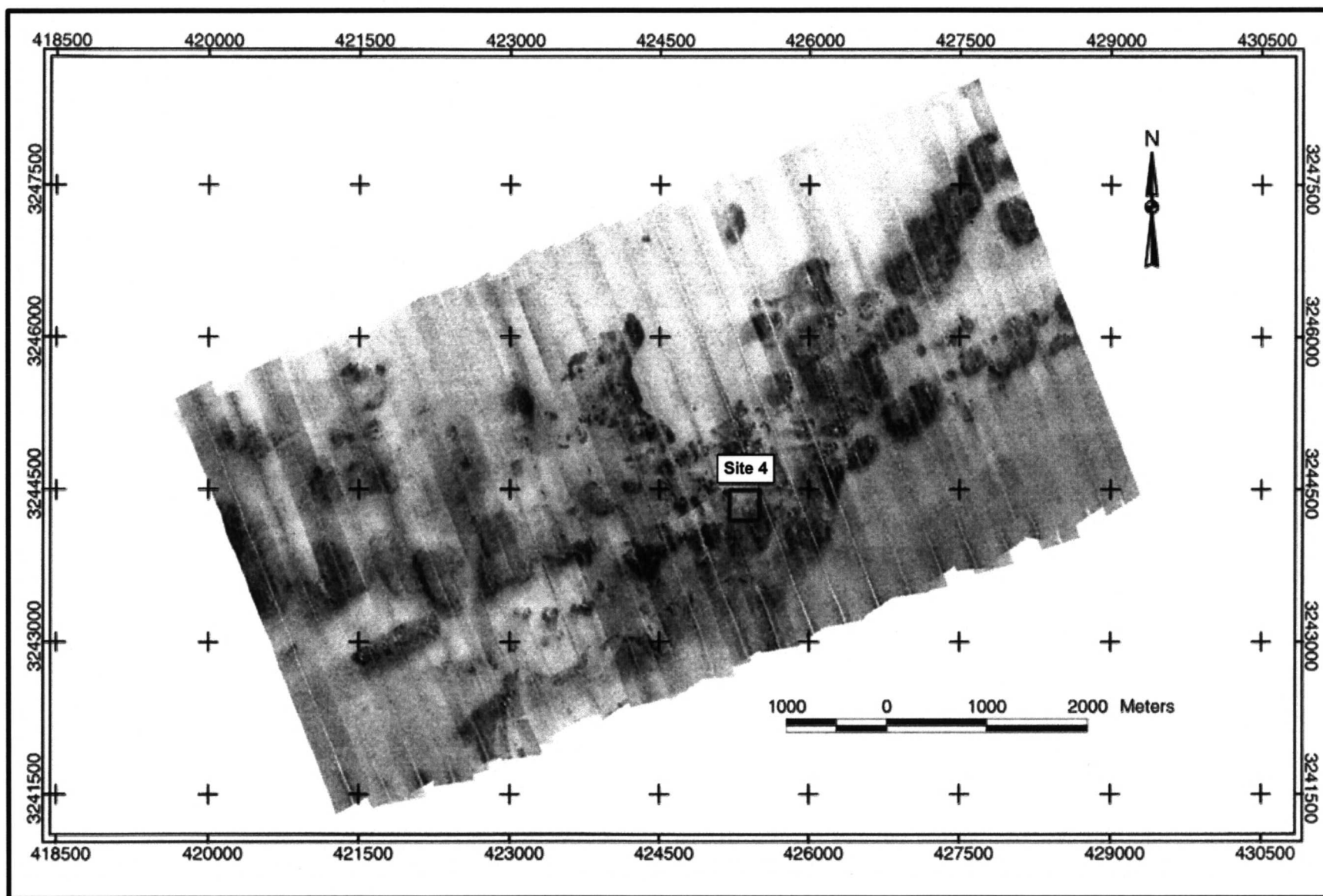
Fig. 4.12. TAMU 2 side-scan sonar mosaic of Megaseite 2, showing Monitoring Site 4 (small box). Conventions as in Fig. 4.10.
