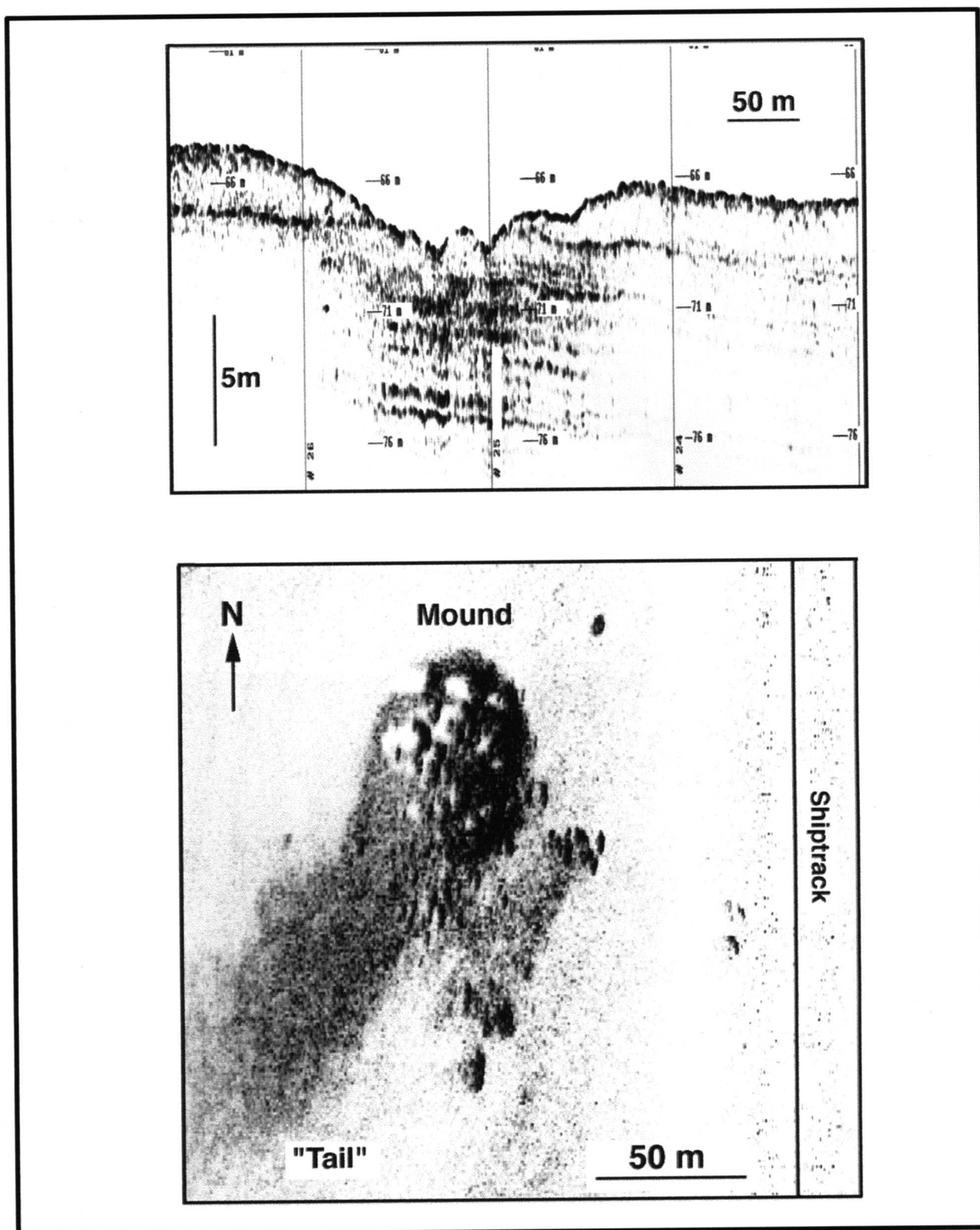
Fig. 4.11. Example of high-backscatter "tail" southwest of a mound in Megasite 1 and associated erosional gully. (Top) Chirp sonar subbottom profile showing gully approximately 3-m deep and 150 m across. (Bottom) High backscatter "tail" to southwest of mound. Dark areas indicate high backscatter and light represents low backscatter. Acoustic illumination is directed away from shiptrack (vertical line at right). Note: The two examples are from different locations because the subbottom profiler must pass directly over the tail feature, but the side-scan sonar does not image well directly beneath the sonar.
