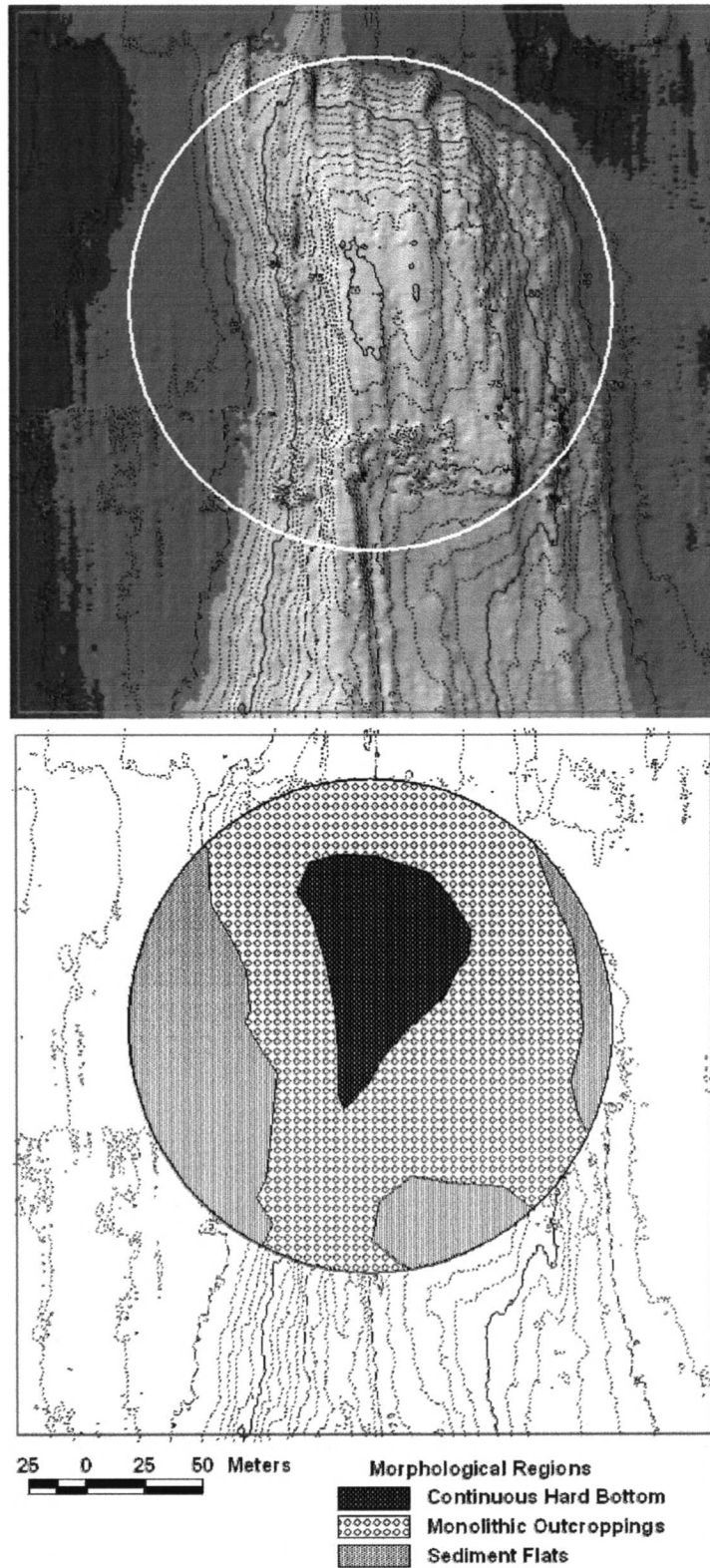
Fig. 4.24. Analysis of sea bottom morphology at Monitoring Site 7 derived from ROV photos and videos. (Top) Shaded relief bathymetry chart (compare to Fig. 4.9 for contour values). White circle denotes area investigated by ROV. (Bottom) Areas of similar seafloor morphology.
