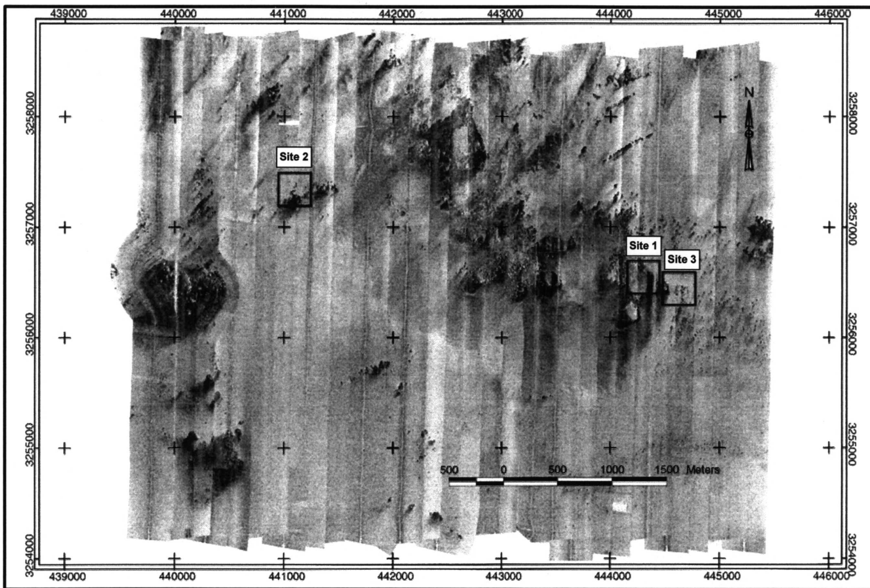
Fig. 4.10. TAMU 2 side-scan sonar mosaic of Megasite 1, showing Monitoring Sites 1-3 (small boxes). Vertical stripes are individual trackline side-scan sonar records pieced together to make the mosaic. Dark areas are high acoustic return (backscatter), whereas light areas are low backscatter. UTM plot with axes labeled in meters.
