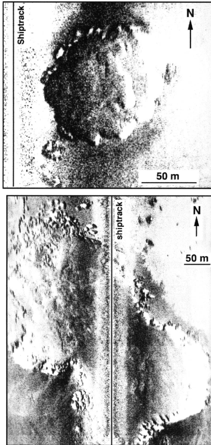
Fig. 4.19. Side-scan sonar images showing smooth-top mounds. (Top) Example from Megasite 3. Note the smooth top shows two levels. (Bottom) Large, flat-topped mound from Megasite 1. Monitoring Site 1 is located on the northeast edge of the top. Conventions as in Fig. 4.17.
