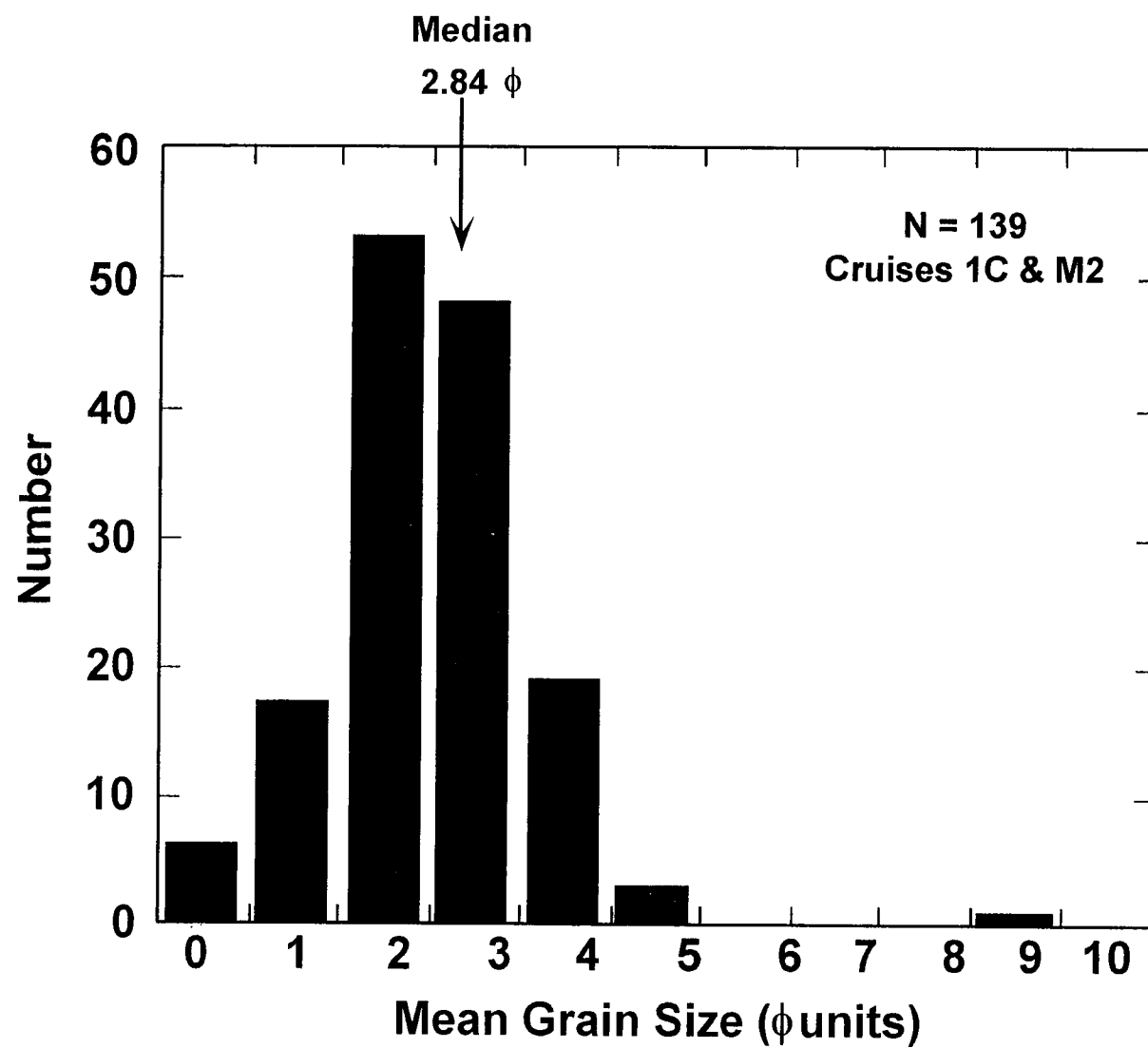
Fig. 4.25. Histogram of mean grain sizes for grab samples from Cruises 1C and M2.
