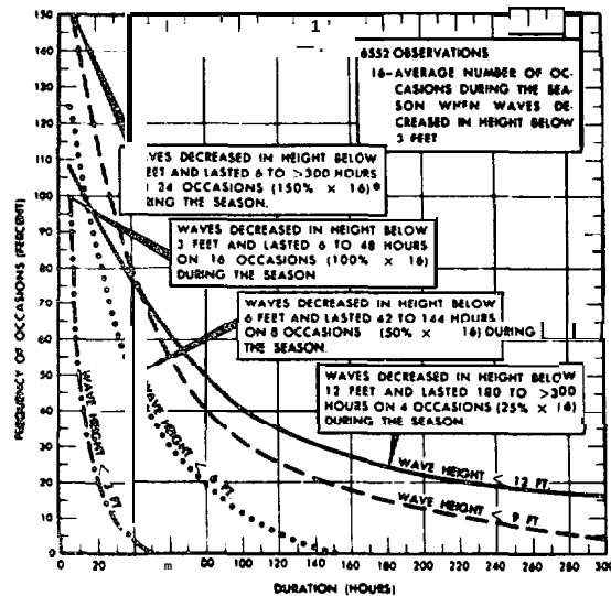
PERSISTENCE OF FAVORABLE SEAS (<3, 6, 9, 12 FT.)
