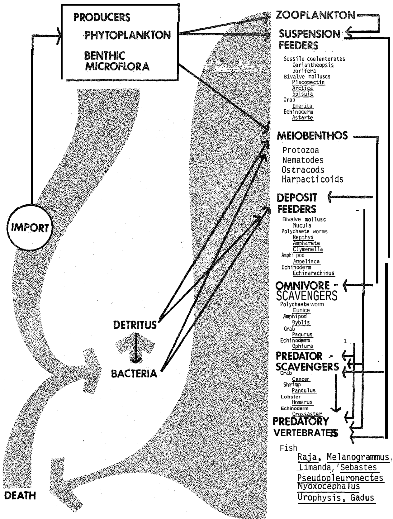
A SOCIO-ECONOMIC AND ENVIRONMENTAL INVENTORY OF THE NORTH ATLANTIC REGION TRIGOM PARC FIGURE Food Web of Offshore Bottom Habitat 3-200
