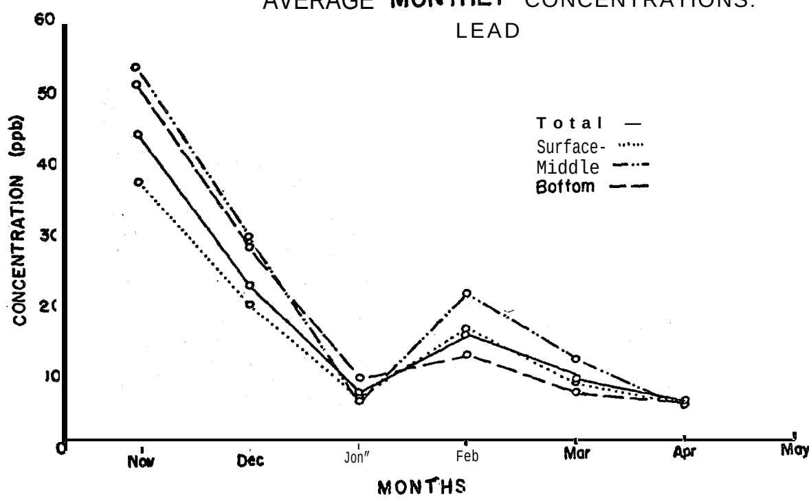
A SOCIO-ECONOMIC AND ENVIRONMENTAL INVENTORY OF THE NORTH ATLANTIC REGION TRIGOM PARC FIGURE 3-194b Average Monthly Concentrations -Dissolved Metals (Kostyla, 1973)
