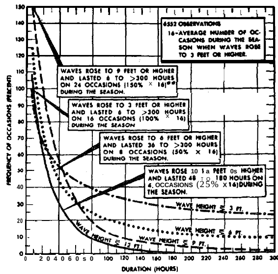
PERSISTENCE OF UNFAVORABLE SEAS (≥3, 6, 9, 12 FT.)
