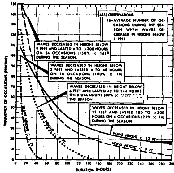
PERSISTENCE OF FAVORABLE SEAS (<3, 6, 9, 12 FT.)
