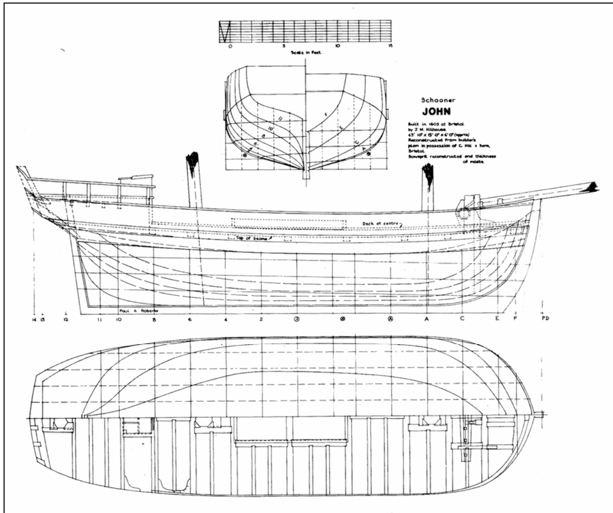
Figure 6.4. Lines and deck plan of John (source: MacGregor 1980:109).
