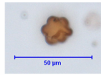
Gallium
