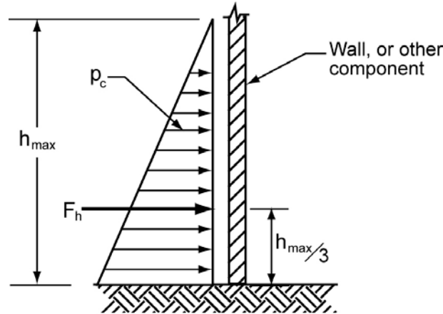
Figure 6-4 Hydrostatic force distribution and location of resultant.
