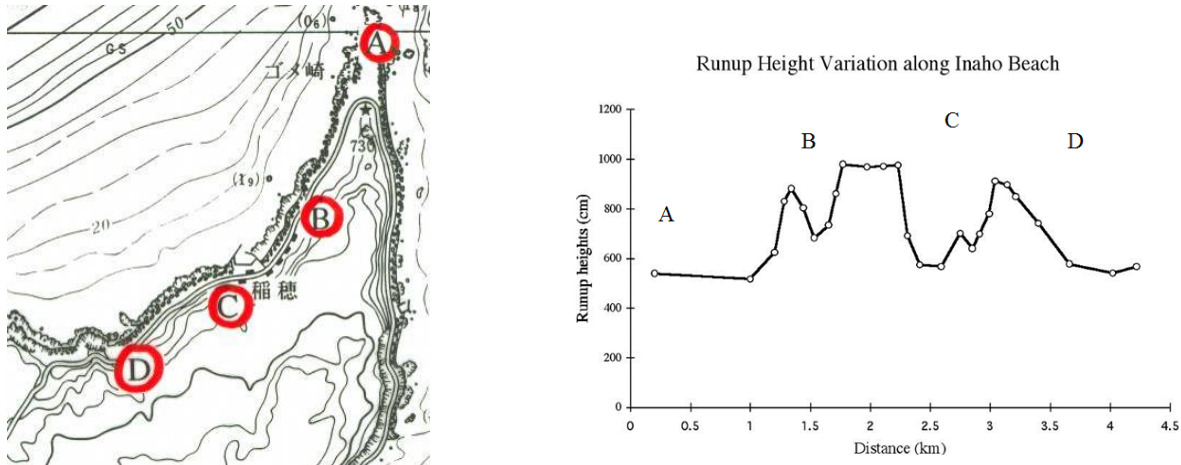
Figure 2-4 Measured runup heights of the 1993 Okushiri tsunami along Inaho Coast, demonstrating that runup height varies significantly between neighboring areas.
