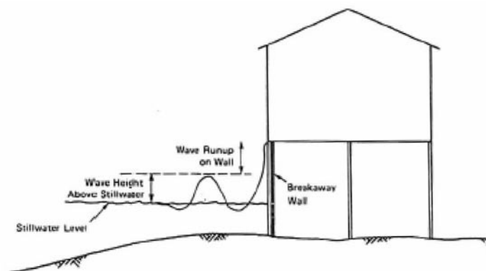
B. WAVE RUNUP ON BREAKAWAY WALL
