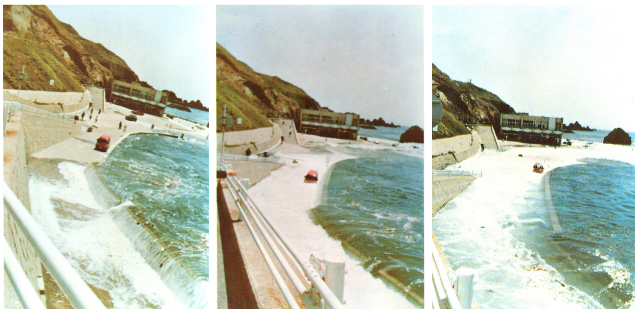
Figure 2-7 A sequence of photos of the 1983 Nihonkai-Chubu Tsunami showing surge flooding from tsunami runup (photo courtesy of S. Sato).
