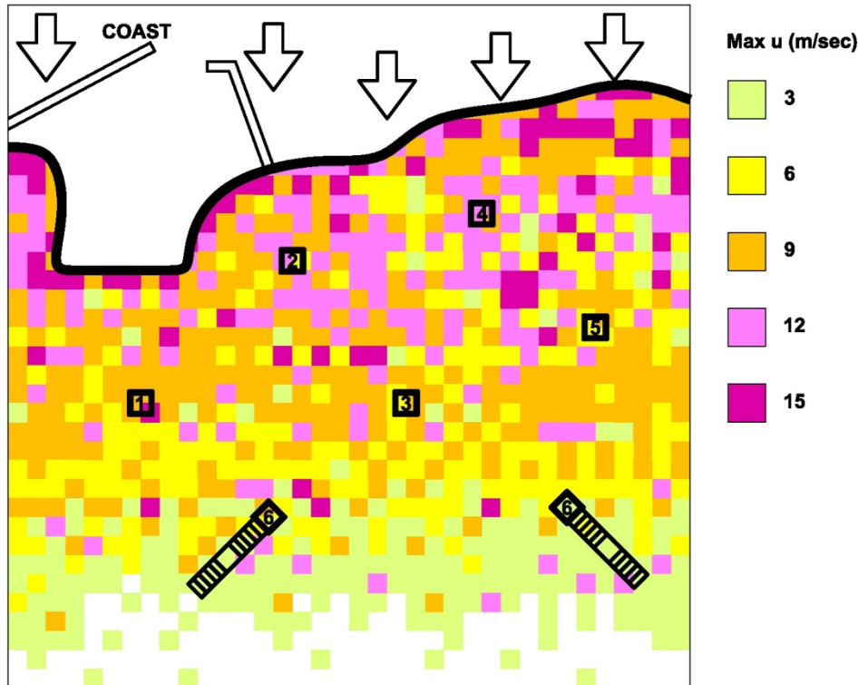
Figure B-3 Example community inundation flow velocity map. Shaded areas show various predicted tsunami flow velocities, u .
