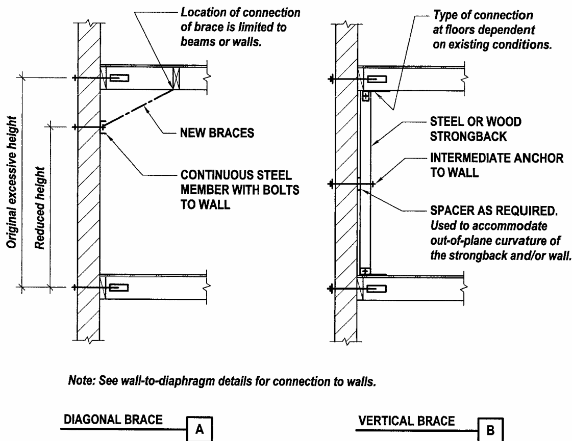
Figure 21.4.3-1: Exposed Out-of-Plane Wall Bracing
