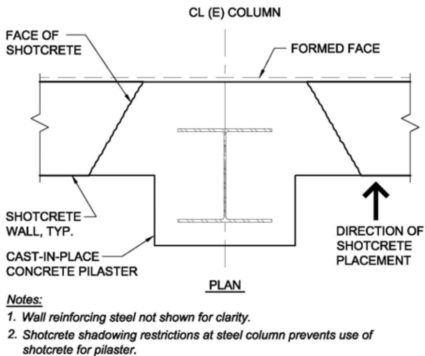
Figure 8.4.2-5: Combined Shotcrete and Cast-In-Place Construction
