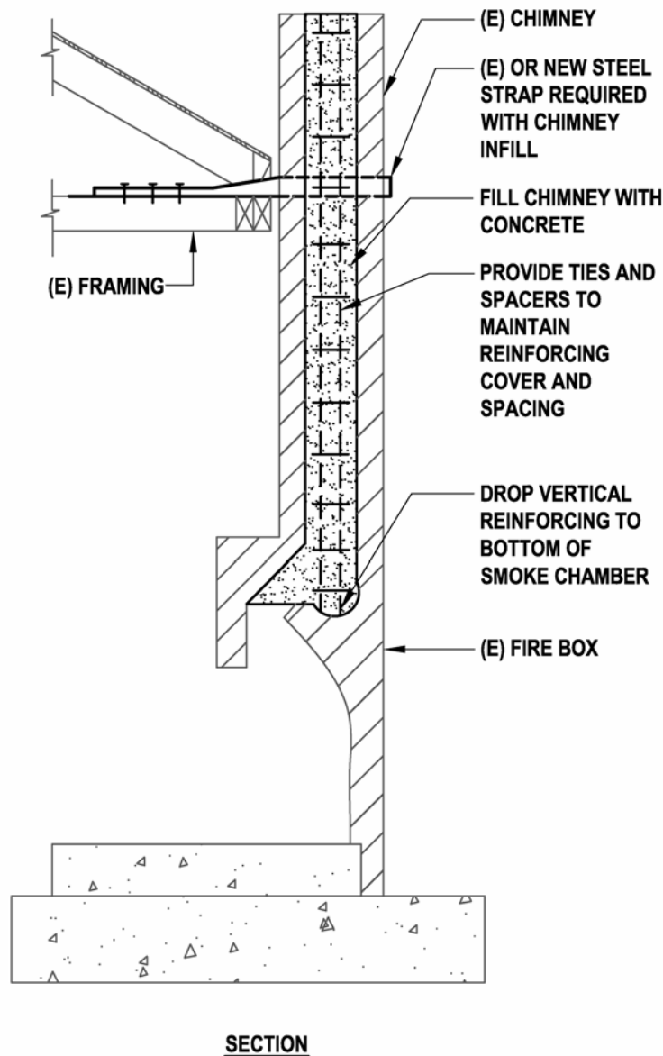
Figure 5.4.6-1: Infill and Bracing of Masonry Chimney
