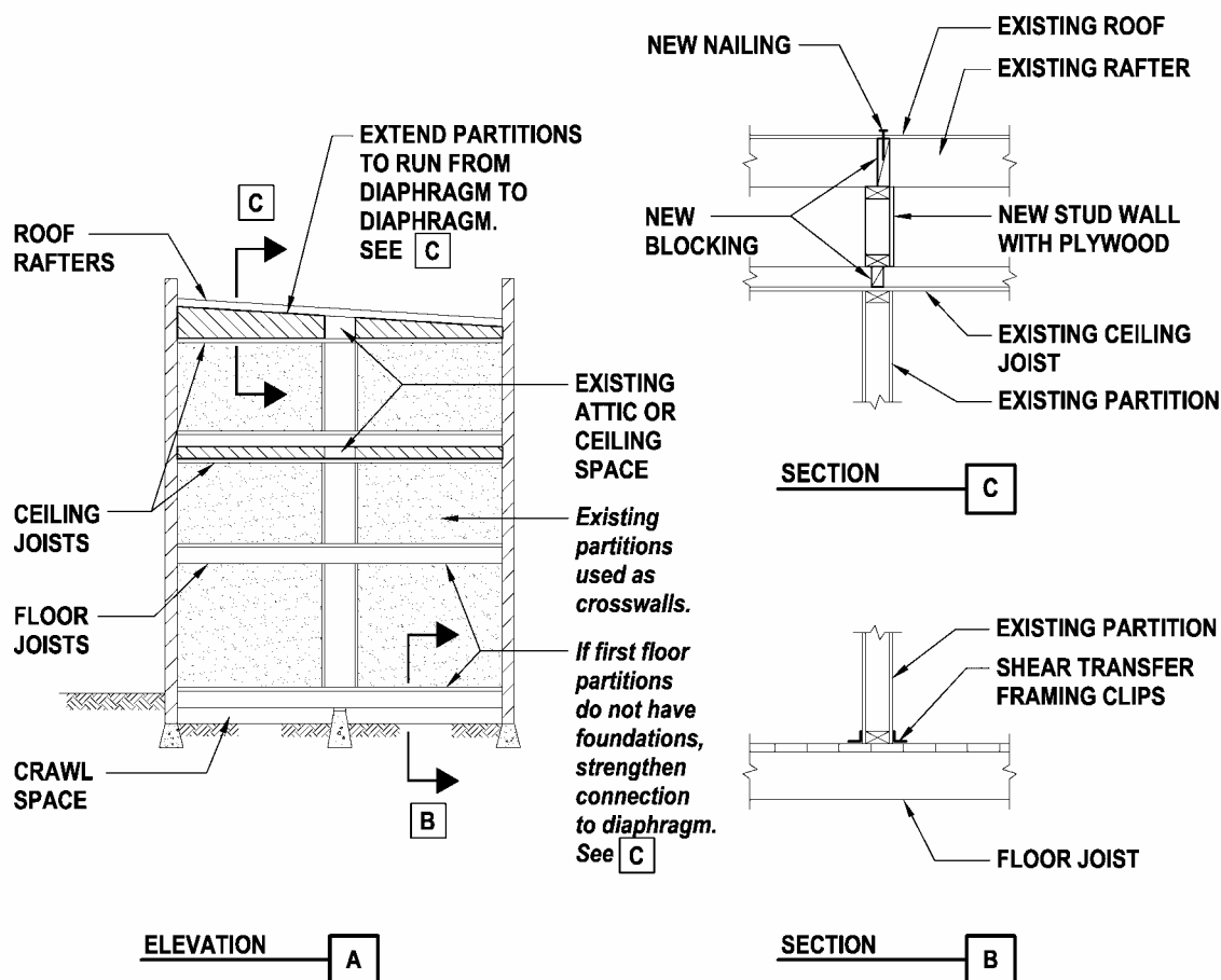
Figure 21.4.10-1: Strengthen Existing Crosswalls
