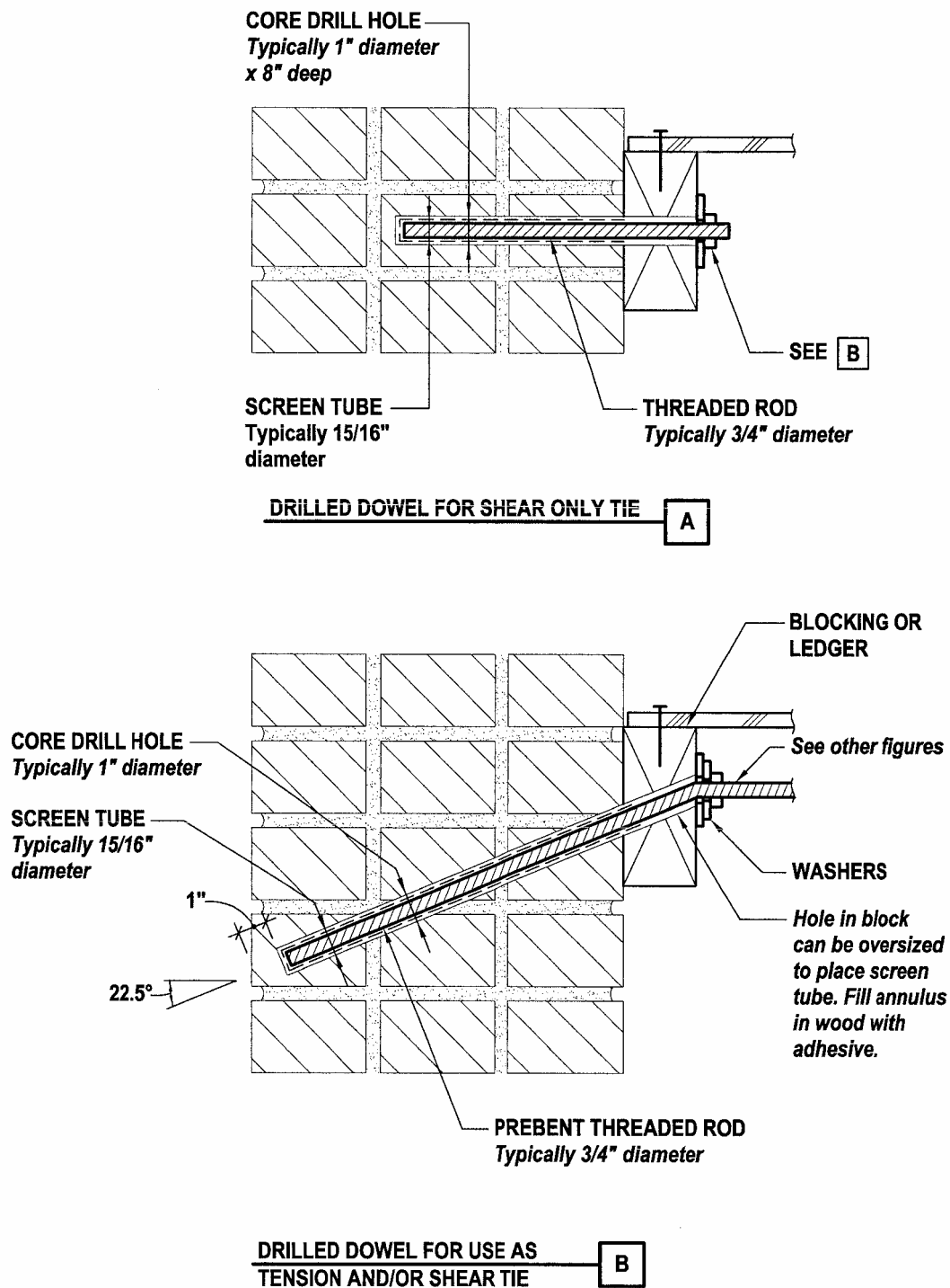
Figure 21.4.2-1: Drilled Dowels
