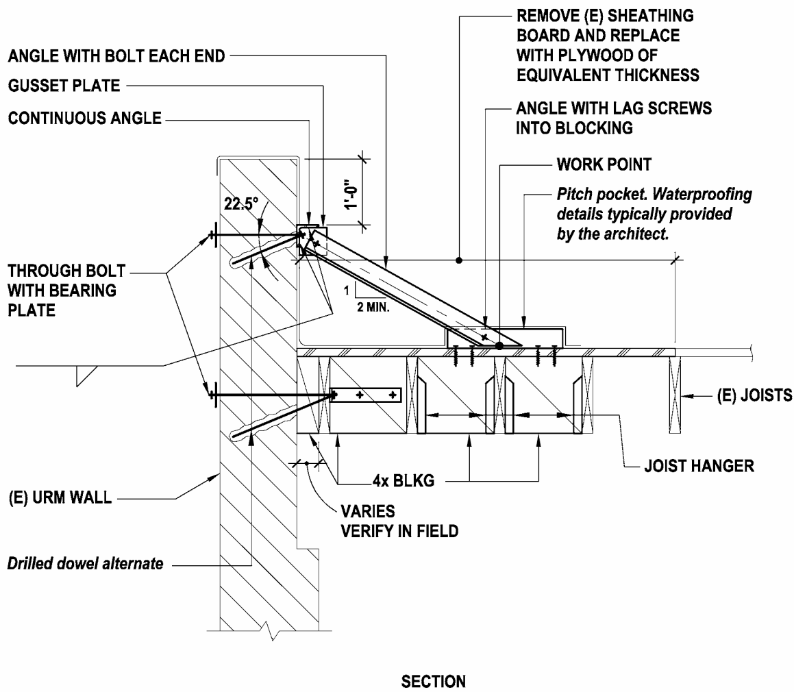
Figure 21.4.1-1: Parapet Bracing
