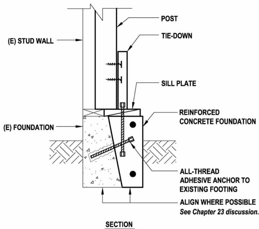
Figure 5.4.1-4: New Continuous Foundation Cast Along Side Existing to Provide Capacity for Tie-Down Anchor
