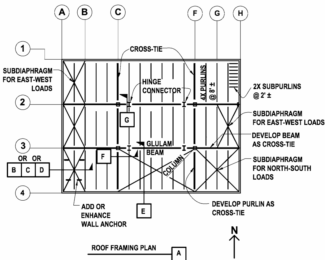
Figure 22.2.3-1A: Roof Plan with Diaphragm Cross-Tie System Using Subdiaphragms, Shown for Wood Diaphragm
