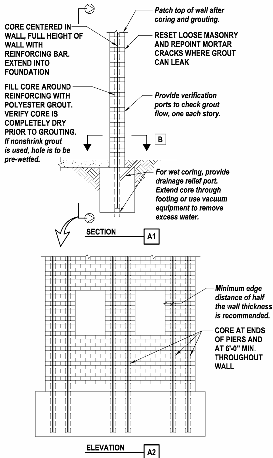
Figure 21.4.4-1A: Reinforced Cores
