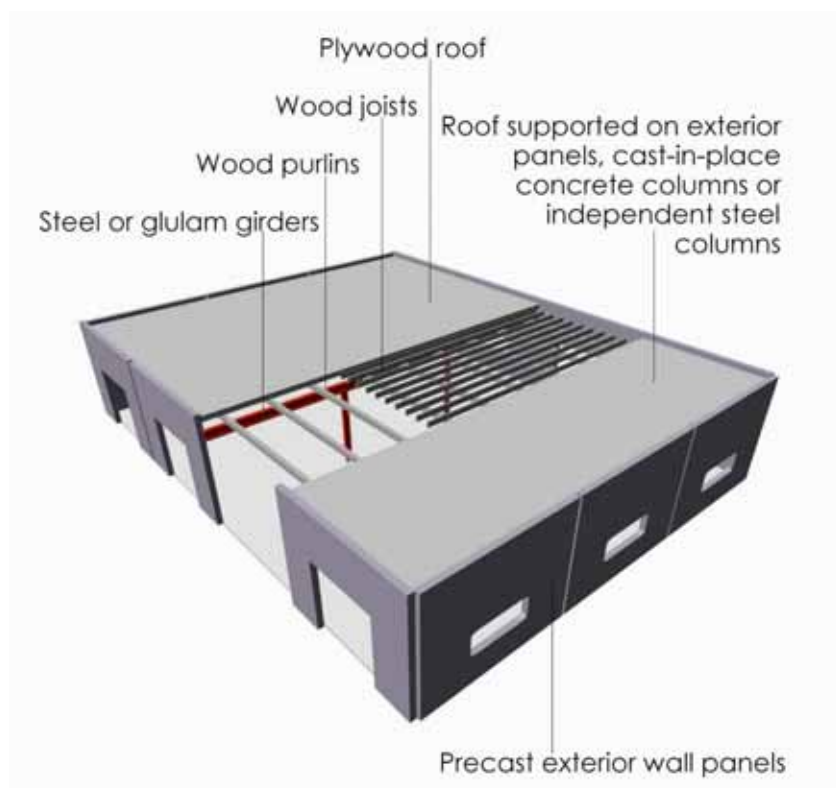
Figure 16.1-1: Building Type PC1: Tilt-Up Concrete Shear Walls
