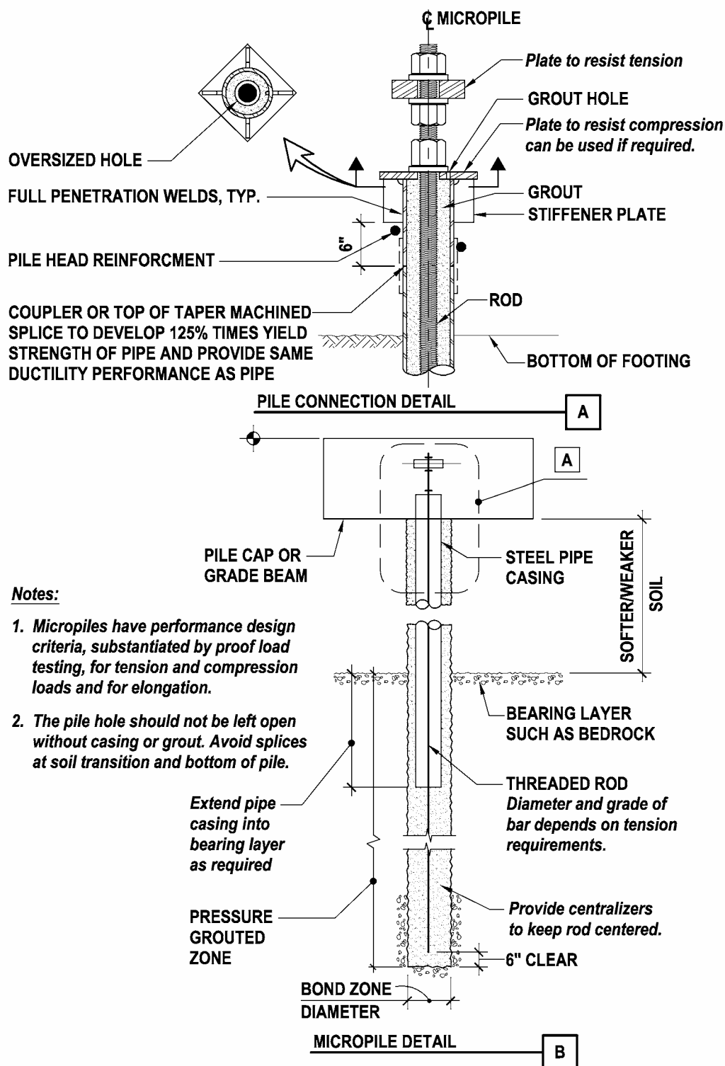
Figure 23.7.2-2: Micropile Details
