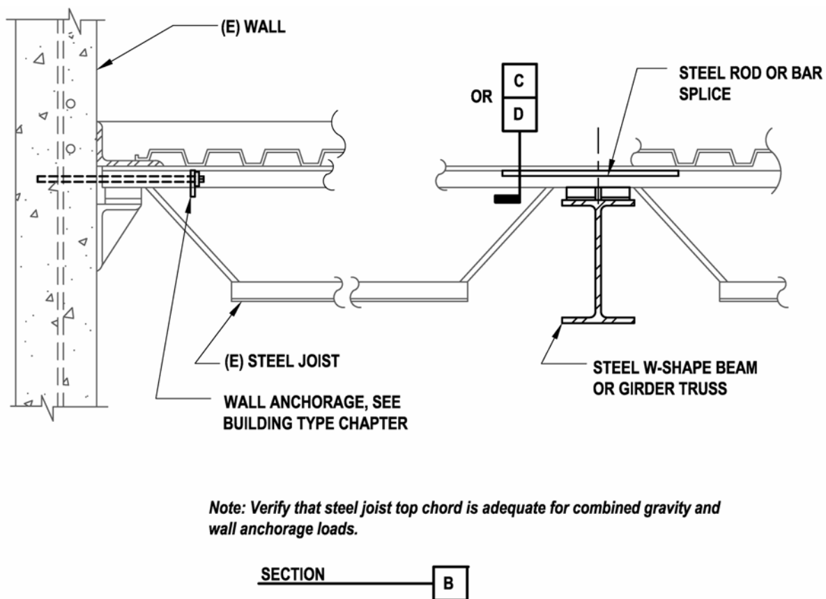
Figure 22.2.3-2B: Cross-Tie for Flexible Steel Diaphragm
