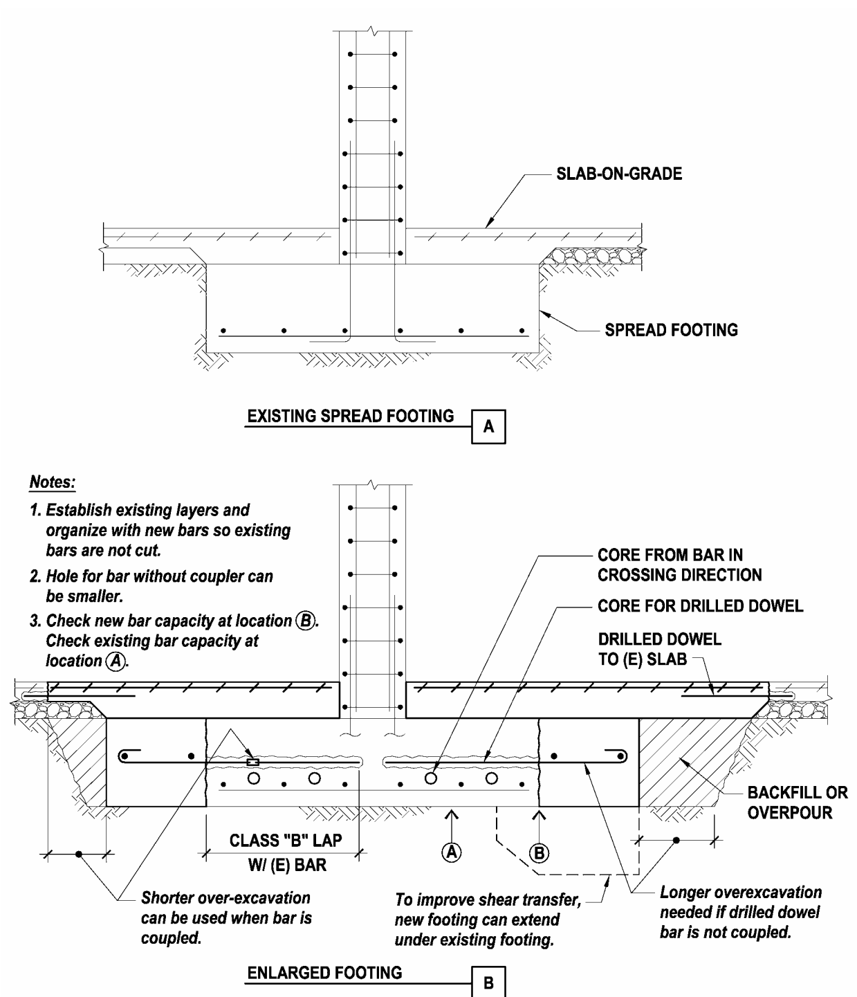
Figure 23.7.3-1: Enlarge Existing Spread Footing
