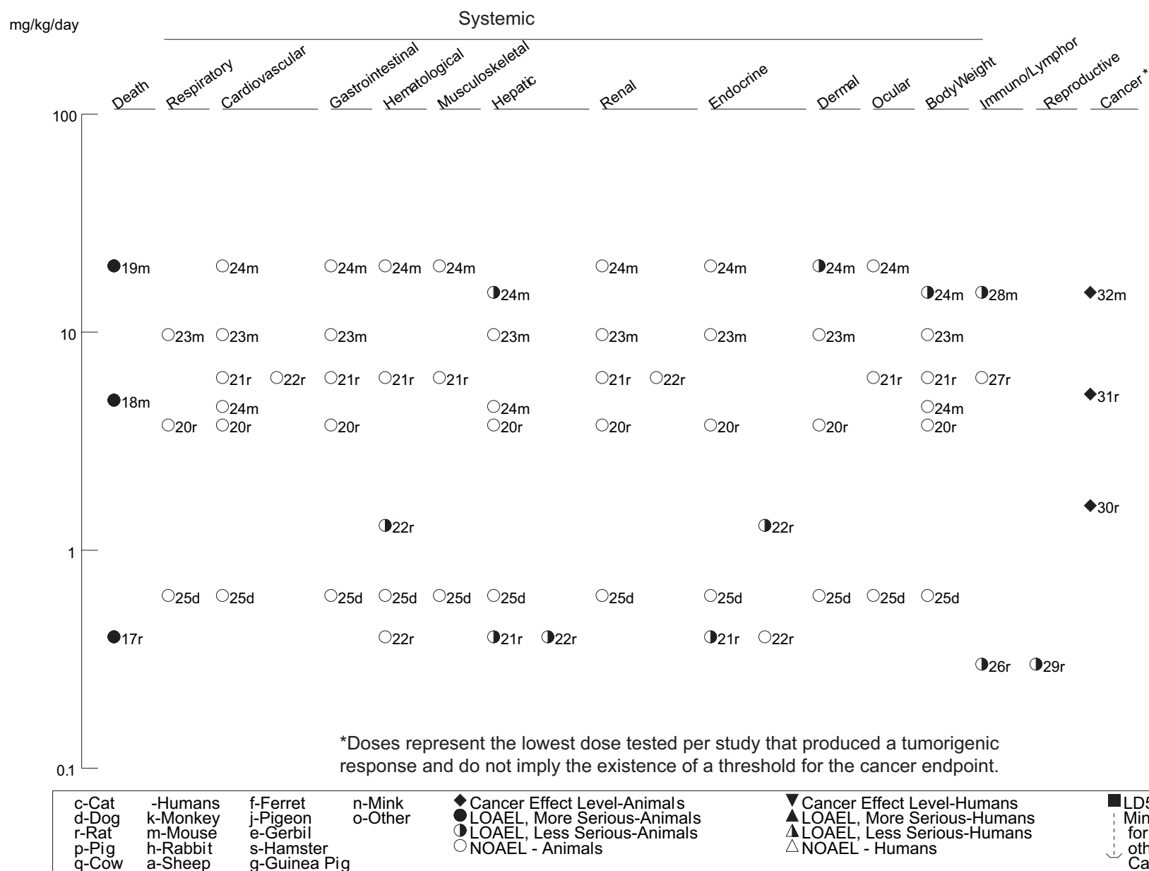
Figure 3-5 Levels of Significant Exposure to Triphenyltins - Oral ( Continued ) Chronic ( \geq 365 days)
