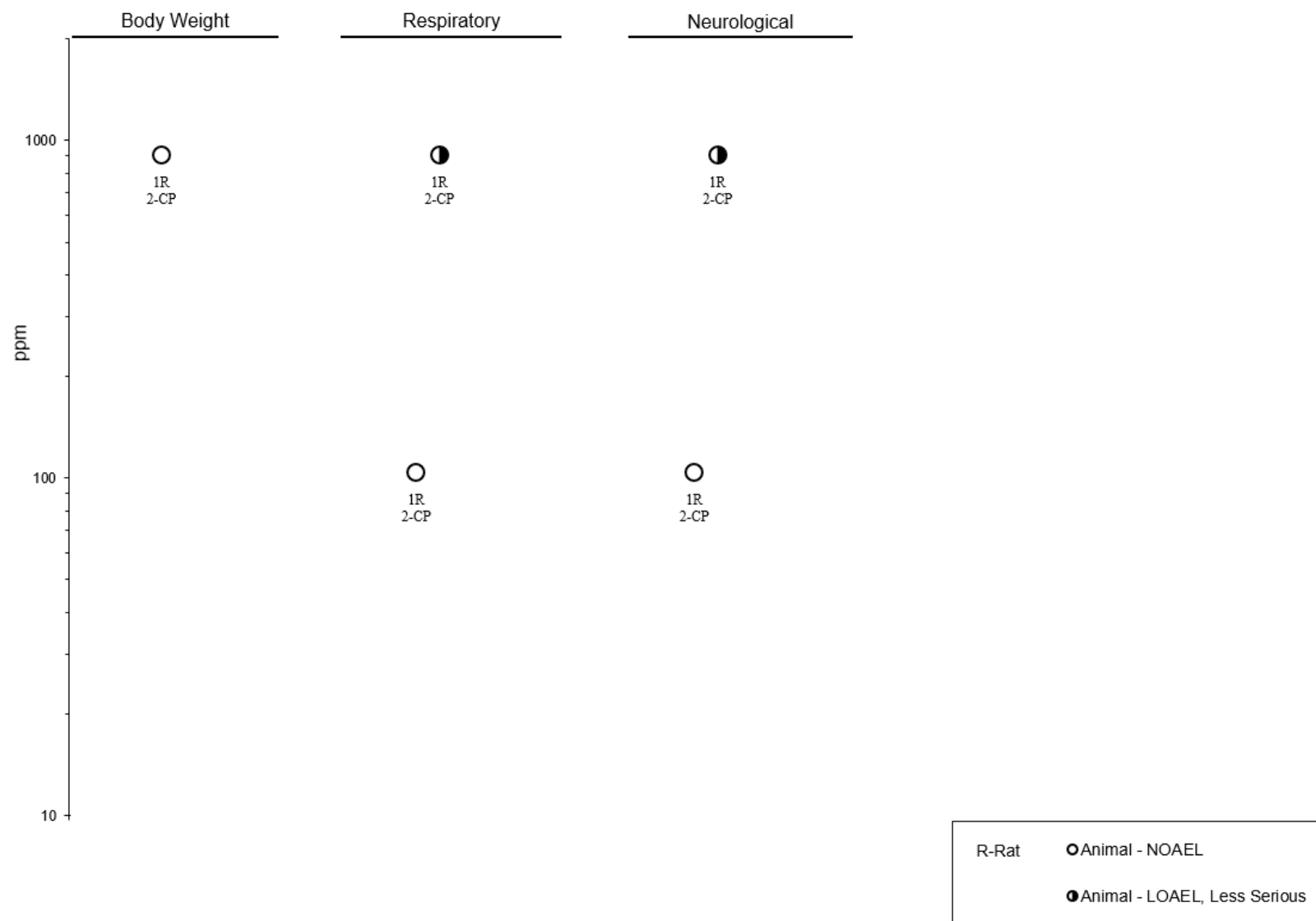
Figure 2-8. Levels of Significant Exposure to Chlorophenols – Inhalation
