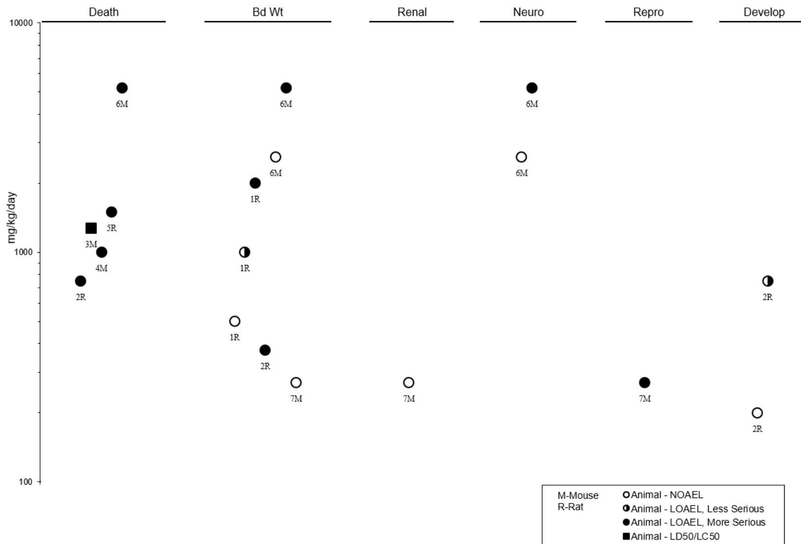
Figure 2-11. Levels of Significant Exposure to 2,4-Dichlorophenol – Oral Acute ( \leq 14 days)
